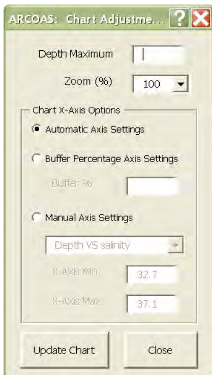
Figure 4.22: Profile Plotting - Chart Adjustments dialogue box.
