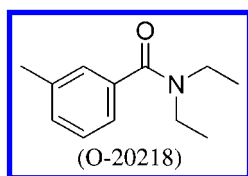
Figure 1. Orlando number and structure of N,N-diethyl-3-methylbenzamide (DEET).
