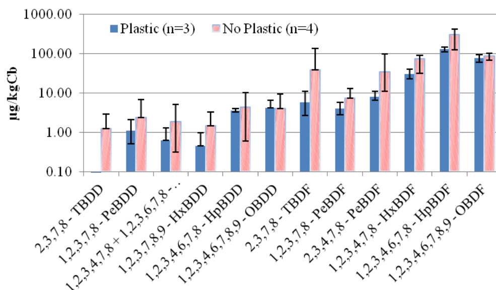
Figure 5: Average PBDD/F Congener Comparison Graph Error Bars represent min and max values
