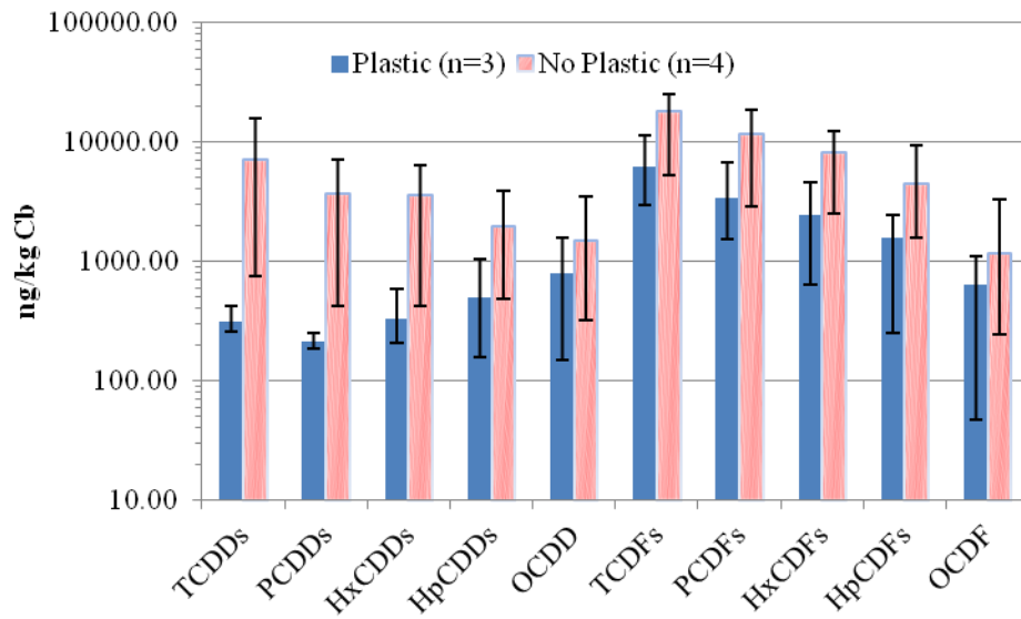
Figure 4: Average PCDD/F Homolog Comparison Graph
