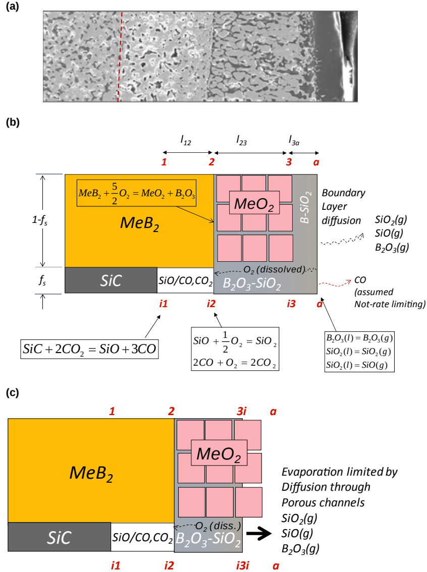
Fig. 1. (a) SEM image of the microstructure of oxidation scale formed on a \text{ZrB}_2 -SiC sample (Courtesy: E Opila, Univ. Virginia) (b, c) Schematic sketches of the oxidation products and morphology assumed in the model. At lower temperatures (b) external glassy scale forms, whereas at higher temperatures or high ambient flow (c), the glassy scale recedes inward due to evaporative loss of \text{SiO}_2 and \text{B}_2\text{O}_3 .
