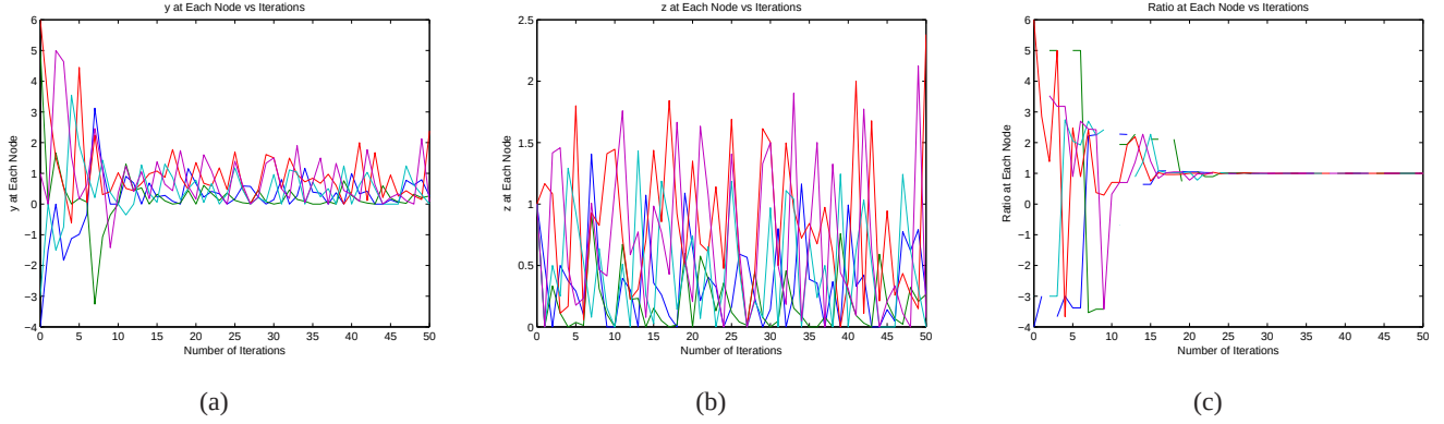
Fig. 3. Evolution of the values of y_j[k] (left), z_j[k] (middle), and \frac{y_j[k]}{z_j[k]} (right) for q = 0.5 , j = 1, 2, 3, 4, 5 .
