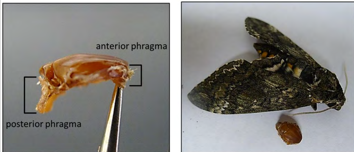
Figure 70 - M.sexta tergum side view and comparison with intact specimen. The phragma are extensions of the cuticle which support the dorsolongitudinal muscles. Despite how it may appear, the tergum is essentially all one continuous piece.
