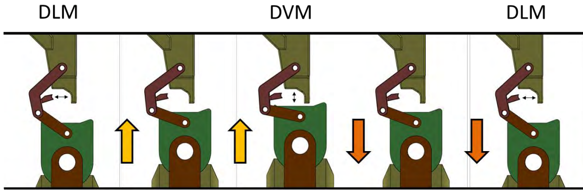
Figure 100 - Sequential representation of one full cycle. From left to right: Shaker is at lowest displacement and DLM compression is complete; shaker travels upward; shaker is at maximum displacement with full DVM compression; shaker travels downward; longitudinal compression begins again.
