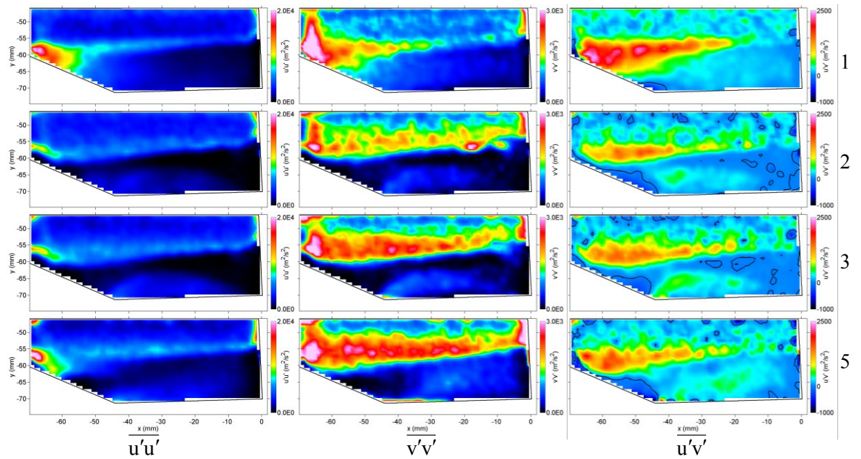
Figure 12: Time-averaged values of \overline{u'u'} , \overline{v'v'} , and \overline{u'v'} .
