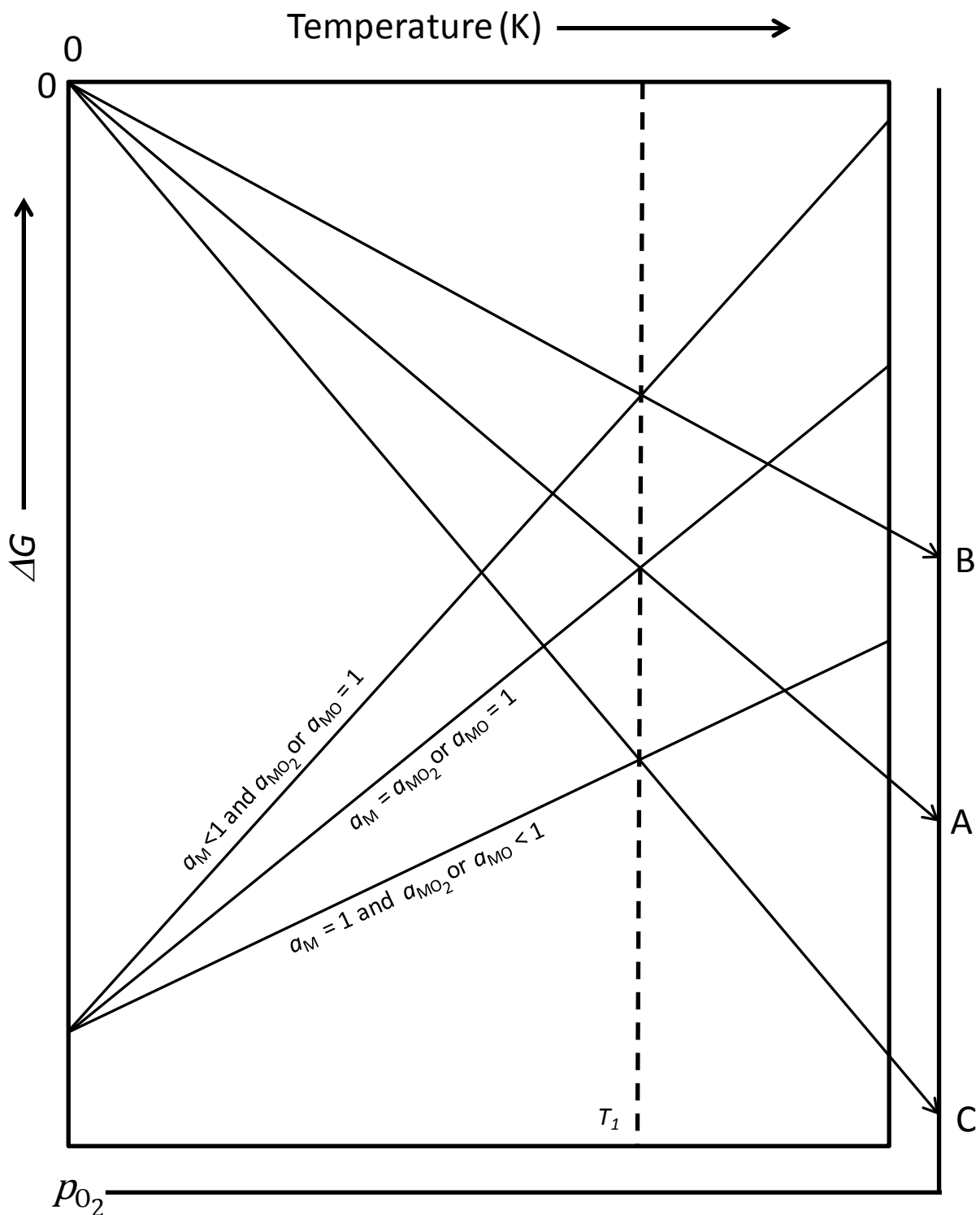
Fig. 2: Variation in \Delta G vs. T line for non-unit activities of metal (M) and its oxide ( \text{MO}_2 or \text{MO} ). For the case of Ti-oxidation, oxide is of type \text{MO}_2 and for Ni-oxidation, oxide is of type \text{MO} . At a fixed temperature T_1 , the equilibrium p_{\text{O}_2} for oxidation reaction is denoted on the nomographic scale by point “A” for the case of a_{\text{M}} = a_{\text{MO}_2} or a_{\text{MO}} = 1 , by point “B” for the case of a_{\text{M}} < 1 and a_{\text{MO}_2} or a_{\text{MO}} = 1 , and by point “C” for the case of a_{\text{M}} = 1 and a_{\text{MO}_2} or a_{\text{MO}} < 1 . Here, a_{\text{M}} and ( a_{\text{MO}_2} or a_{\text{MO}} ) stand for activities of metal and its oxide, respectively. After ref. [25].
