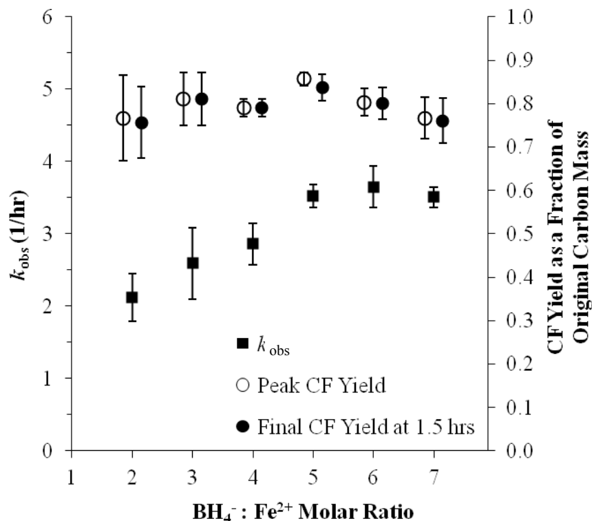
Figure 3.1. Degradation of CT by nZVI synthesized at varying \text{BH}_4^- : \text{Fe}^{2+} molar ratios. k_{obs} is the observed pseudo-first order rate constant. [\text{nZVI}] = 0.01 \text{ g/L} , [\text{C0}] = 0.25 \text{ mg/L} , [\text{CMC}] = 2 \text{ g/L} , \text{pH} = 7 , and the sampling period lasted 1.50 hrs.
