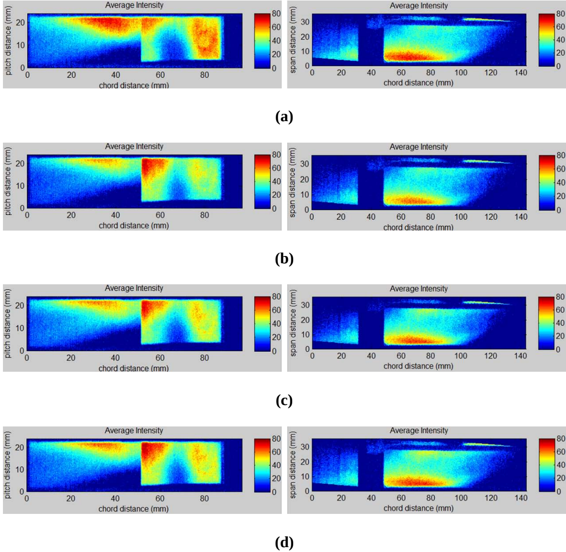
Figure 5.1: Side view (left) and top view (right) HSV results for (a) 66 % of fuel in the seeder box and both injectors on (b) Injector 1 off, (c) Injector 2 off, and (d) UCC section injectors at half their blowing ratios, MFR = 0.2 , \Phi = 2.2
