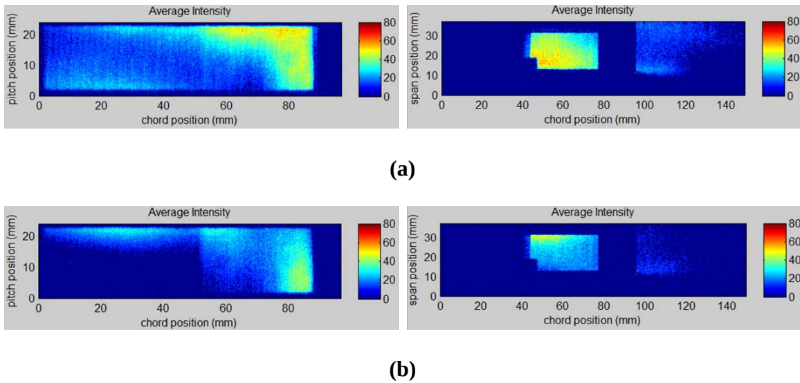
Figure 5.6: Side view (left) and bottom view (right) showing the effect of changes in MFR to the RVC on the top of the core section for (a) MFR = 0.3 and (b) MFR = 0.1
