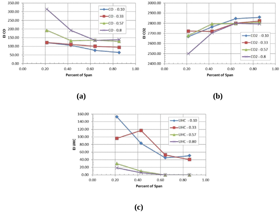
Figure 5.15: Emission Index for tiger claw at MFR = 0.1, g-loading = 1000 g's, and \Phi = 2.2 for (a) CO, (b) CO 2 , and (c) UHC
