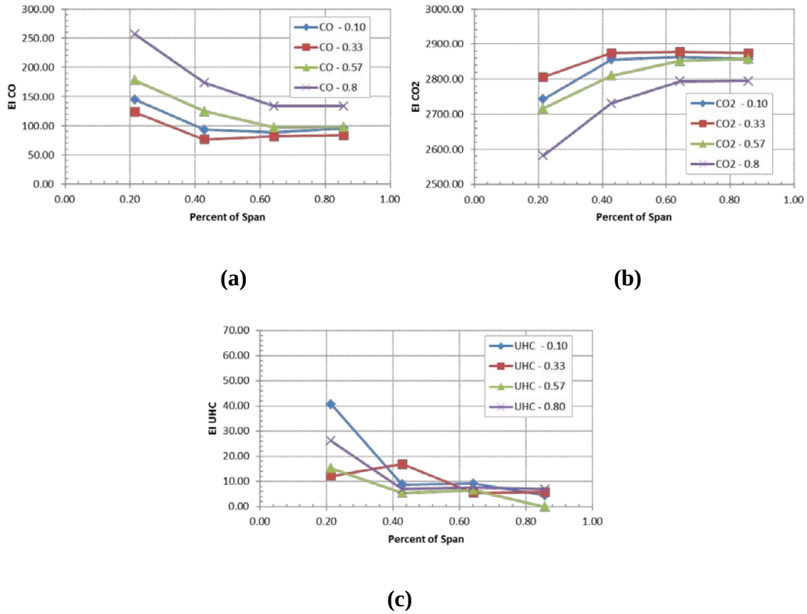
Figure 5.14: Emission Index for tiger claw at MFR = 0.3, g-loading = 1000 g's, and \Phi = 2.2 for (a) CO, (b) CO 2 , and (c) UHC
