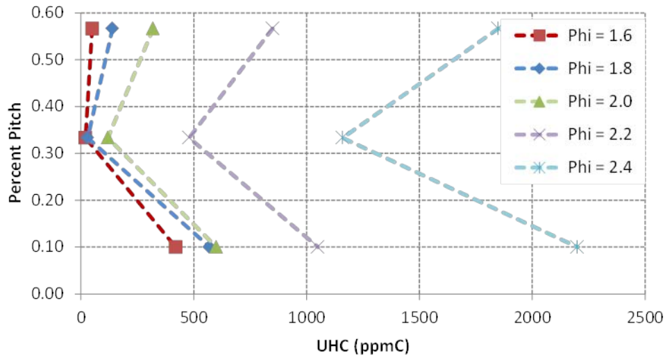
Figure 4.3: UHC concentration as a function of equivalence ratio at 21 % span
