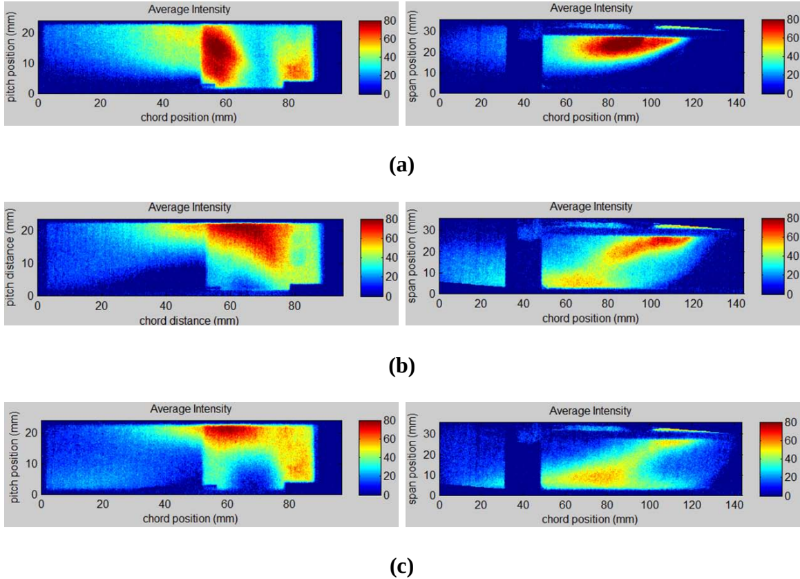
Figure 5.4: Side view (left) and top view (right) showing the effect on the flame shape and intensity due to changing MFR for (a) MFR = 0.1 , (b) MFR = 0.2, and (c) MFR = 0.3
