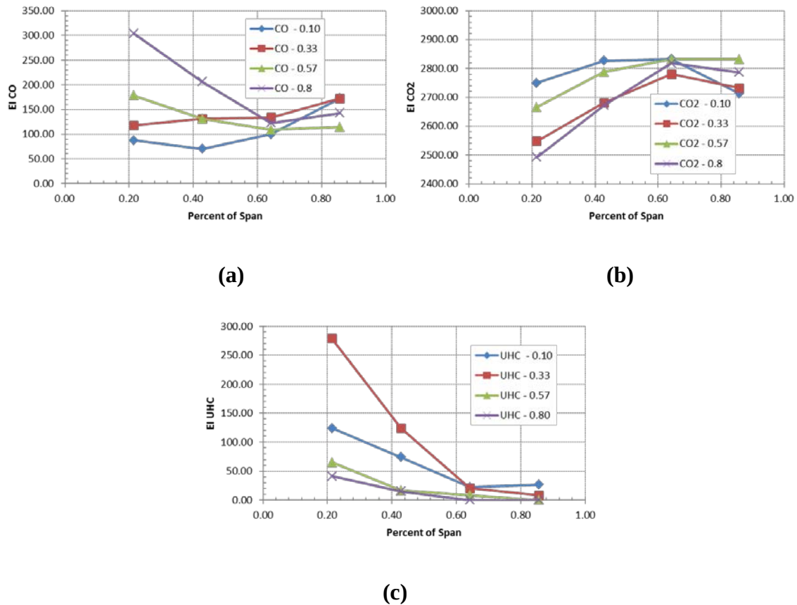
Figure 5.16: Emission Index for tiger claw at MFR = 0.2, g-loading = 500 g's, and \Phi = 2.2 for (a) CO, (b) CO 2 , and (c) UHC
