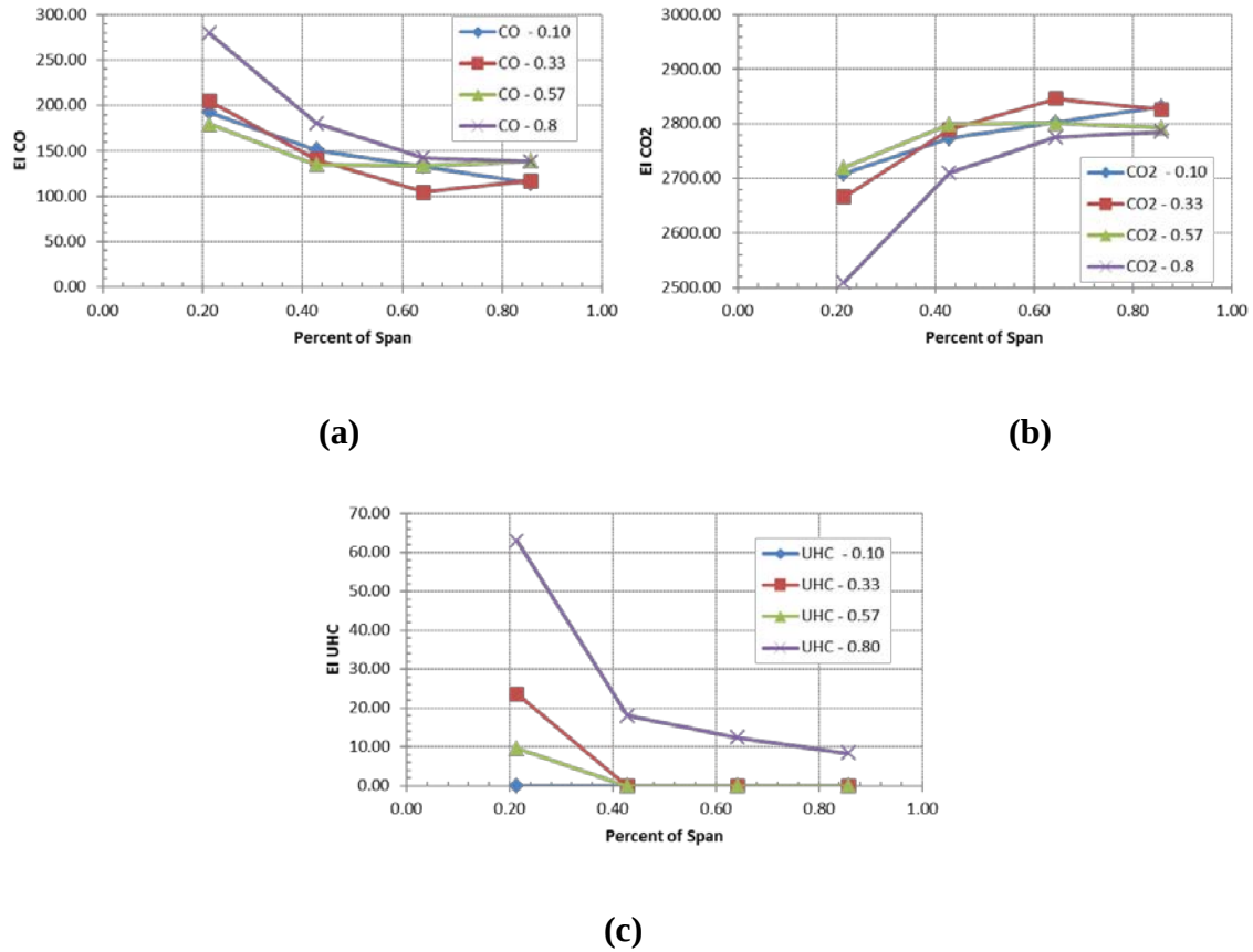
Figure 5.11: Emission Index for (a) CO, (b) CO 2 , and (c) UHC for the RVC vane located on the top of the core section for MFR = 0.2, g-loading = 1000 g, and \Phi = 2.2
