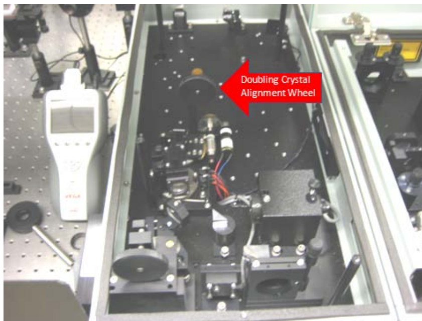
Figure A.20: Inside the dye laser, highlighted is the Doubling Crystal Alignment Wheel, used to focus the UV beam
