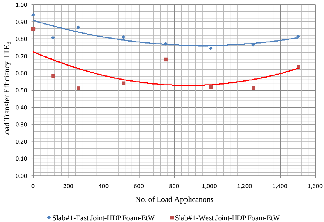
Figure C-1. Load Transfer Efficiency (LTE δ ) for Slab #1
