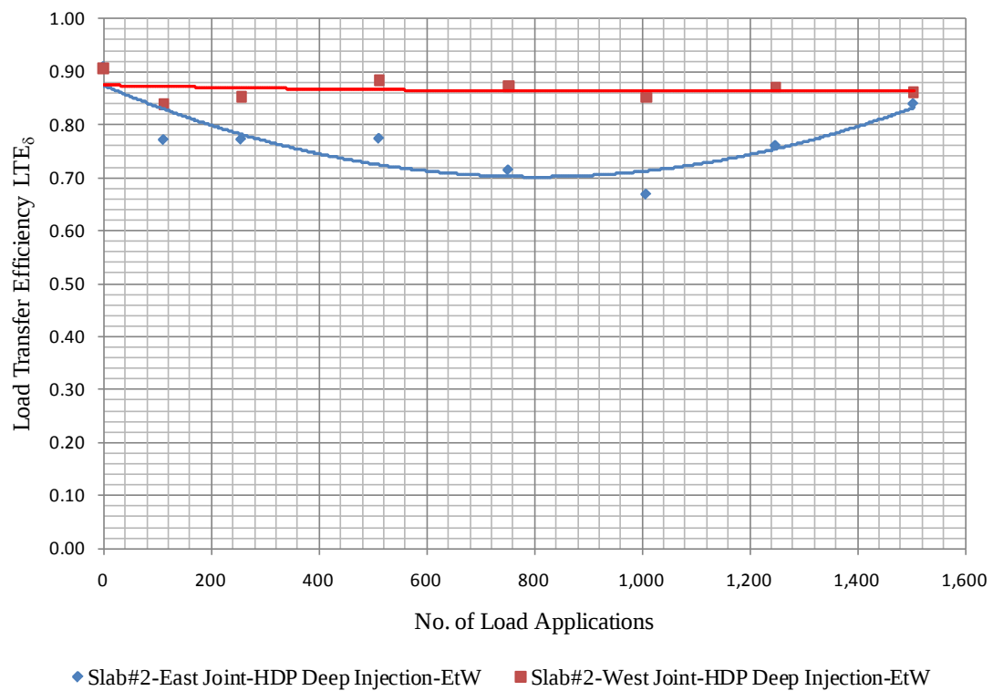
Figure C-2. Load Transfer Efficiency (LTE δ ) for Slab #2
