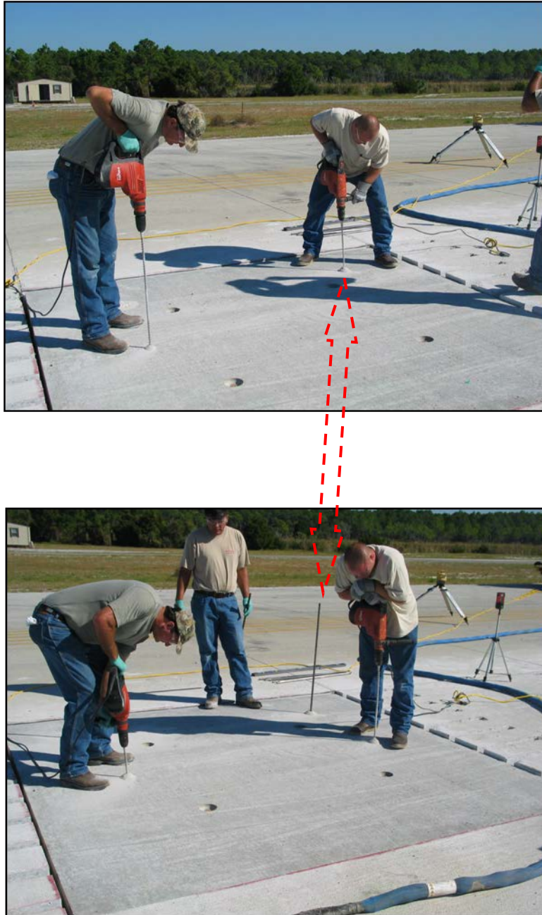
Figure 25. Installation of Hollow Injection Rods for Uretek Deep Injection
