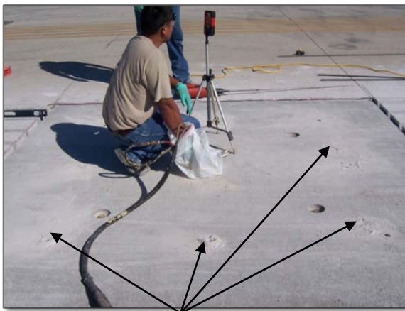
Injection ports
