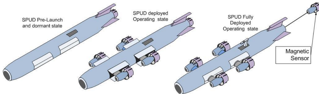
Figure 41. SPUDS Vehicle: Alternative One
