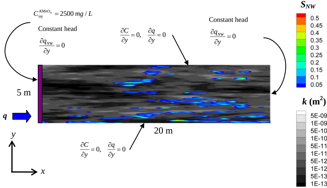
Figure 2. Cross-section of model domain with boundary and initial conditions. Section located at z = 5 m for TCE base case.
