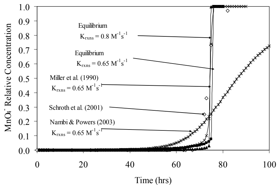
Figure 4 - Comparison of experimental \text{MnO}_4^- effluent concentrations (Schroth et. al, 2001) with model results for two TCE- \text{KMnO}_4 reaction rate constants.
