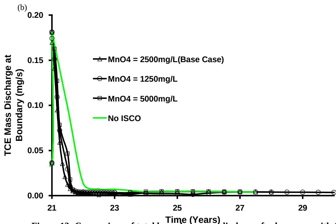
Figure 13: Comparison of total boundary mass discharge for base case with (a) various \text{MnO}_4 concentration injected and (b) since the start of the Treatment stage only (timescale expanded for clarity).
