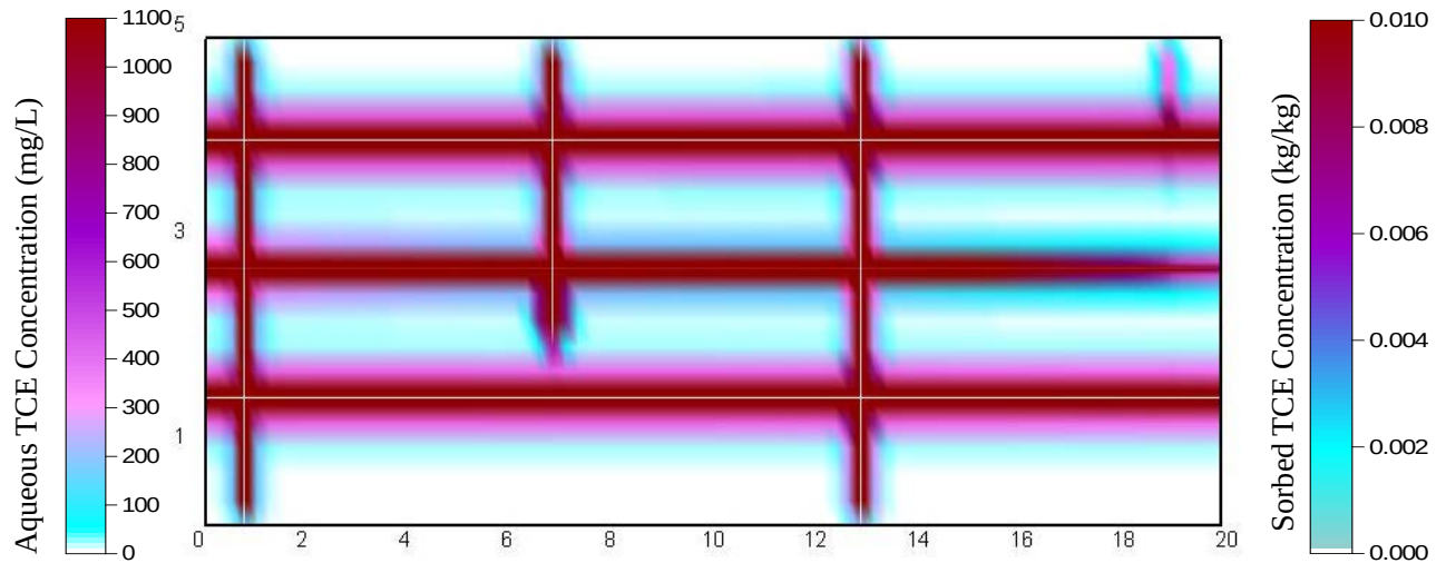
Figure 9: Distribution of aqueous and sorbed TCE after 20 years ( t_{\text{TOTAL}} = 21 years) of DNAPL dissolution.
