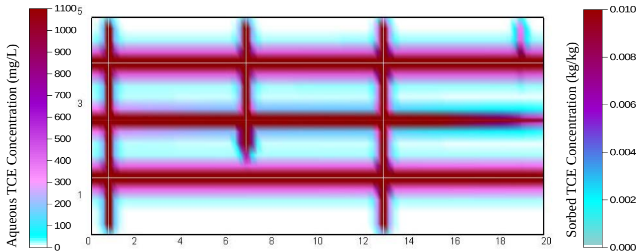
Figure 4: Distribution of aqueous and sorbed TCE after 20 years ( t_{\text{TOTAL}} = 21 years) of DNAPL dissolution (i.e., Site Ageing stage).
