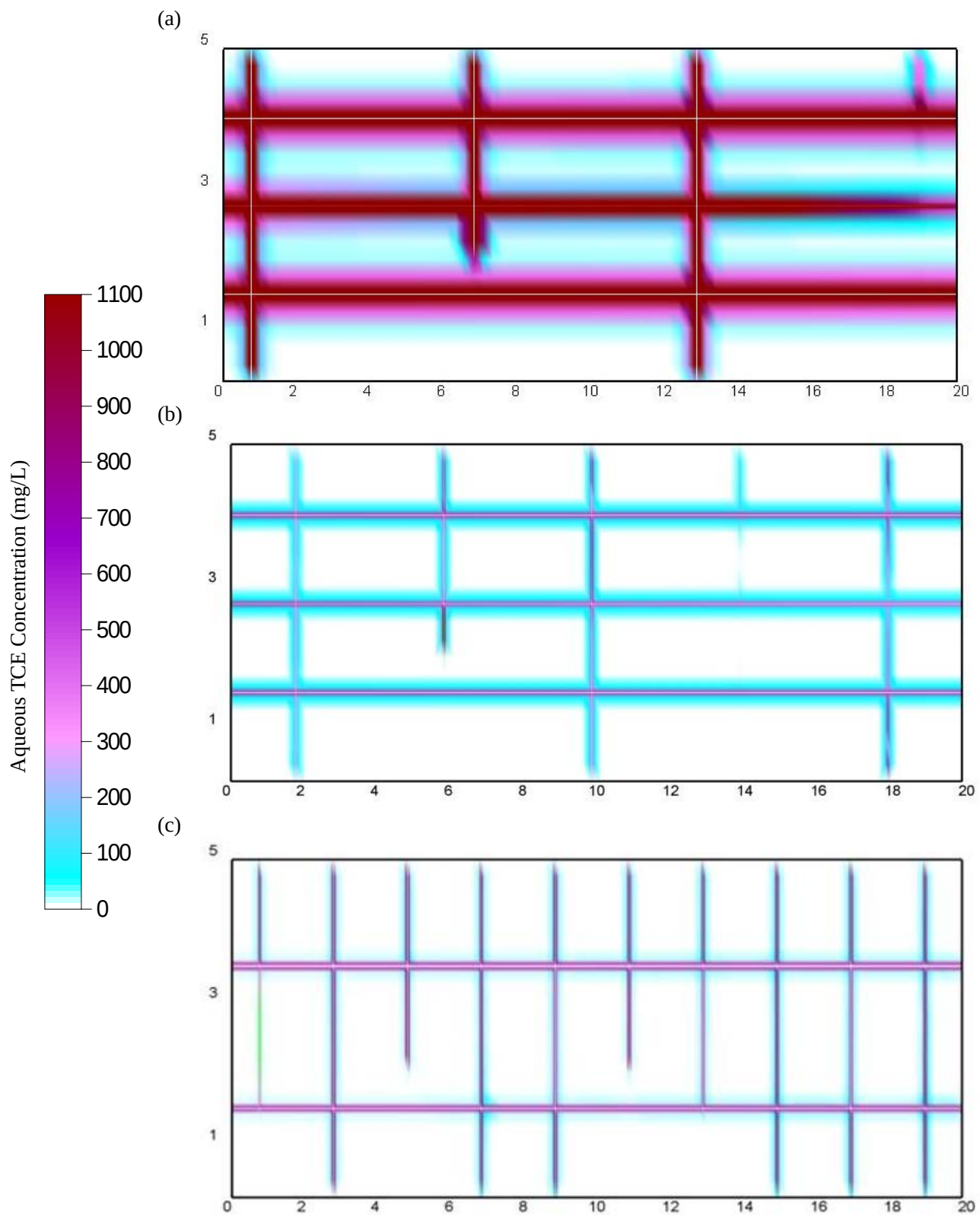
Figure 27: Distribution of aqueous TCE after 20 years ( t_{\text{TOTAL}} = 21 years) of DNAPL dissolution in (a) Sandstone, (b) Shale and (c) Granite.
