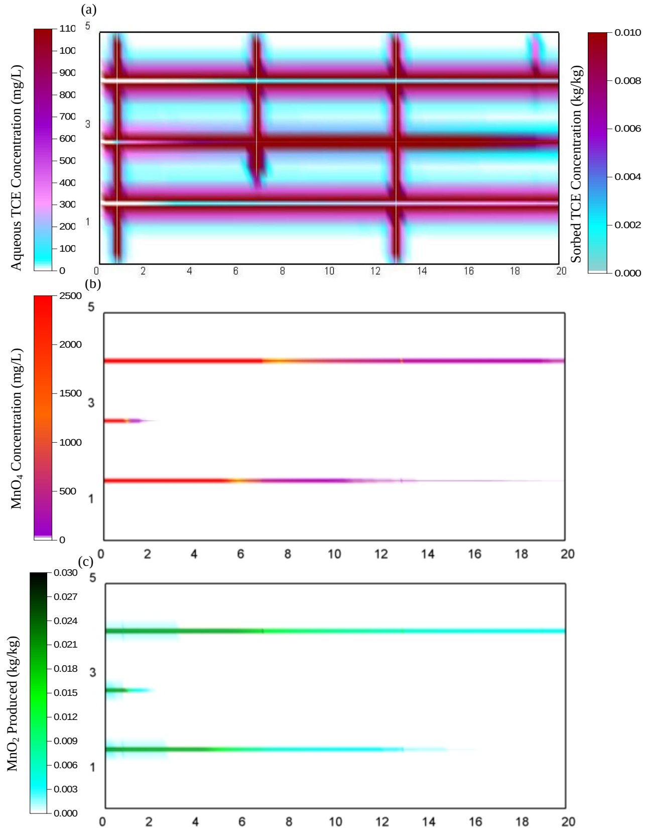
Figure 5: Distribution of aqueous species concentrations at t_{\text{TOTAL}} = 23 years for Base Case after 2 years of chemical oxidation (i.e., Treatment stage): (a) TCE, (b) \text{MnO}_4^- , (c) \text{MnO}_2 .
