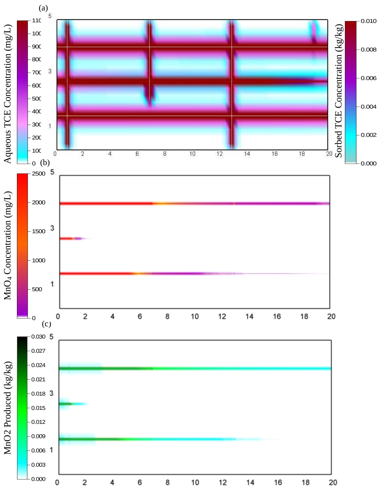
Figure A5: Distribution of aqueous species concentrations at t_{\text{TOTAL}} = 23 years for 1 Year Pulsing Simulation, after 2 years of chemical oxidation, aging period: (a) TCE, (b) MnO 4 , (c) MnO 2
