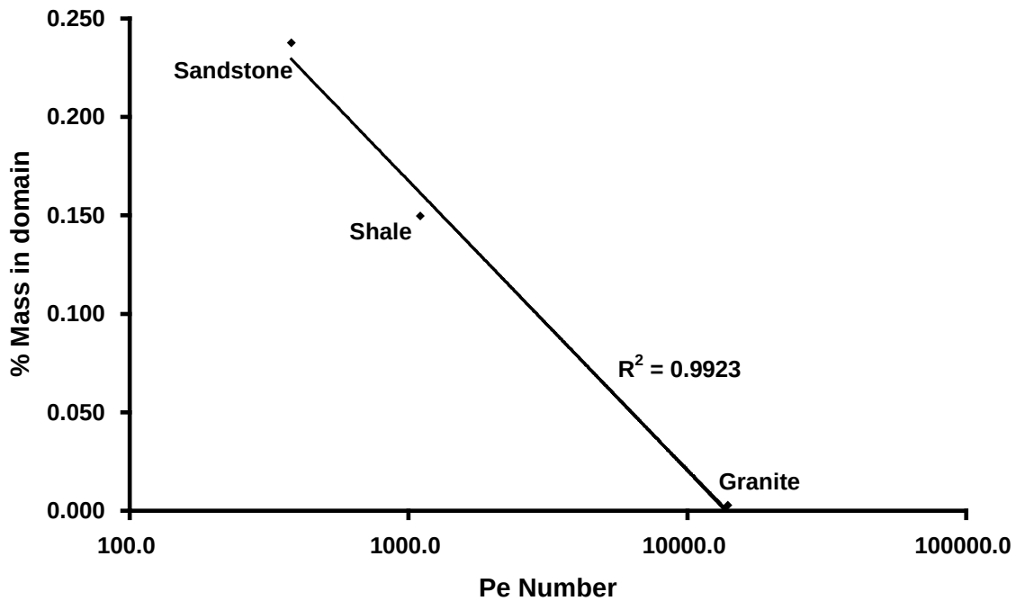
Figure 29: Mass of aqueous and sorbed TCE in various rock domains at end of Site Ageing stage (i.e., t_{TOTAL} = 21 years) vs. Peclet number (log scale) for each individual domain.
