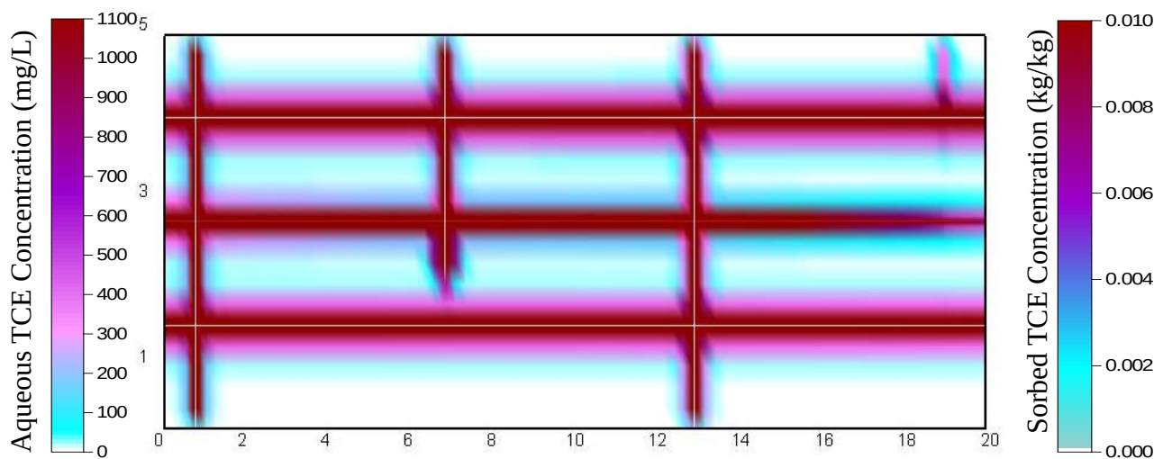
Figure 6: Distribution of aqueous and sorbed TCE after 20 years ( t_{\text{TOTAL}} = 21 years) of DNAPL dissolution (i.e., Site Ageing stage).
