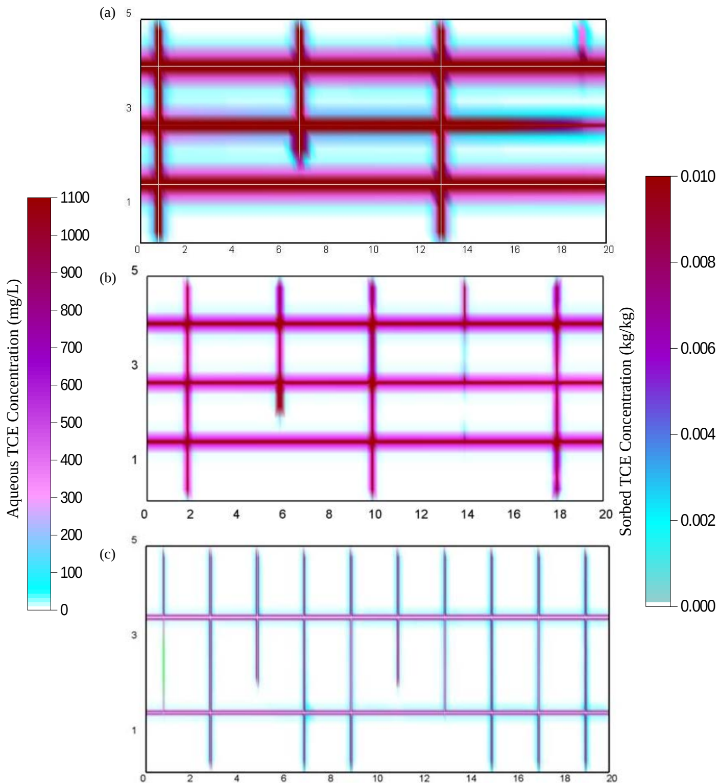
Figure 16: Distribution of aqueous TCE after 20 years ( t_{\text{TOTAL}} = 21 years) of DNAPL dissolution (i.e., Site Ageing stage) in (a) Sandstone, (b) Shale and (c) Granite.
