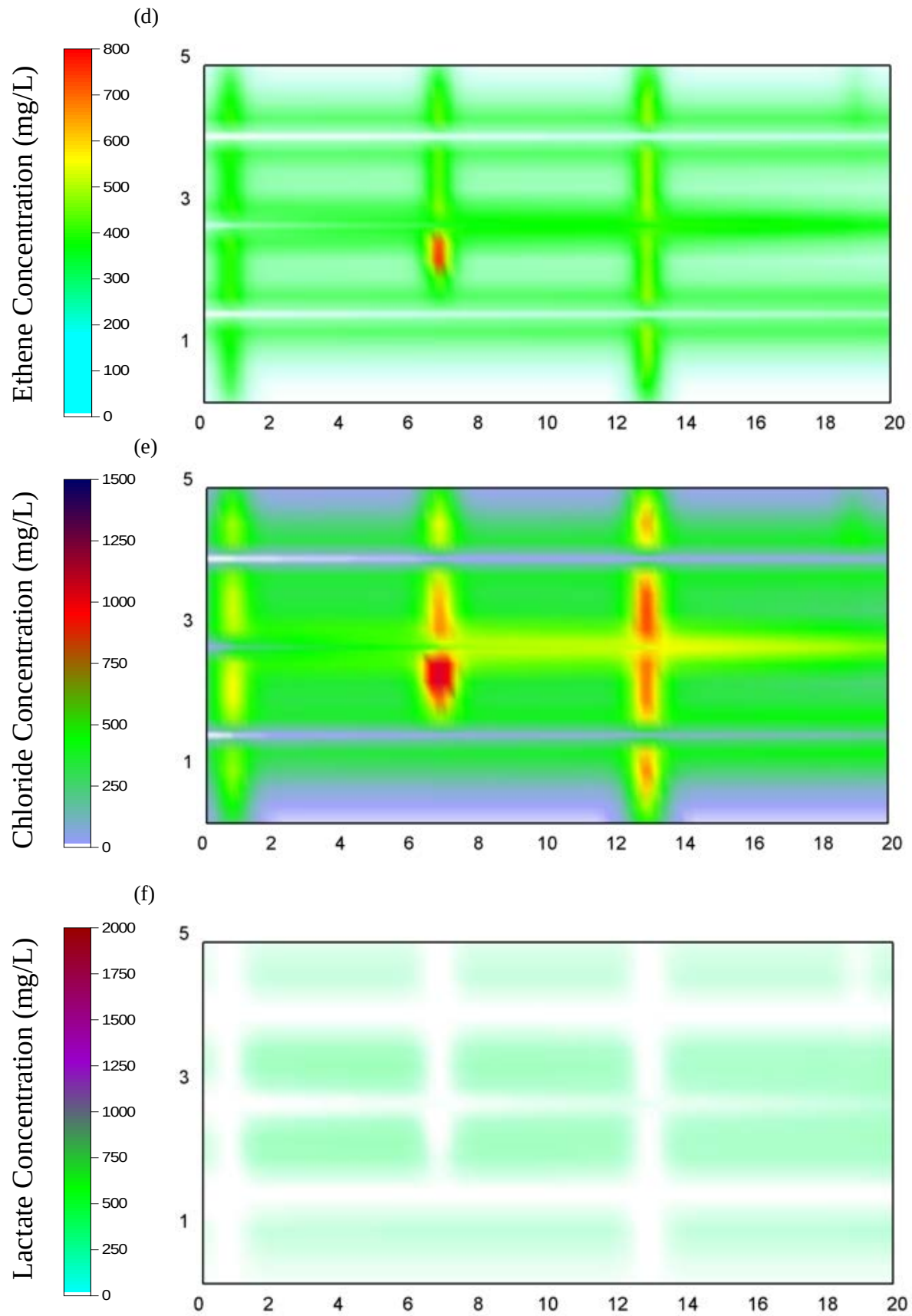
Figure 8: Distribution of aqueous species concentrations at t_{\text{TOTAL}} = 28 years for Base Case (i.e., 5 years Post-Treatment stage): (a) TCE; (b) 1,1, DCE; (c) VC; (d) Ethene; (e) Chloride; (f) Lactate.
