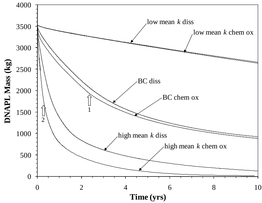
Figure 3. Influence of domain mean k on source zone DNAPL mass depletion. Label 'diss' denotes the case of dissolution only (no treatment) while simulations with chemical oxidation by potassium permanganate are labeled 'chem ox'. Label 'BC' denotes the base case with TCE. Vertical arrows indicate the time when treatment was terminated and the number beneath the arrow denotes the simulation number from Table 4. Note that treatment was not terminated for the low mean k template site.
