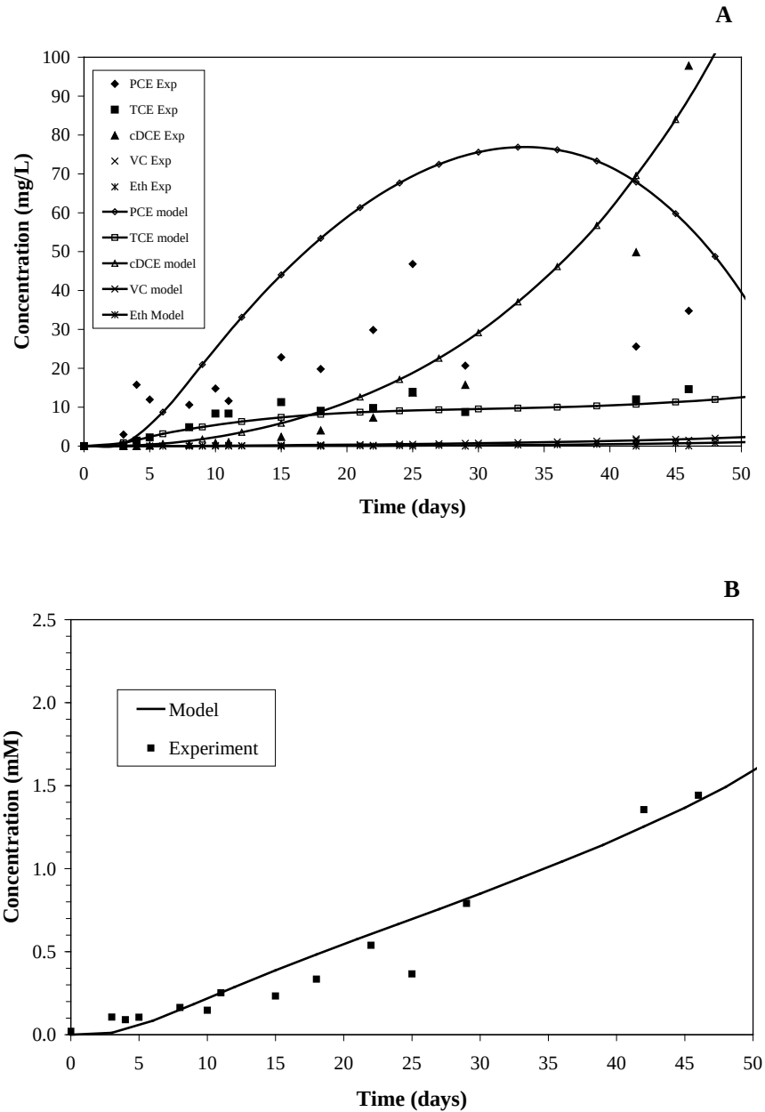
Figure 3. Comparison of DNAPL3D-RX (“Model”) to the column experiment by Yang and McCarty (2000b) for sequential degradation of PCE DNAPL in the presence of fermentors converting pentanol to H_2 for the first 50 days (adopted from Yang and McCarty, 2000b, Figure 8). Plot A is the effluent concentrations for each of PCE, TCE, cDCE, VC, and Eth. Plot B is for total ethenes.
