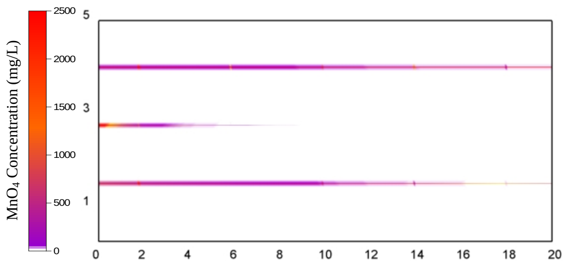
Figure A10: Distribution of MnO 4 concentrations at t_{\text{TOTAL}} = 22 years for Shale, 1 years after chemical oxidation
