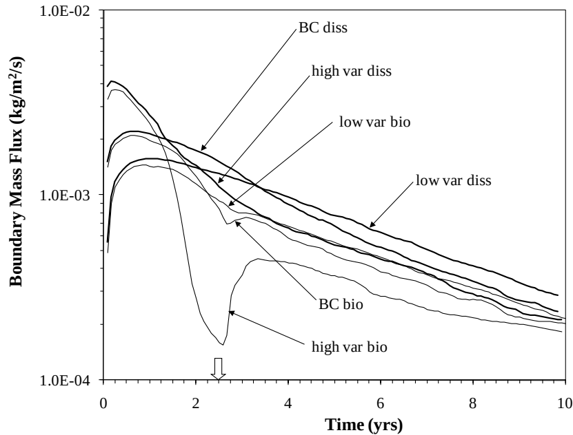
Figure 15. Influence of domain heterogeneity on downgradient solute boundary mass flux. The label ‘var’ refers to the variance in heterogeneity. The vertical arrow denotes the end of active treatment at 2.5 years for all simulations.
