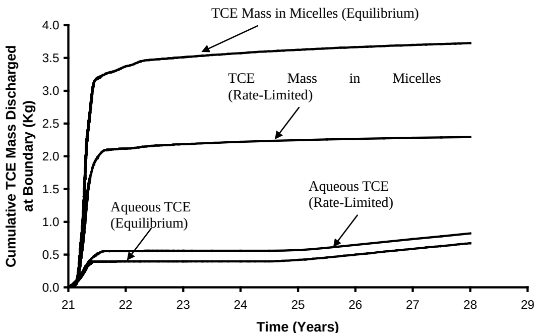
Figure 40: Cumulative mass discharged at downgradient boundary for (a) equilibrium and (b) rate limited mass transfer model.
