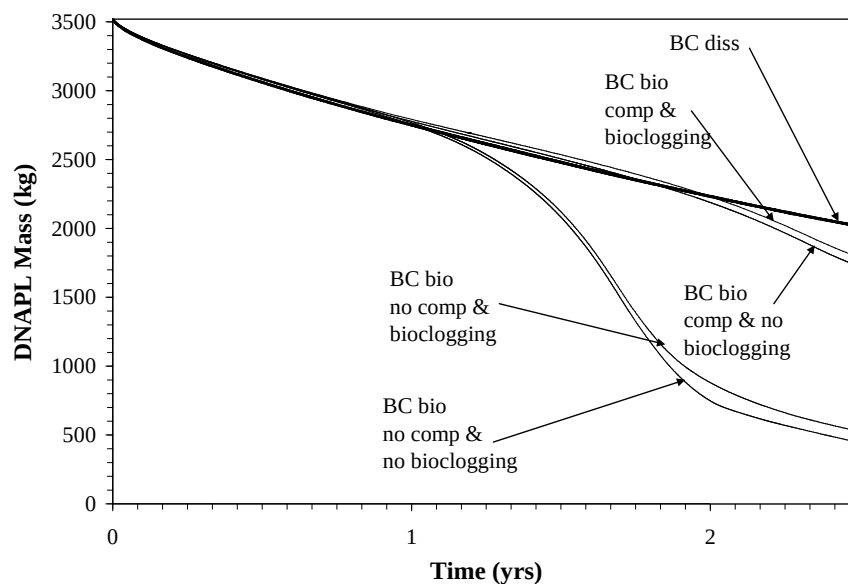
Figure 13. Influence of bioclogging and competition with methanogens on source zone DNAPL mass depletion. Treatment was terminated at 2.5 years.
