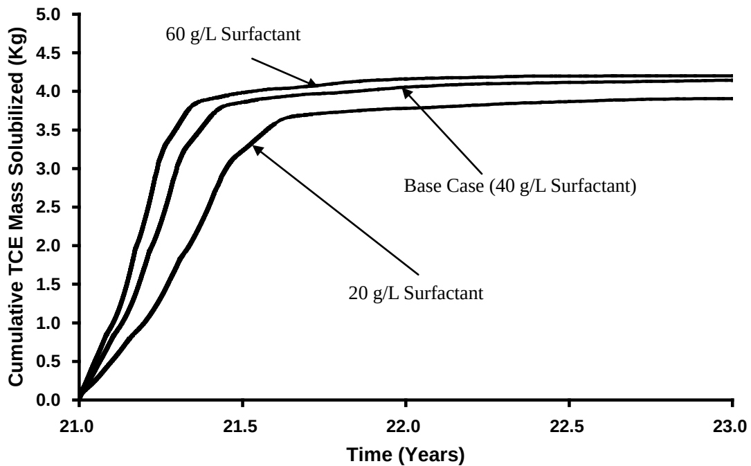
Figure 20: Cumulative mass of TCE solubilised by micelles over time for different injected concentration.
