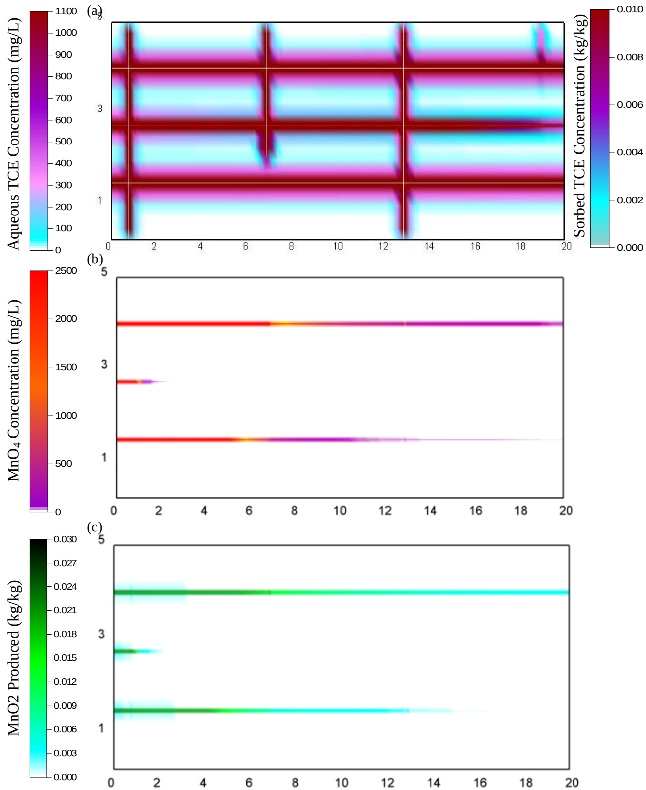
Figure A4: Distribution of aqueous species concentrations at t_{\text{TOTAL}} = 23 years for 6 Months Pulsing Simulation, after 2 years of chemical oxidation, aging period: (a) TCE, (b) \text{MnO}_4^- , (c) \text{MnO}_2
