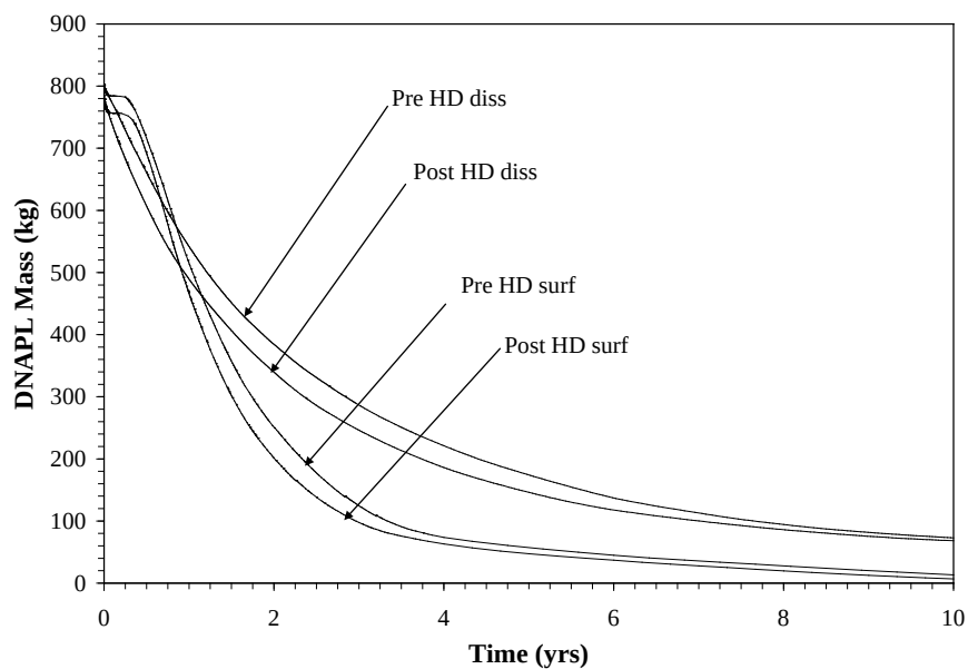
Figure 9. Influence of pre- and post-hydraulic displacement (HD) small DNAPL volume template sites. Surfactant injection times for the pre- and post-HD simulations were 5 days (see Table 3). Vertical arrows denote injection times greater than 20 days.
