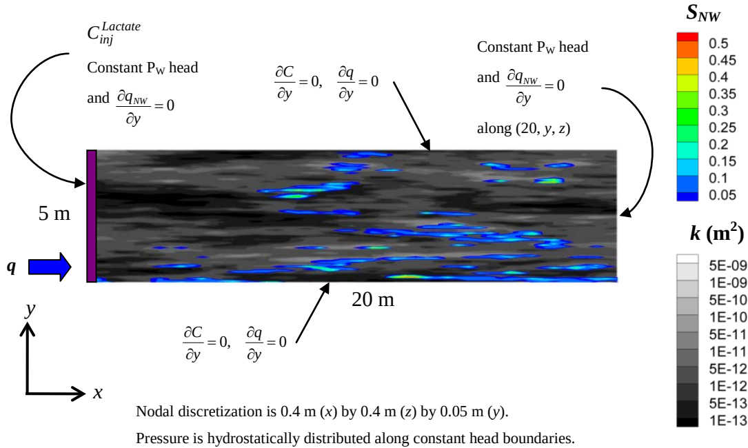
Figure 5. Cross-section of model domain with boundary and initial conditions. Section located at a z = 5 m for TCE base case.
