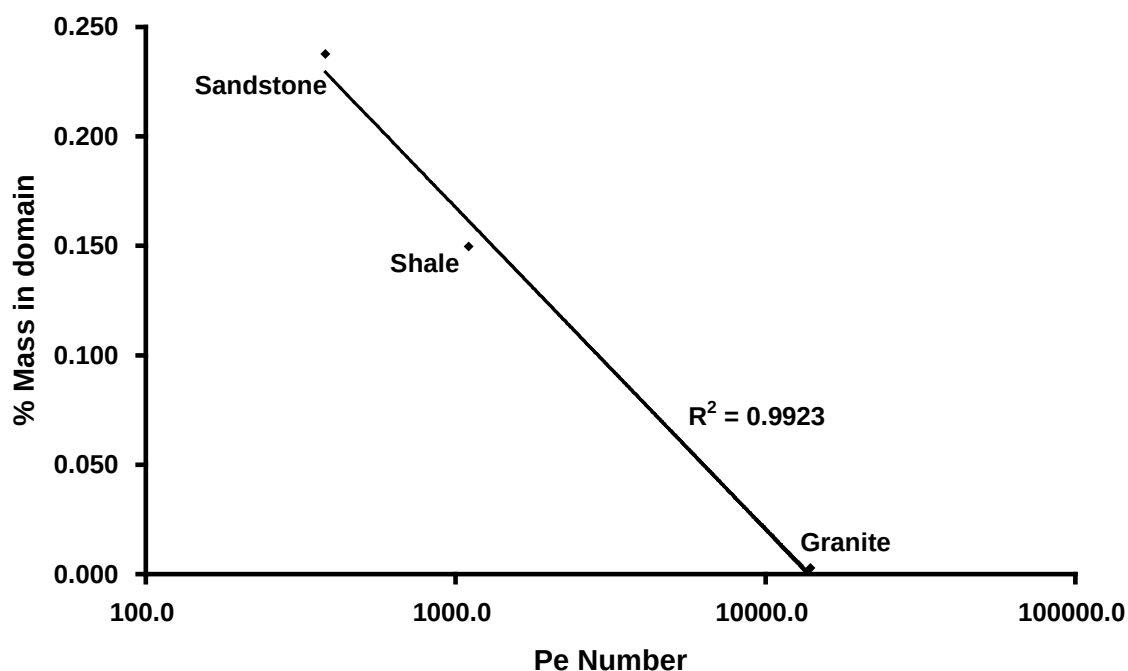
Figure 28: Mass of aqueous and sorbed TCE in various rock domains at end of Site Ageing stage (i.e., t_{TOTAL} = 21 years) vs. Peclet number (log scale) for each individual domain.
