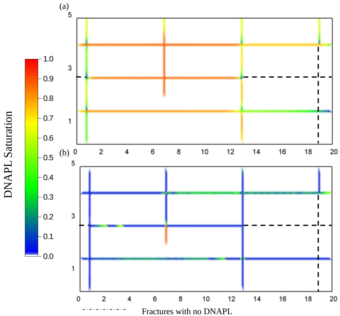
Figure 3: DNAPL distribution for Base Case at (a) t_{TOTAL} = 0.5 years when DNAPL inflow and outflow are equal, and (b) t_{TOTAL} = 1 year when all DNAPL migration has ceased.
