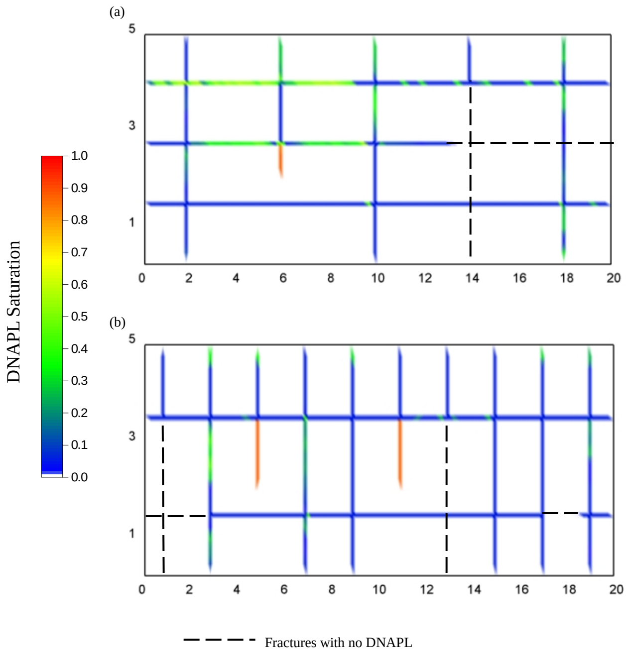
Figure A6: DNAPL distribution for (a) Shale and (b) Granite at t_{\text{TOTAL}} = 1 year when all DNAPL migration has ceased.
