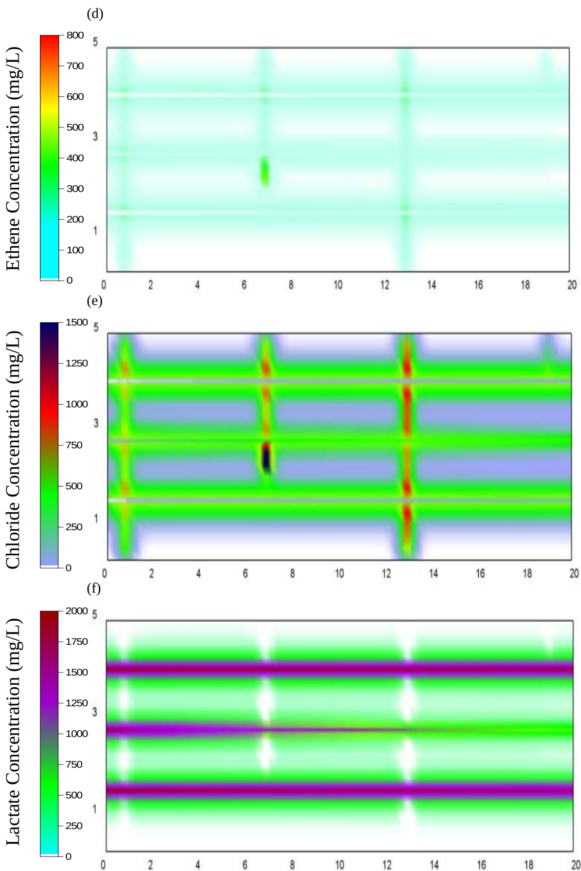
Figure 7: Distribution of aqueous species concentrations at t_{\text{TOTAL}} = 23 years for Base Case after 2 years of lactate injection (i.e., Treatment stage): (a) TCE; (b) 1,1, DCE; (c) VC; (d) Ethene; (e) Chloride; (f) Lactate.
