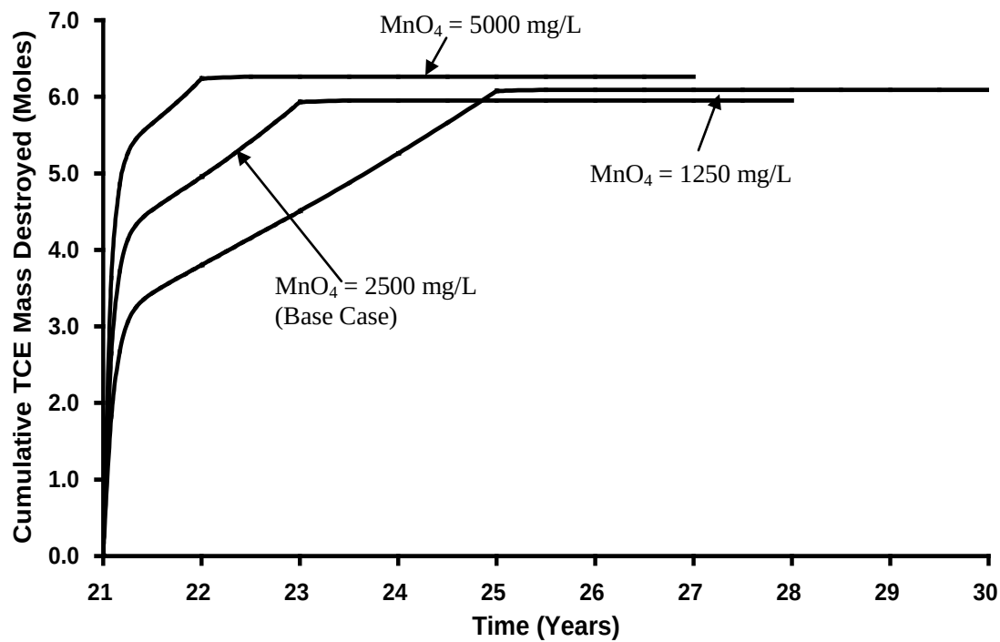
Figure 12: Cumulative mass of TCE destroyed for various \text{MnO}_4 concentrations.
