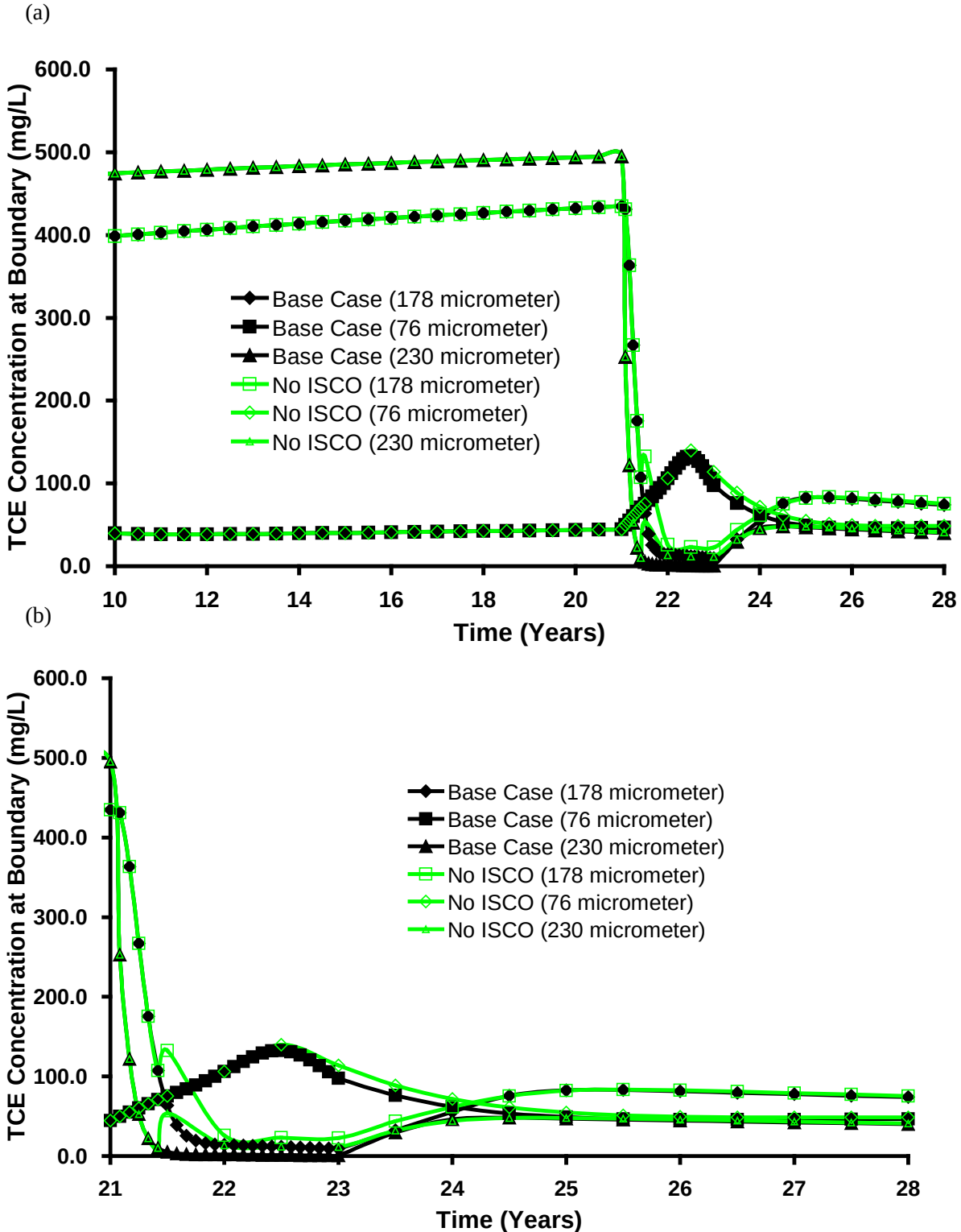
Figure 11: Concentration of TCE at all three horizontal fractures in the Sandstone base case at the downgradient boundary over (a) the latter 18 years, and (b) since the start of the Treatment stage only (timescale expanded for clarity).
