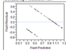
Residual by Predicted Plot
