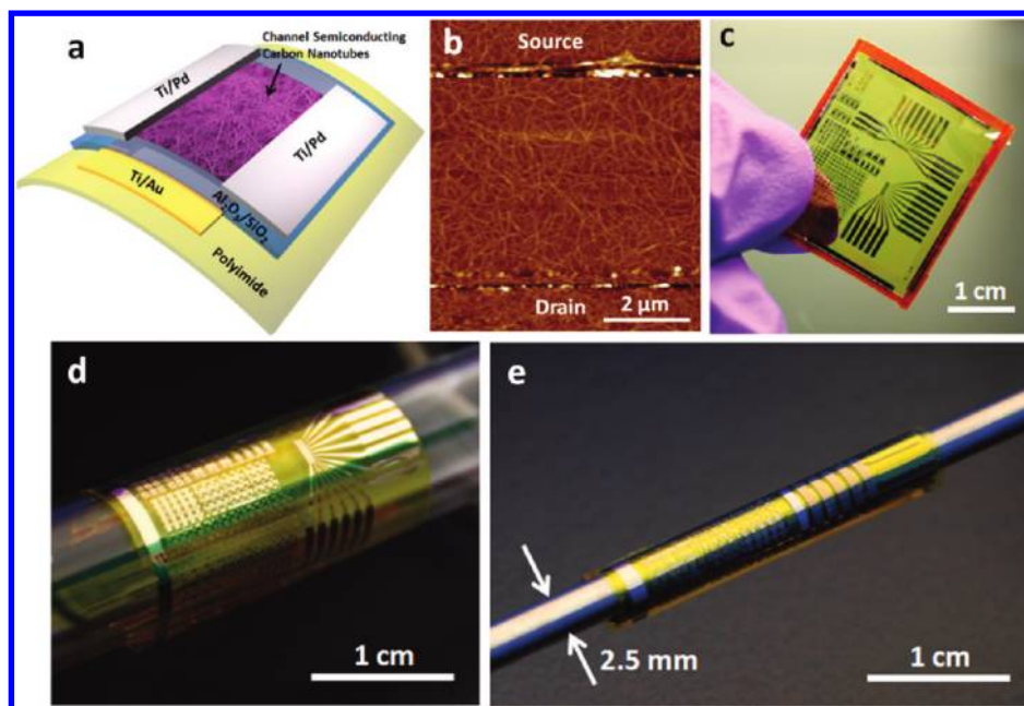
Figure 1. Flexible thin-film transistors and integrated circuits using semiconducting carbon nanotube networks. (a) Schematic diagram of a local-gated nanotube TFT on a flexible substrate. (b) AFM image showing the channel of the flexible nanotube TFT, which consists of random networks of semiconducting carbon nanotubes. (c) Photograph of a flexible nanotube circuit with a size of \sim 2.5 \times 3 \text{ cm}^2 . (d,e) Photographs showing the extreme bendability of the flexible nanotube circuits, where the samples are being rolled onto a test tube with a diameter of 10 mm (d), and a metal rod with a diameter of 2.5 mm (e).
