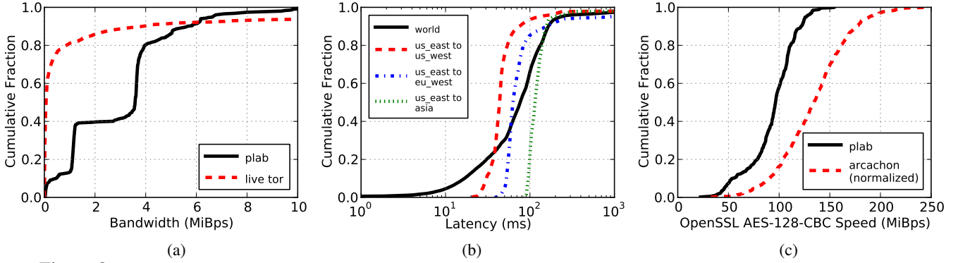
Figure 8: Network and CPU measurements used for Shadow experiments. (a) Bandwidth measurements of PlanetLab nodes and live Tor relays. Relay bandwidth values were taken from a live consensus. (b) Latency between PlanetLab nodes, shown as aggregate (“world”) and inter-region latency measurements. (c) Measured CPU speeds for PlanetLab nodes and our Intel Core2 Duo lab machine arcachon . The results from arcachon were normalized to create a distribution usable in Shadow.
