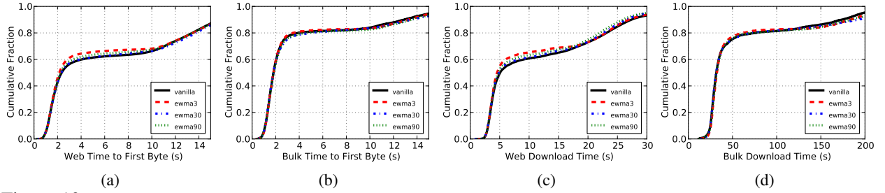
Figure 10: Network performance under an extremely light load of 475 web and 25 bulk clients. When the network load is too light, the circuit scheduling algorithm has an insignificant impact on performance.
