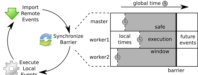
Figure 7: Main loop and conservative multi-process synchronization using dynamic barriers. Safe execution windows are calculated using the minimum local worker time plus the minimum simulated latency between nodes. The barrier is dynamically pushed as local times advance.
