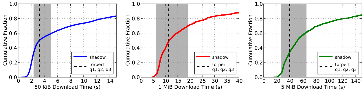
Figure 4: Shadow-Tor compared with live-Tor network performance. TorPerf represents statistics from metrics.torproject.org . The gray area shows TorPerf first to third quartile stretch while the dotted line represents the TorPerf median. Shadow closely approximates Tor performance for all file sizes.
