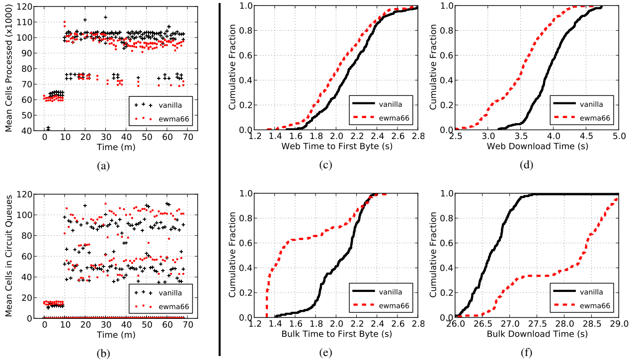
Figure 5: Seven-node bottleneck experiment similar to that performed by Tang and Goldberg [42]. The number of cells processed (a) and queued (b) increases at Time=10, when the measurement clients begin downloading. The EWMA scheduler improves responsiveness for bursty traffic (c), (d), and (e) but, contrary to the author’s claims, decreases performance for bulk downloads (f).
