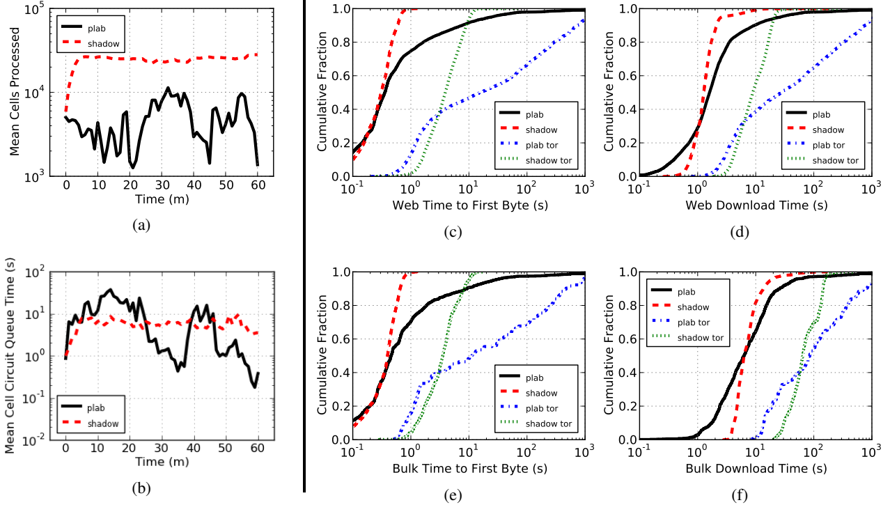
Figure 3: Shadow and PlanetLab network performance. PlanetLab download experiments were run with and without Tor and mirrored in Shadow. As shown in (a) and (b), Shadow approximates PlanetLab performance reasonably well while PlanetLab results show higher variability due to co-location and network/hardware interruptions. Also shown are CDFs of the number of elapsed seconds until the first byte of a 320 KiB file (c) and a 5 MiB file (e) is received, and the time to complete a download of the same files (d), (f).
