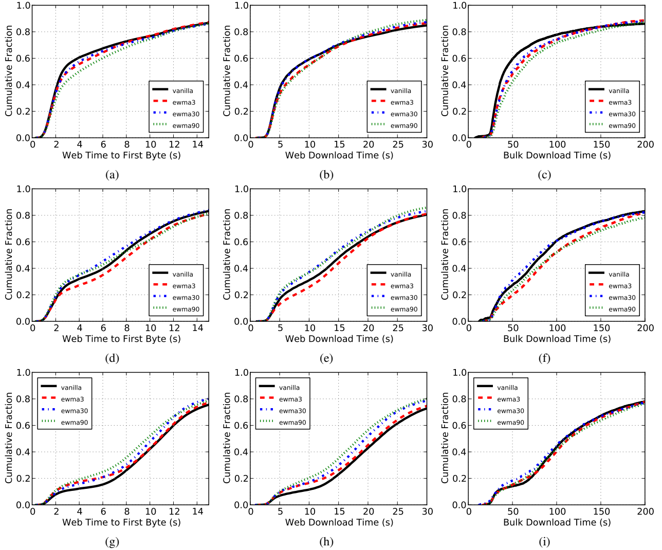
Figure 6: Performance of a full-network deployment of the EWMA circuit scheduler and vanilla Tor using a round-robin scheduler. Load is generated with 950 web clients and varied using (a)–(c) 25 bulk clients (d)–(f) 50 bulk clients, and (g)–(i) 100 bulk clients. While the EWMA circuit scheduler works best under heavily loaded networks, there are EWMA half-life configurations that lead to reduced client performance.
