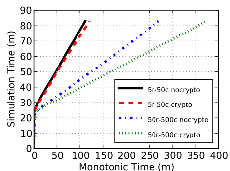
Figure 2: Simulation vs. wall clock time. Skipping expensive cryptographic operations results in a linear decrease in experiment runtime – nearly a one-third reduction in runtime for a small, 550-node Tor experiment.
