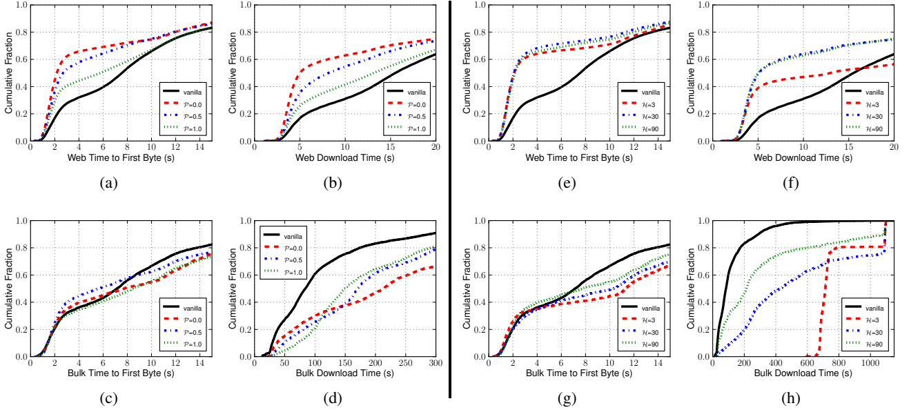
Figure 4: Throttling clients by flagging bulk connections. Flagged connections are rate-limited at 5 KiBps until their cell count EWMA reaches fraction \mathcal{P} of the fair bandwidth cell count EWMA. (a)–(d) use a constant per-connection half-life \mathcal{H} of 90 seconds and varies \mathcal{P} , affecting the length of the throttling period, and (e)–(h) vary \mathcal{H} , affecting the ability to differentiate bulk from web connections, while keeping \mathcal{P} constant at 0.0.
