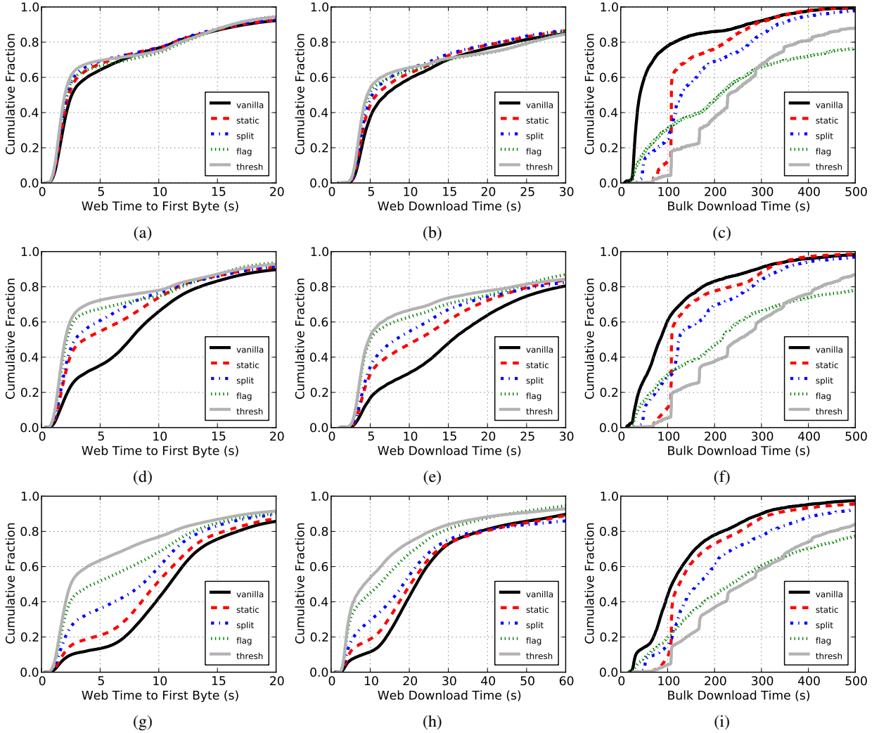
Figure 6: Comparison of client performance for each throttling algorithm and vanilla Tor, under various load. All experiments use 950 web clients while bulk clients are adjusted to 25 for (a)–(c), left at the default of 50 for (d)–(f), and adjusted to 100 for (g)–(i). The parameters for each algorithm are tuned to maximize client performance, according to experiments presented in Section 4.
