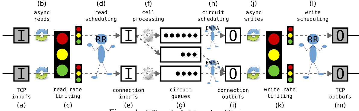
Figure 1: A Tor relay's internal architecture.
