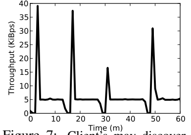
Figure 7: Client’s may discover the throttle rate by probing guards.
