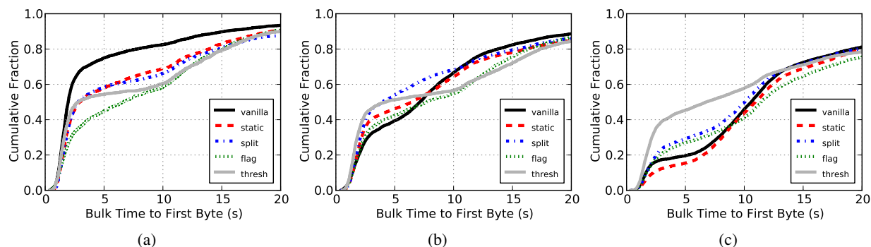
Figure 10: Comparison of responsiveness for bulk clients for each throttling algorithm and vanilla Tor, under various load. All experiments use 950 web clients while bulk clients are adjusted to 25 for (a), 50 for (b), and 100 for (c). The parameters for each algorithm are tuned to maximize client performance, according to experiments presented in Section 4.
