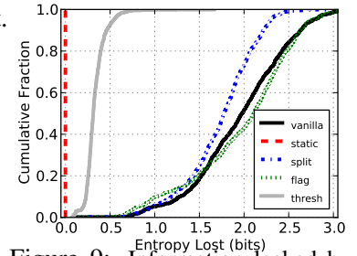
Figure 9: Information leaked by learning guards’ throttle rates.
