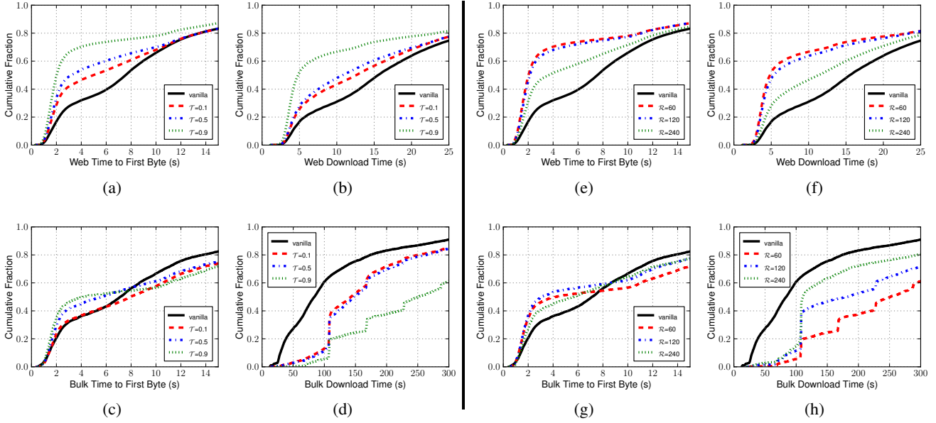
Figure 5: Throttling clients using thresholds. The threshold \mathcal{T} configures the loudest fraction of connections that get throttled, while the throttle rate is obtained from the average throughput of the \mathcal{T}^{th} loudest connection over the last \mathcal{R} seconds. (a)–(d) show performance while varying \mathcal{T} as shown with a constant \mathcal{R} of 60 seconds. (e)–(h) hold \mathcal{T} constant at 0.9 while varying \mathcal{R} as shown. A 90 percent threshold and 60 second refresh period shows the best performance for interactive clients in our simulations while flooring the throttle rate at \mathcal{F} = 50 KiBps.
