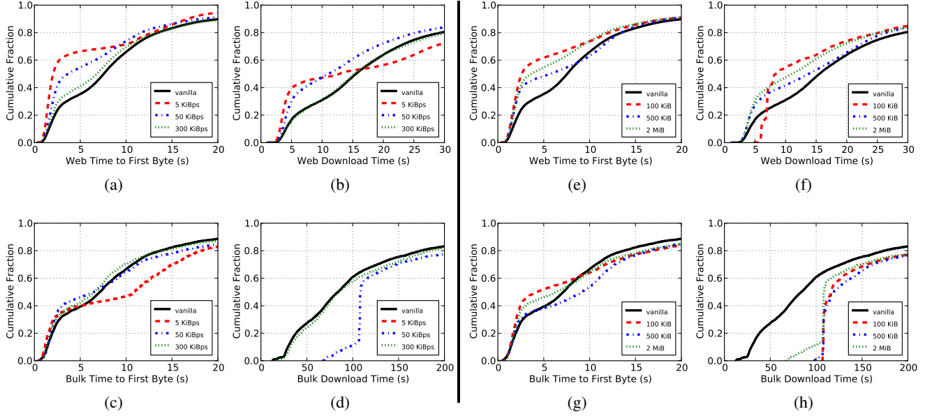
Figure 2: Throttling clients with static throttle configurations. (a)–(d) show performance with a varied PerConnBWRate as shown and a constant 2 MiB PerConnBWBurst while (e)–(h) use a constant 50 KiBps PerConnBWRate and varied PerConnBWBurst as shown. A rate of 50 KiBps and burst of 2 MiB leads to the most significant performance improvements in our simulations.
