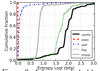
Figure 8: Information leaked by learning circuit throughputs.
