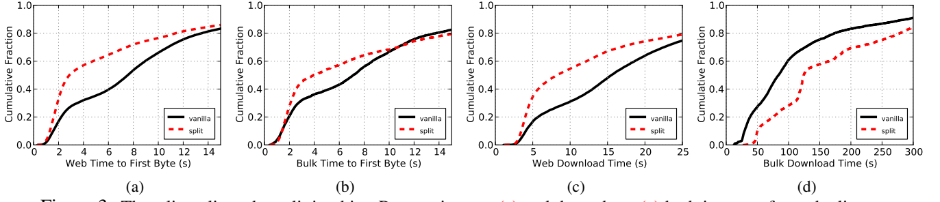
Figure 3: Throttling clients by splitting bits. Responsiveness (a) and throughput (c) both improve for web clients at the expense of bulk throughput (d).
