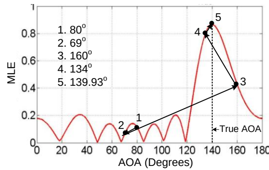
Figure 3. Illustration of a contractive map simulation example.
