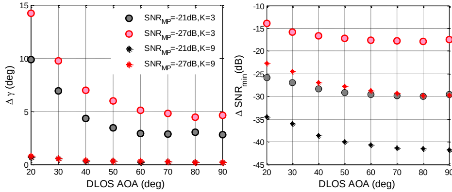
Fig. 6. \Delta\phi_{\text{blind}} (top) and \Delta\text{SNR}_{\text{min}} (bottom) for K=3 and 9, multipath SNR=-21dB and -27dB for DLOS AOAs between 20° and 90°.
