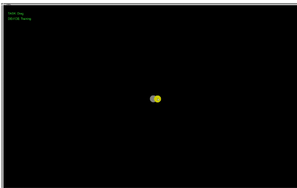
Figure 9. Dragging task.
