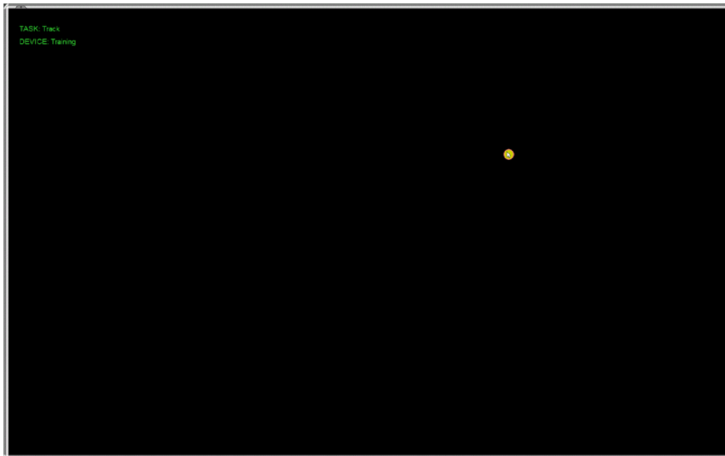
Figure 8. Tracking task.
