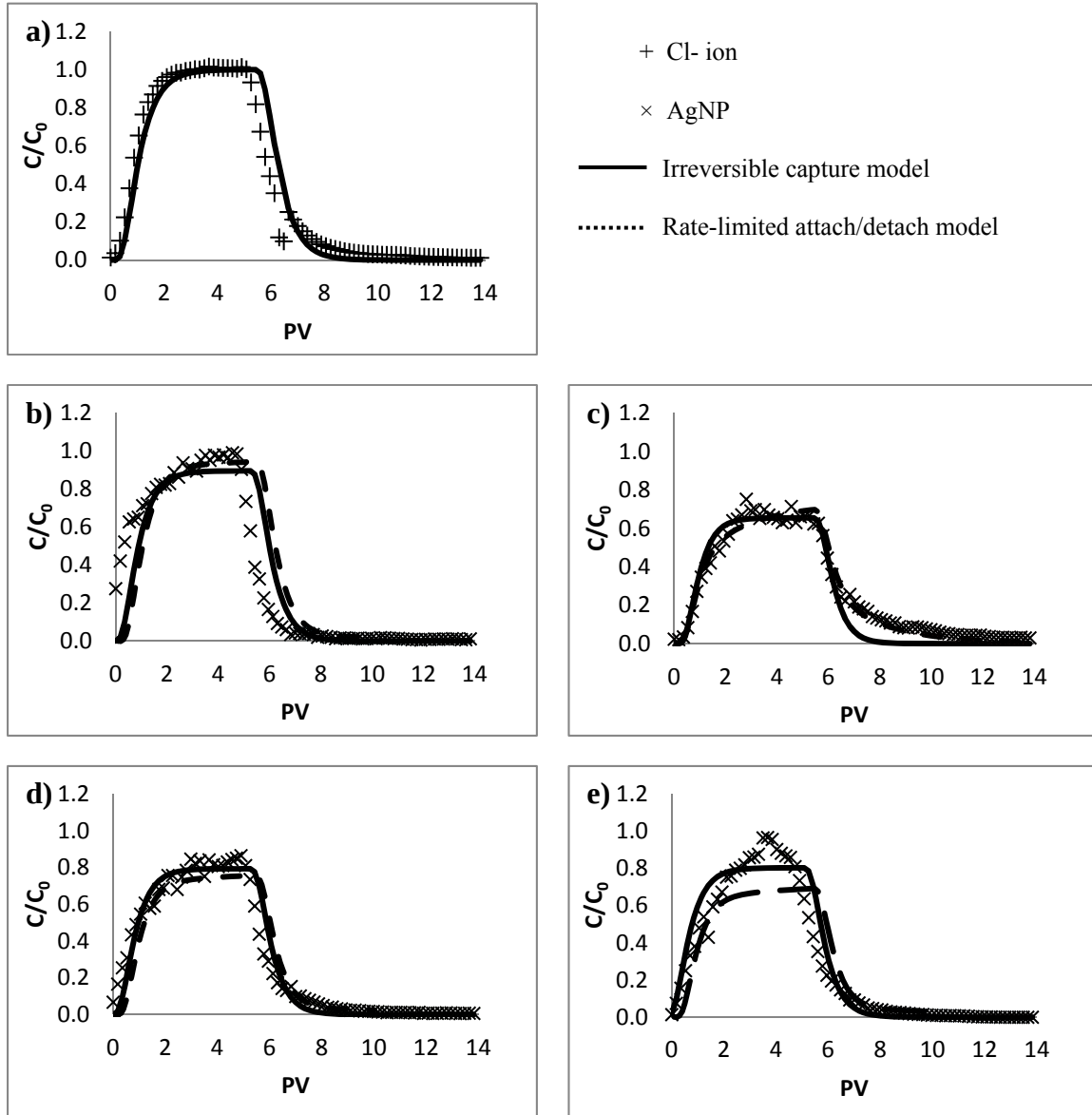
Figure 4: Breakthrough curves for (a) Cl ion and AgNPs at (b) pH 4, (c) pH 6.5, (d) pH 9 and (e) pH 11, along with model fits. Experimental conditions: Cl ion: C_0 = 100 mg/L, AgNP: C_0 \sim 20 mg/L, ionic strength: 0.01 mM KCl and flow rate: 1 mL/min
