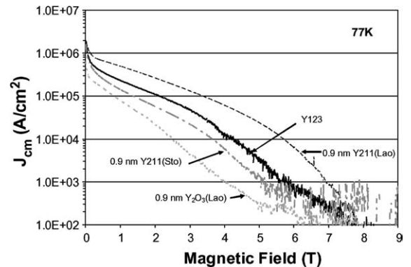
Fig. 10. J_{cm} comparison of Y_2O_3 /Y123 multilayer film with 0.9 nm Y_2O_3 pseudo-layer thickness and Y211/Y123 multilayer films with 0.9 nm Y211 pseudo-layer thickness, each with approximately equal Y123 layer thickness. The plot shows the deterioration of film properties due to the increased Y_2O_3 pseudo-layer thickness.
