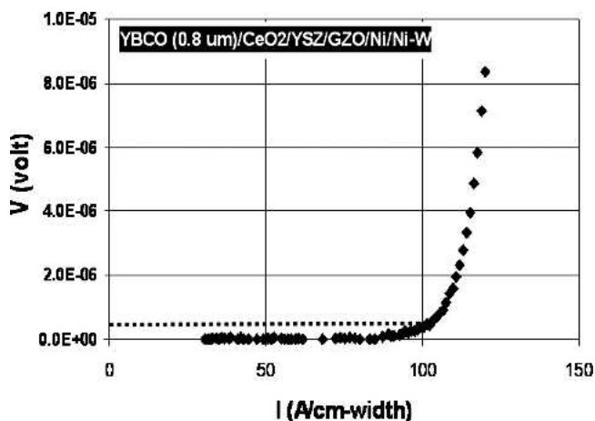
FIG. 9. Current-voltage curve of a YBCO/ \text{CeO}_2 /YSZ/GZO/Ni/Ni-W sample, where YBCO is processed via the ex situ TFA approach. The dashed line indicates the voltage criterion for definition of I_c .
