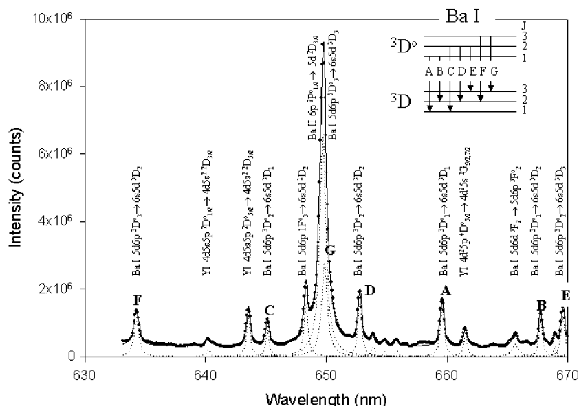
Fig. 3. Portion of the visible plume emission spectrum showing the seven components of the Ba I 5d6p ^3D^\circ \rightarrow 6s5d \ ^3D fine structure. The spectrum was fit to a series of Lorentzian profiles (··) to determine the relative intensities of the various spectral features.
