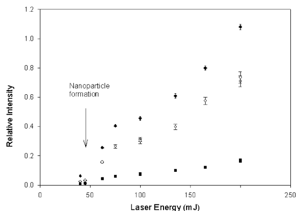
Fig. 4. Emission intensity from neutral Ba (■) ^1P_1 \rightarrow ^1S_0 at \lambda = 553.5 nm, Y (◆) ^2D_{5/2}^\circ \rightarrow ^2D_{5/2} at \lambda = 643.5 nm, and Cu (○) ^2P_{3/2}^\circ \rightarrow ^2D_{5/2} at \lambda = 510.6 nm, as a function of laser energy.
