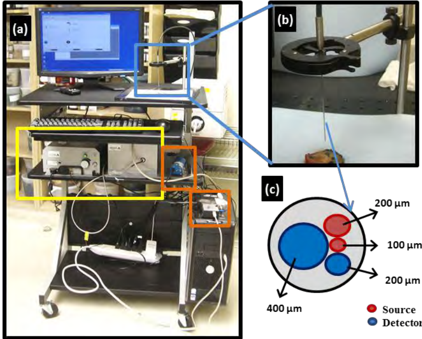
Fig. 1 (a) A photograph of the combined LRS/AFLM system for ex vivo human prostate specimen measurements. The yellow square contains the main AFLM hardware. The orange squares contain LRS hardware, namely the broadband light source and a CCD array spectrometer. (b) An inset of (a) showing a close up of the measurement geometry with the integrated probe, probe holder and tissue sample. (c) Detailed geometry of the probe tip. Two 200-μm fibers are connected to the LRS system; the other two fibers go to the AFLM system.
