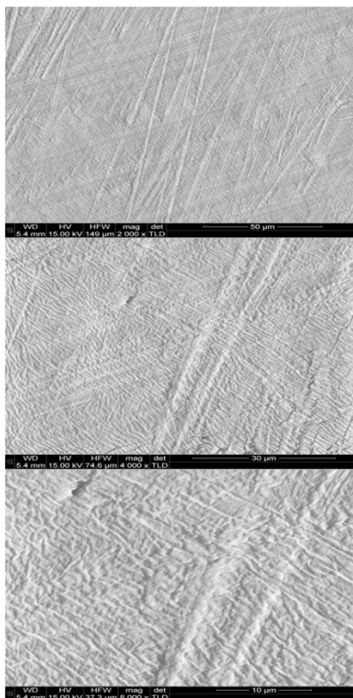
Figure 8. SEM image of the metalized surface of plasma-treated UHMWPE at different magnifications: (a) 2000 \times , (b) 4000 \times , and (c) 8000 \times .
