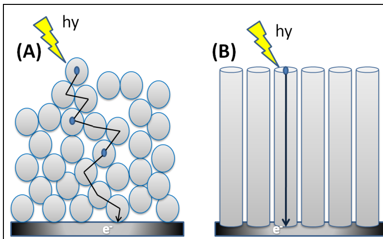
Figure 2. (a) Random electron path thru nanoparticles and (b) direct electron transport in nanotubes.
