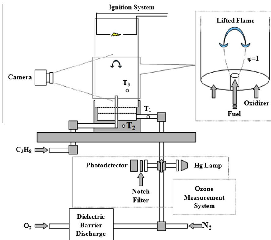
Fig. 2. Experimental set-up schematic of the lifted flame burner integrated with a dielectric barrier plasma discharge device and \text{O}_3 absorption measurement system.
