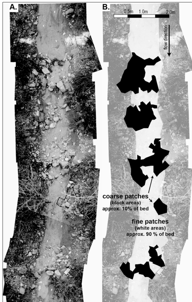
Figure 3. Photographic map of a section of the Lucky Hills channel bed without (A) and with (B) the patch boundaries delineated.
