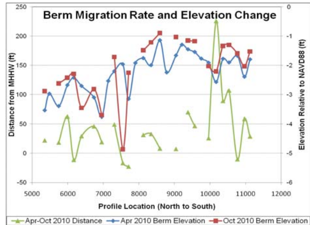
Figure 20. Longshore variations of berm crest elevation, and changes in distance from berm crest to MHHW line (green line). Profile location is referred to the distance to the northeastern most profile.
