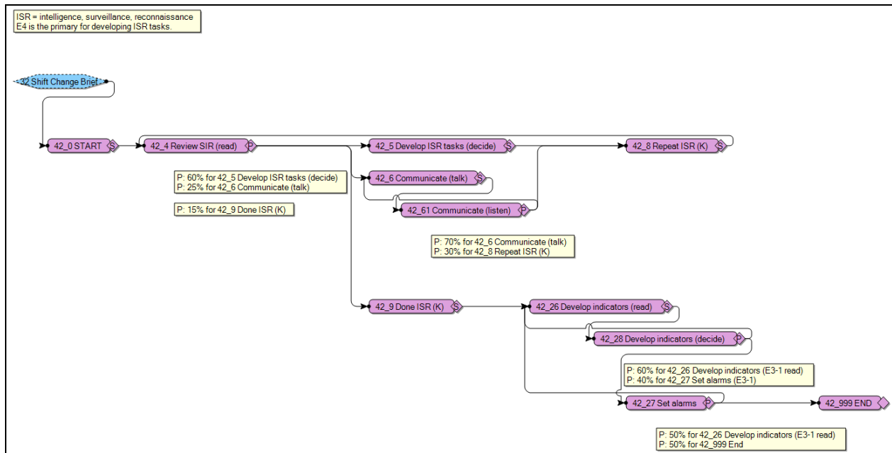
Figure 3. Baseline function Setup ISR —develop intelligence, surveillance, and reconnaissance tasks and requirements.
