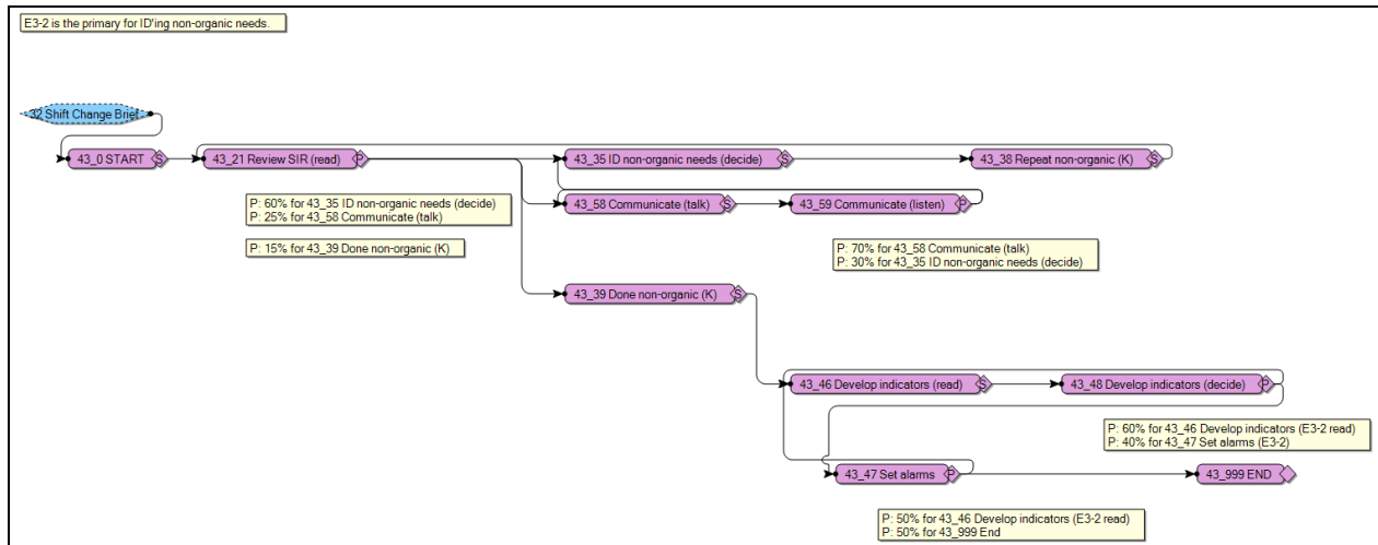
Figure 4. Baseline function Non-Organic Needs —develop non-organic asset and information requirements.
