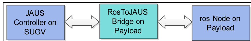
Figure 1. Message flow between the SUGV and ROS via the ROSToJAUSBridge.
