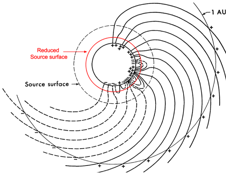
Figure 3 Cartoon illustrating that a smaller source surface will encompass more open field lines and enlarge the coronal hole areas from which the open field emanates. Note that the number of polarity reversals also increases. Figure adapted from Schatten, Wilcox, and Ness (1969).
