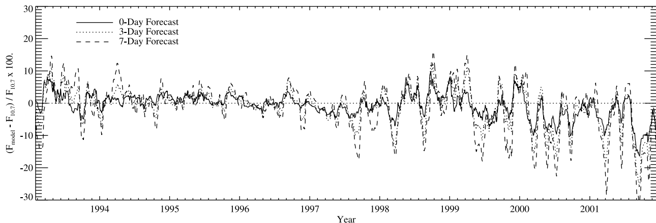
Figure 4. Interval A (1993–2001), the percent difference between the 0 day (solid), 3 day (dotted), and 7 day (dashed) ADAPT forecasts, and the adjusted observed F_{10.7} values. Smoothed with a 21 day running mean, the differences highlight how the forecasts generally underestimate F_{10.7} during high activity (1999–2001).
