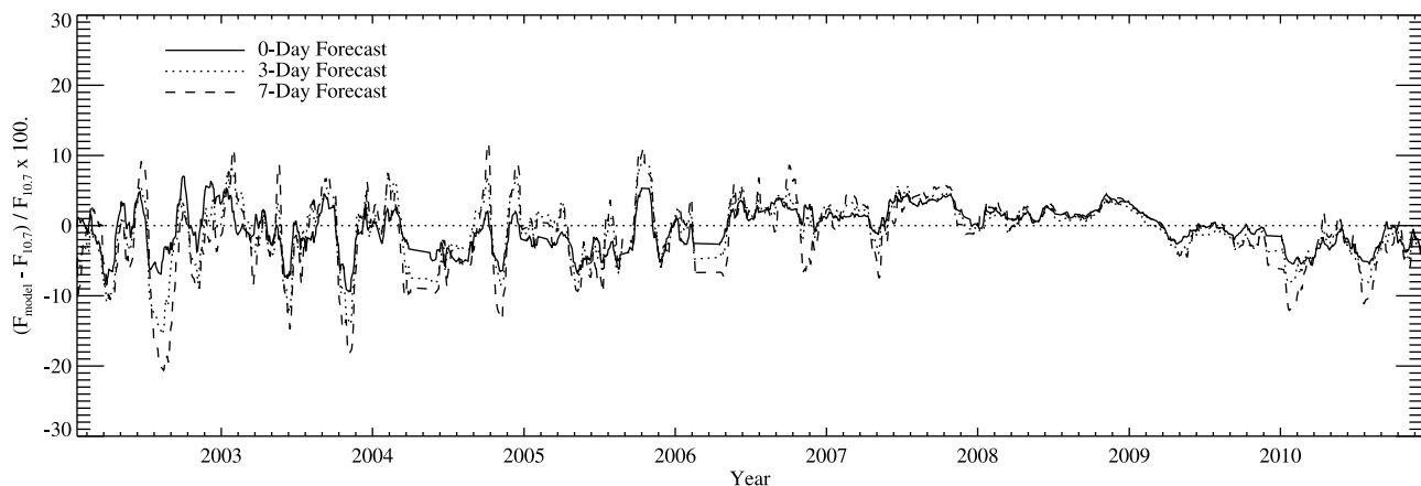
Figure 5. Interval B (2002–2010), the percent difference between the 0 day (solid), 3 day (dotted), and 7 day (dashed) ADAPT forecasts, and the adjusted observed F_{10.7} values. Smoothed with a 21 day running mean, the differences highlight how the forecasts generally underestimate F_{10.7} during high activity (2002–2006).
