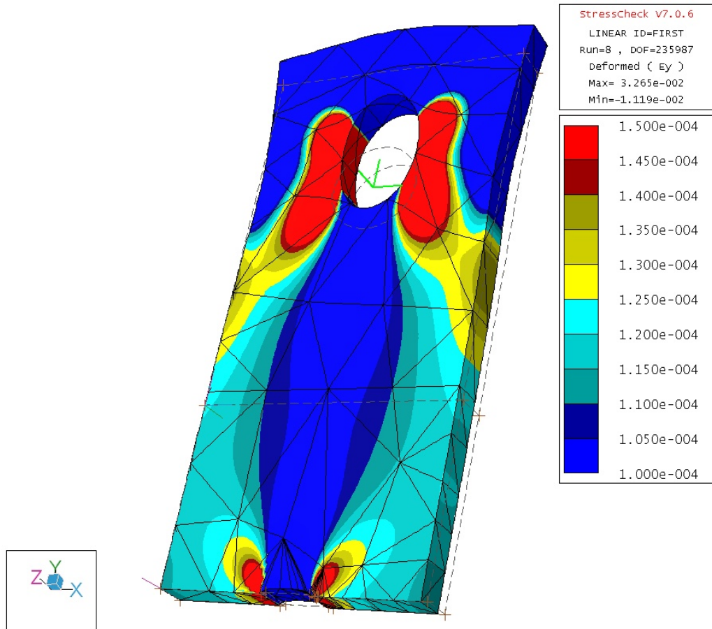
Figure 27. Early global model from StressCheck version 7.0.6. This plot shows y axis strain ( E_y ) with deformation
