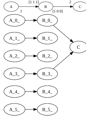
(b) CSDF graph to HSDF graph
