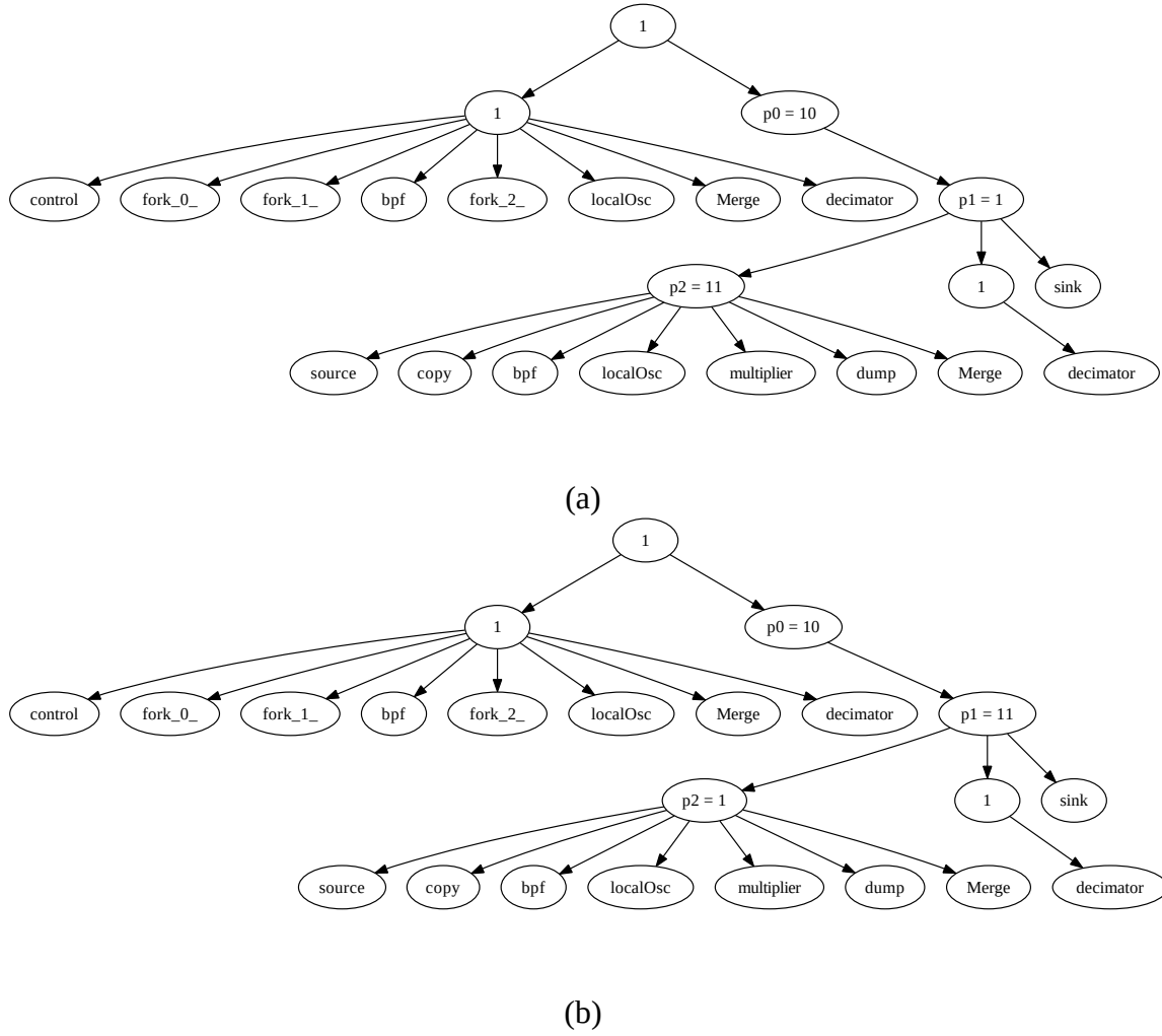
Figure 6.7: PLSs for the TDD application configured for a decimation factor of 11, and decimator actor employing the (a) PSDF and (b) PCSDF models of computation.
