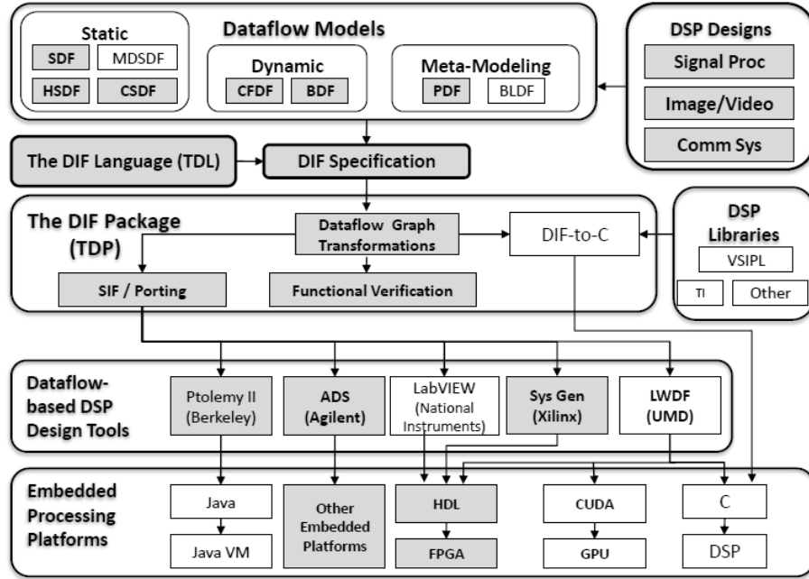
Figure 1.2: DIF based design flow.
