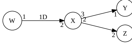
Figure 2.1: An SDF graph.
