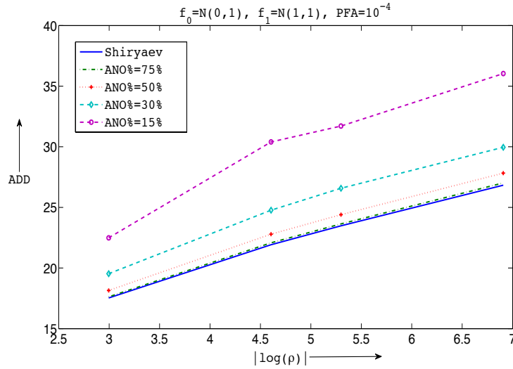
Figure 10.7: Trade-off curves comparing performance of two-threshold algorithm with the Shiryaev test for ANO% of 75, 50, 30 and 15%. f_0 \sim \mathcal{N}(0, 1) , f_1 \sim \mathcal{N}(1, 1) , and \text{PFA} = 10^{-4} .
