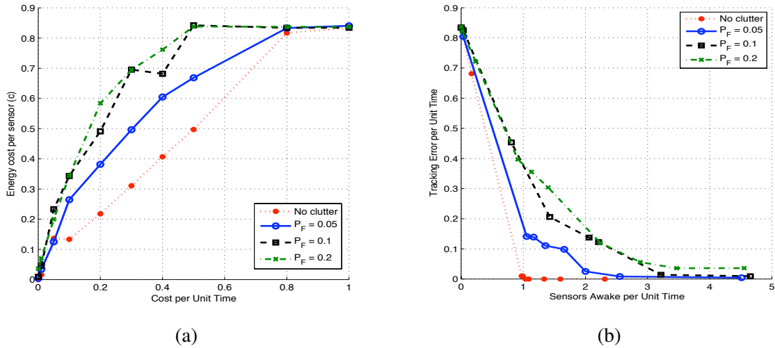
Figure 4.21: (a) Total cost per unit time versus energy cost per sensor for the overlap network; (b) Energy tracking tradeoff for different clutter densities for network with overlapping sensing ranges
