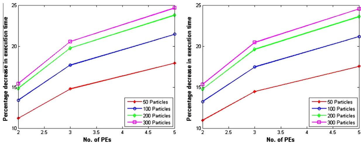
Fig. 10. Percentage decrease in execution time (1 iteration) for uni-variate non-stationary growth model and uni-dimensional failure prognosis model implementations.
