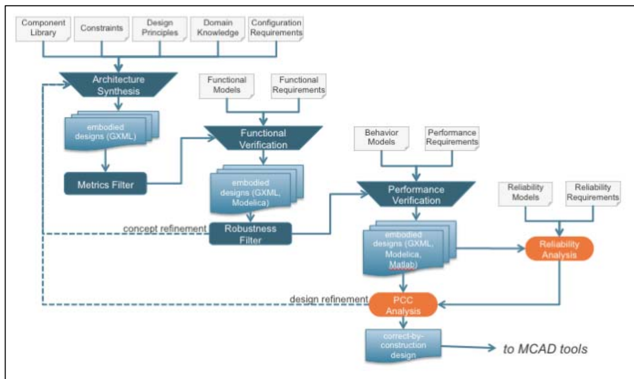
Figure 1. The Model-Based System-Engineering Process Flow
