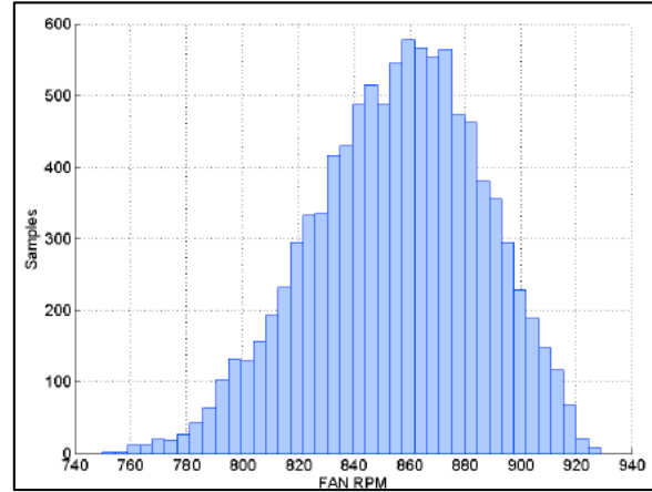
Figure 14. Phase 2/3 Output Distribution from MCS.
