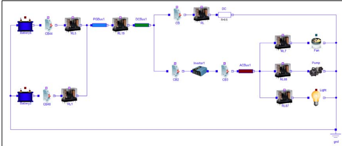
Figure 11. Automatically generated Modelica performance with redundant power sources.
