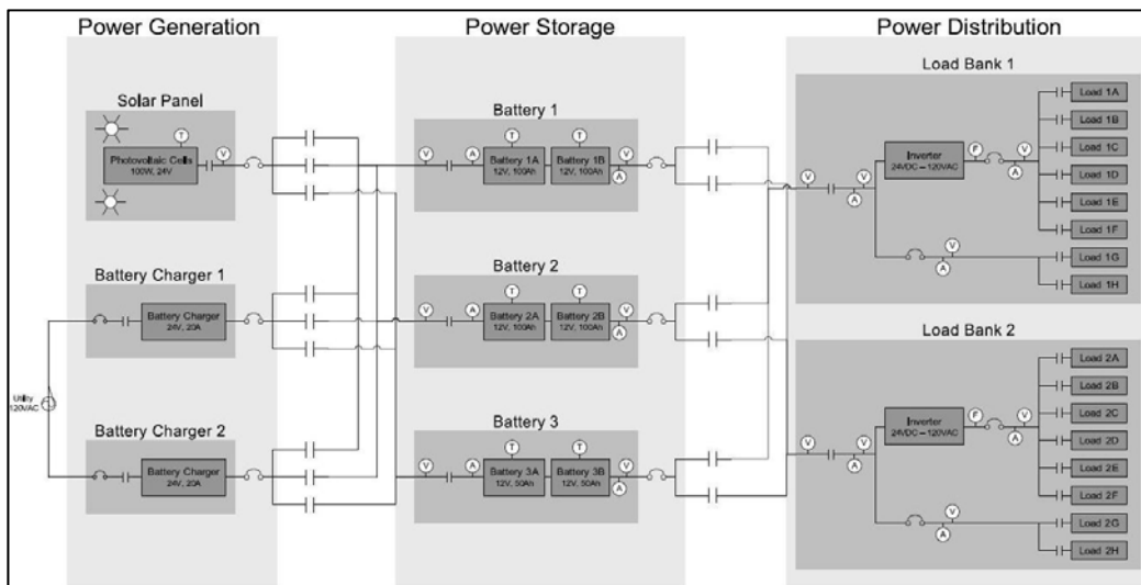
Figure 7. The ADAPT Testbed Structure (Picture Reproduced from [10])
