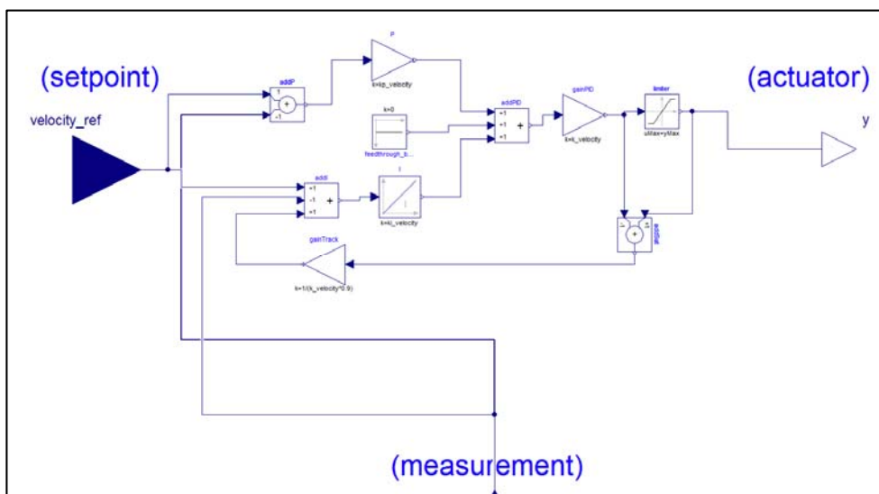
Figure 18. The Control Subsystem
