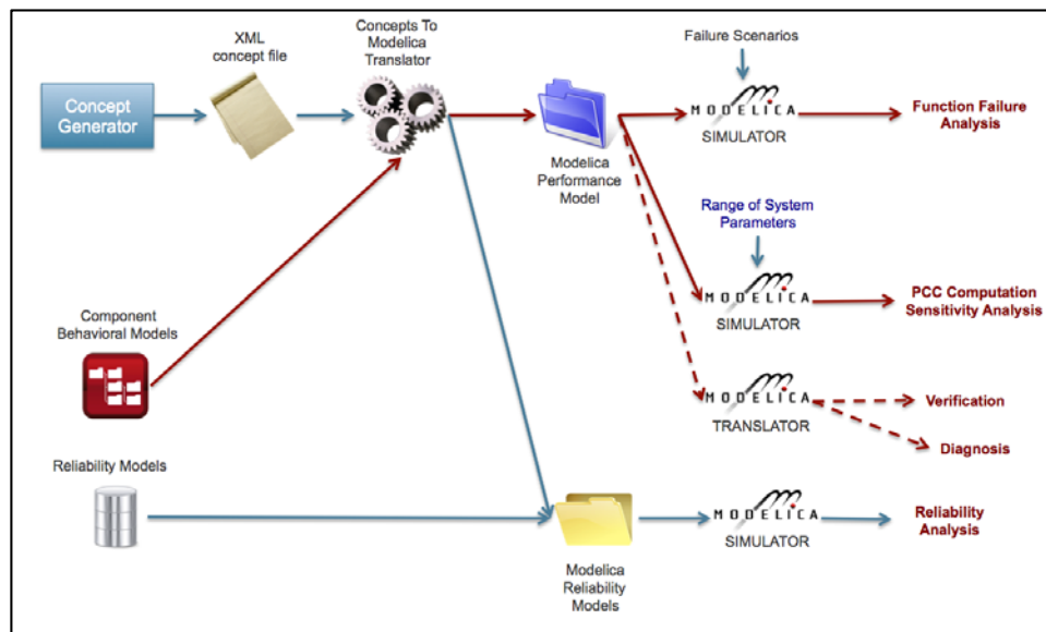
Figure 10: Type of Modelica models generated by the Automated Model Generator
