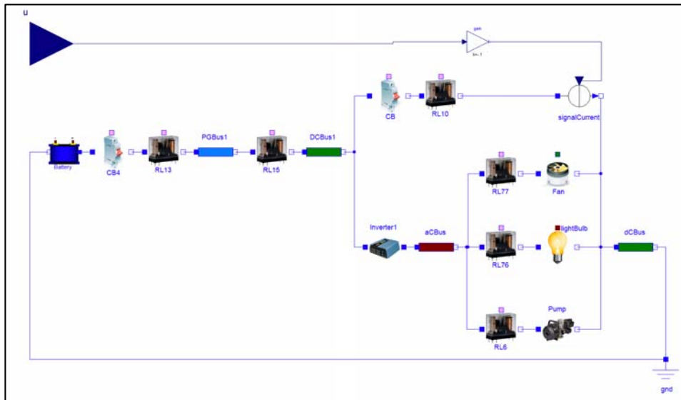
Figure17. The Electrical Power Subsystem
