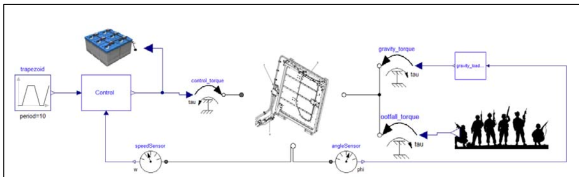
Figure 16. The Modelica Model of a Rear Ramp System
