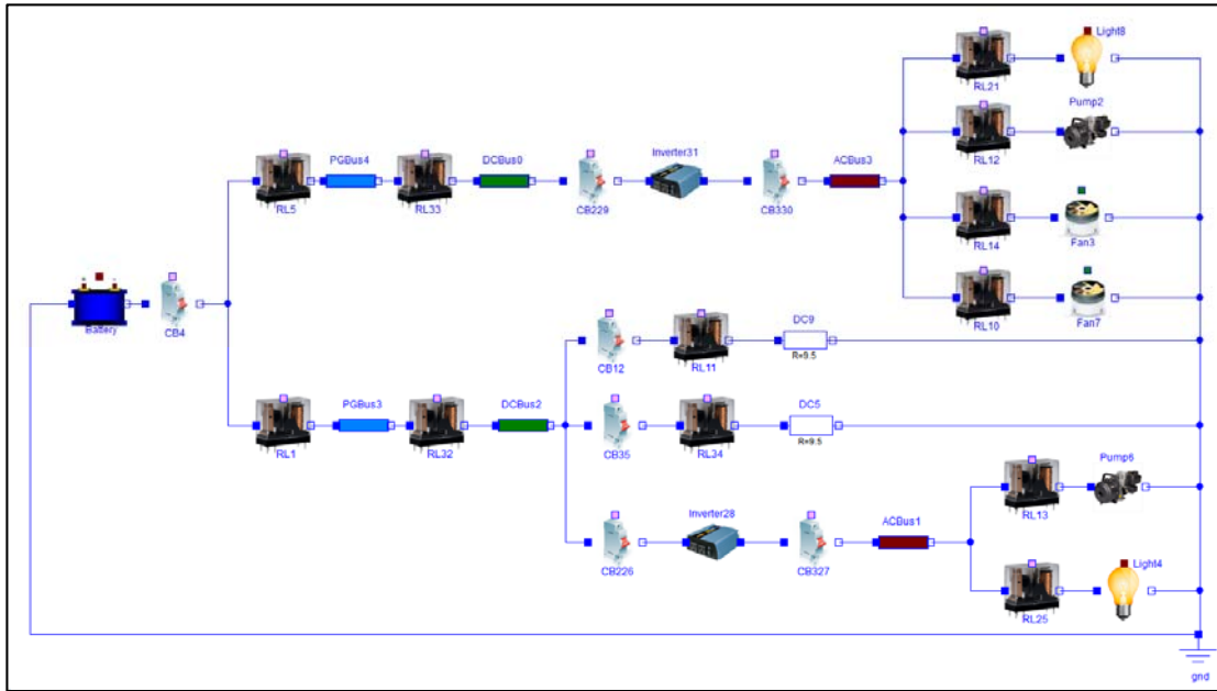
Figure 12. Automatically generated Modelica performance model with one power source and multiple loads.
