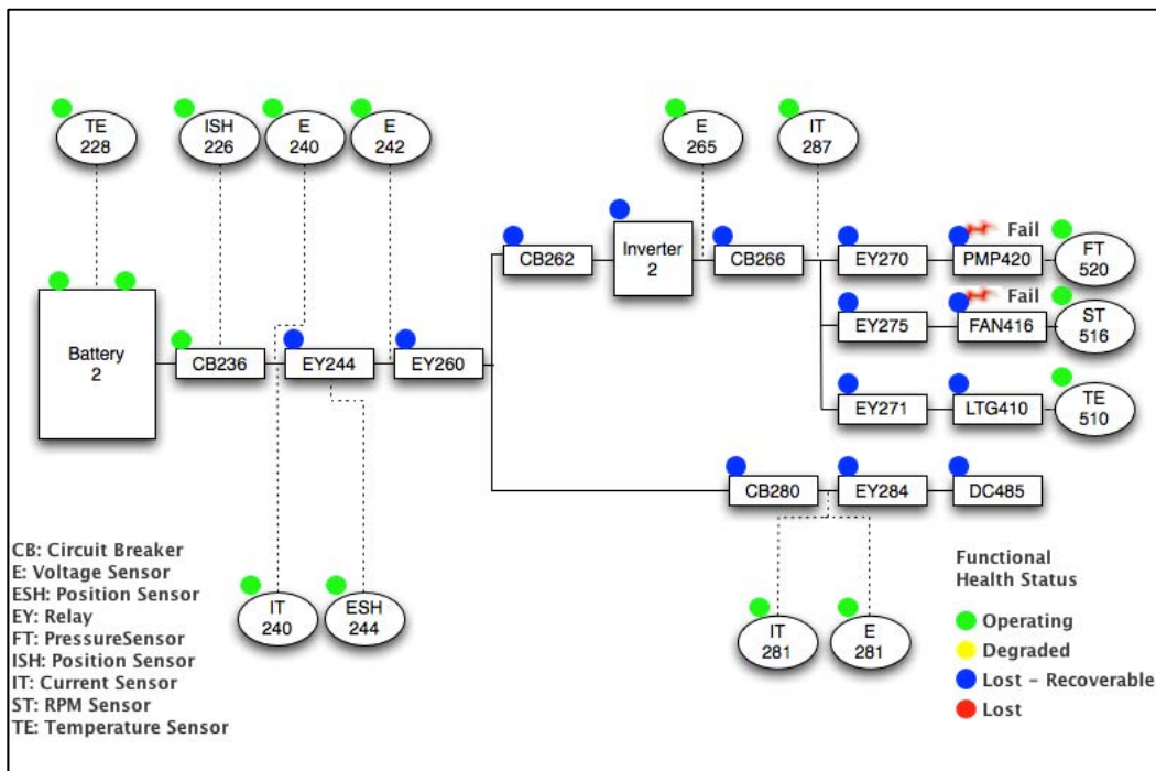
Figure 4. Results of an FFA Fault Propagation Simulation on an EPS Design
