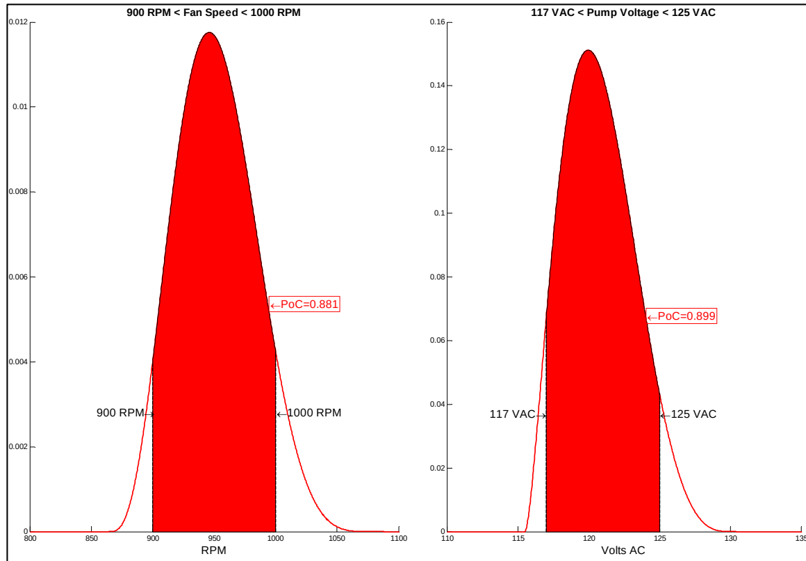
Figure 5. PoC Computation for an EPS Model with Respect to Two Different Requirements
