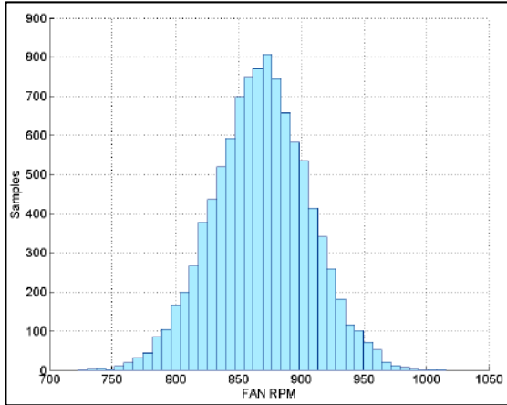
Figure 13. Phase 1 Output Distribution from MCS.
