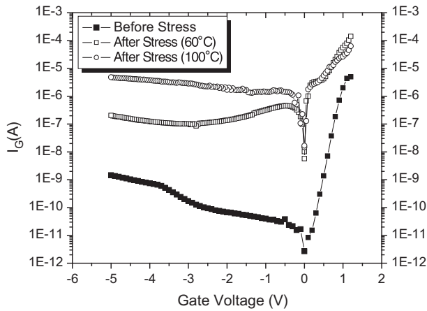
Fig. 3. Gate current of 0.17 \mu\text{m} gate length HEMT before and after on-state step stress with a base-plate temperature of 60 °C and 100 °C.
