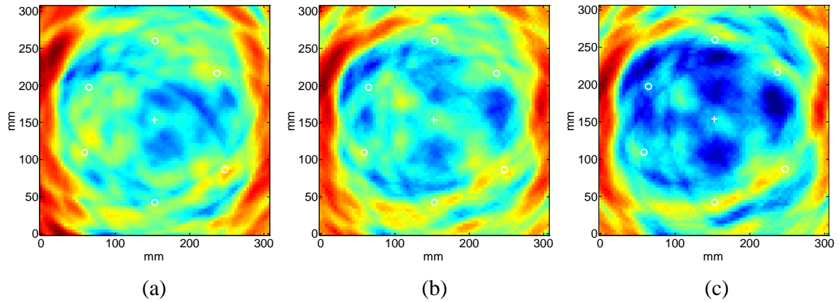
Figure 5. Images generated between data set 3 (baseline signals) and data set 7 (current signals, 5.4 mm long fatigue crack) at mismatched loads. All three images are shown on a 10 dB color scale normalized to their maximum amplitudes. (a) 23/0 MPa (20/0% load), max amplitude of -57 dB, (b) 69/0 MPa (60/0% load), max amplitude of -55 dB, and (c) 115/0 MPa (100/0% load), max amplitude of -51 dB.
