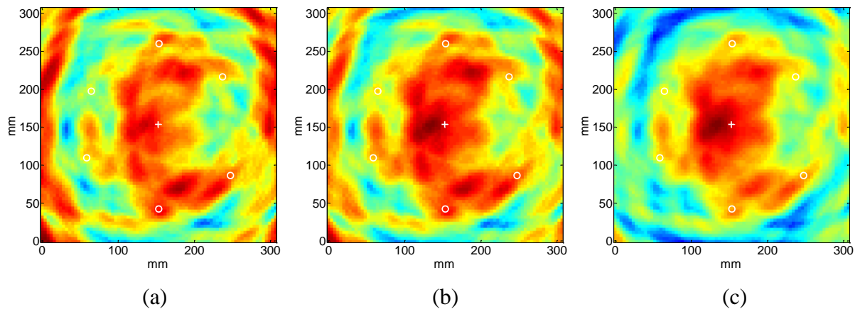
Figure 6. Images generated between data set 3 (baseline signals) and data set 7 (current signals, 5.4 mm long fatigue crack) at mismatched loads. All three images are shown on a 10 dB color scale normalized to their maximum amplitudes. (a) 0/115 MPa (0/100% load), max amplitude of -48 dB, (b) 46/115 MPa (40/100% load), max amplitude of -49 dB, and (c) 92/115 MPa (80/100% load), max amplitude of -49 dB.
