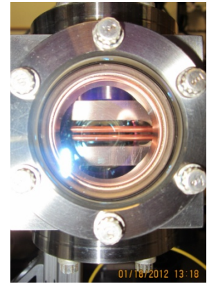
Figure 2c: View into the condensation region. The window has sufficient space for imaging and tunneling-barrier lasers.
