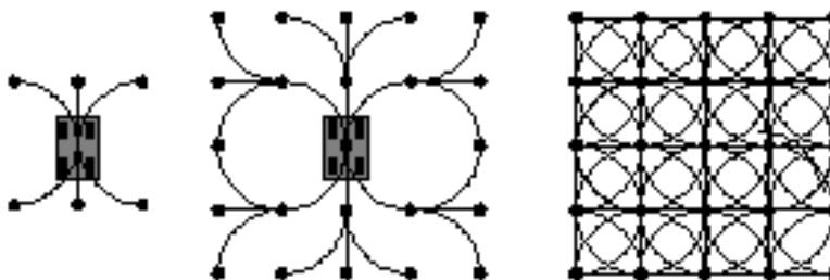
Figure 3.2.1: State lattice for Reeds-Shepp car. The Reeds-Shepp car can move forward and backward and it can drive straight or turn left or right at a fixed curvature. The presented rudimentary control set is derived from these basic controls by choosing their length such that only four heading values are used. Left: The designed control set precisely hits vertices in a rectangular grid. Center: The reachability tree to depth 2. Right: The reachability tree obtained by copying the control set at every vertex in a C space with 4 headings. Each dot represents 4 distinct vertices overlaid over each other, each representing different values of heading. While this search space will not generate a turn exceeding the chosen curvature, and while heading is continuous across vertices, the instantaneous transitions among curvatures at the vertices do not respect steering rate limitations.
