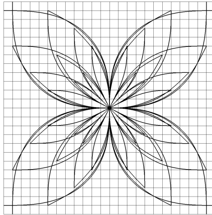
Figure 8.1.1: Experiment control sets. The state lattice control set selected for testing has 16 discrete headings, a maximum curvature of 1/8 of cell, and an average outdegree of 12, for a total of 192 curves. The straight edges cannot be seen because they are obscured by the longer curved edges.
