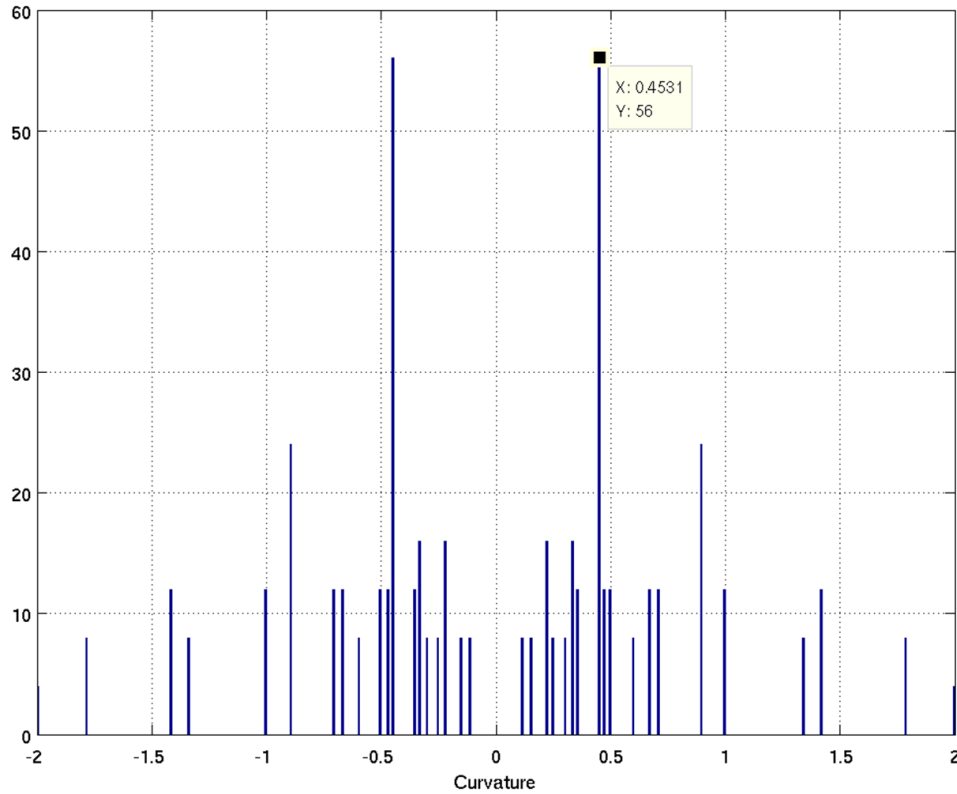
Figure 6.3.3: Arc curvature histogram. In determining steering angle discretization for the car-like system example, a constant-curvature arc is computed for each (x, y, \theta) -point in a region around the vehicle. The curvatures of the resulting arcs are plotted in this histogram. The expected symmetry is apparent. Similar to Figure 6.3.2, the values of steering angle discretization are chosen from the peaks of the histogram, in descending order.
