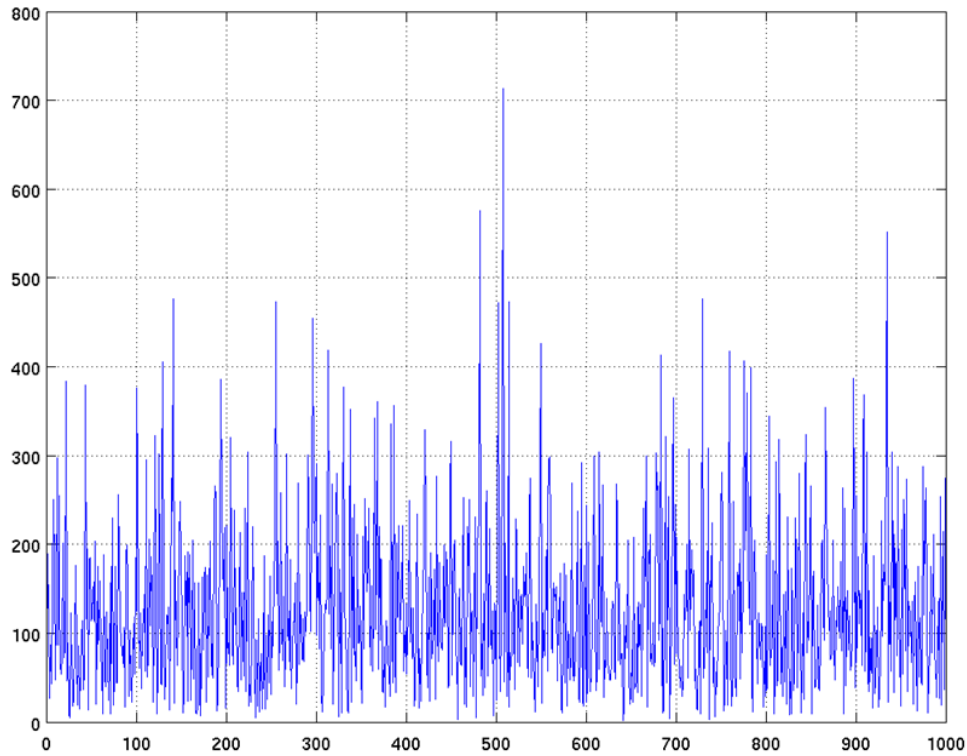
Figure 4.1.4: HLUT vs. Euclidean Comparison. This figure plots the (seconds) runtime ratios, of executing a set of motion planning queries with a car-like robot model with two A* planners, where the only difference was the choice of the heuristic: HLUT and Euclidean distance. The plot demonstrates that utilizing an HLUT leads to over 100x speed-up in planning runtime.
