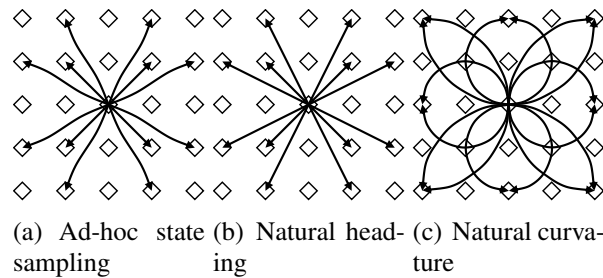
Figure 6.3.1: Motivating natural sampling rule. Part a): ad-hoc state sampling may result in overly complex controls. Straight lines b) and arcs c) are natural for a car-like system because they do not require actuation of the steering angle.
