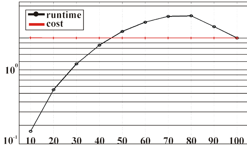
Figure 8.2.2: Simulated robot traversal: limited perception. The results of the simulated robot traversal using graduated fidelity as in Figure 8.2.1, but with the a limited perception horizon. Averages over 10 independent trials are presented.
