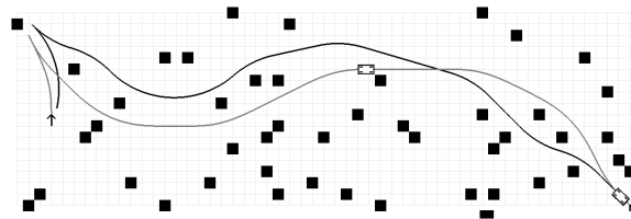
Figure 8.1.2: World with Obstacles. A portion of the world with point obstacles used in the experiments is shown here. Two plans are shown which solve the same query. The black line shows the plan generated by the state lattice, while the grey line traces the path returned from the BL planner.
