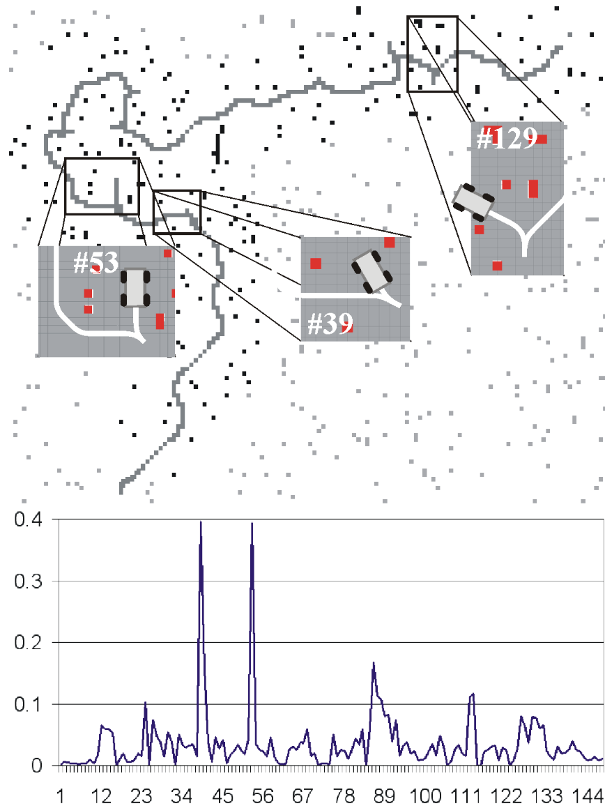
Figure 8.3.1: Long-distance simulated forest traversal. A simulated experiment of traversing about 500 meters among previously unknown obstacles. Top: the first 40 meters of the path are shown for clarity. Note that all motions generated by the planner were globally feasible, and backing up maneuvers were generated automatically when necessary. Bottom: plot of planner runtime (vertical axis is runtime in seconds, and the horizontal axis is replan cycle number).
