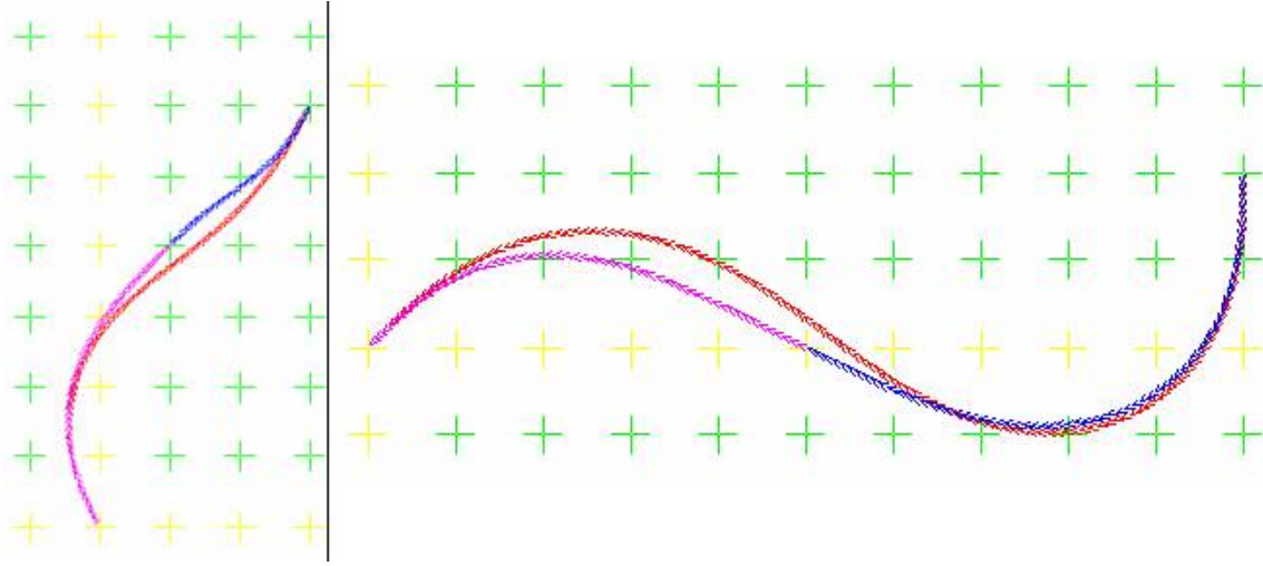
Figure 7.3.3: Motion decomposition examples. The original path is red, the two eliminating sub-paths are magenta and blue. In either case, two sub-paths happened to exist in the control set so that a). they could be concatenated to produce a path with the same initial and final pose as the original, and b). the produced path was not spatially distinct from the original.
