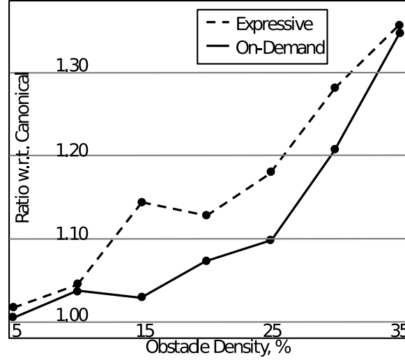
Figure 8.5.4: Relative coverage. A plot of the number of attainable states using Planners 2 and 3, represented as the ratios to the corresponding quantities of Planner 1. The plot demonstrates that on-demand expansion (solid line) features a similar improvement over the canonical motion set as the expressive motion set, while allowing significantly lower computation cost, as suggested in Figure 2a).
