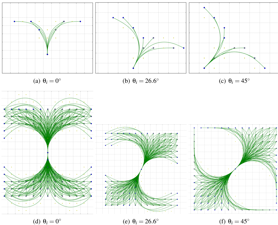
Figure 8.5.2: Canonical and expressive control sets. Top row: a set of canonical motion primitives that represents the minimal expressiveness, yet yields fast planning due to its small size. Bottom row: the other end of the spectrum: high expressiveness, yet longer planning runtime.
