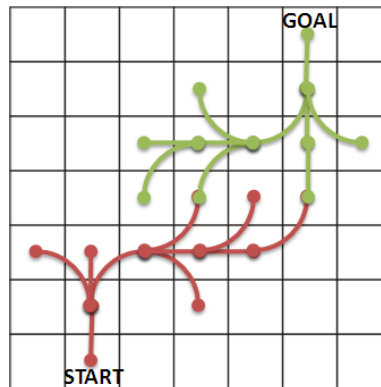
Figure 4.5.1: State Lattice Bi-RRT . The problem of gaps at the connections of the leaves of the two trees is eliminated with lattice primitives due to the regularity of endpoints in state space.
