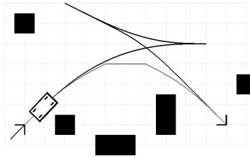
Figure 8.1.11: Control sets with and without turn-in-place. In black, a control set with a minimum turning radius of 8 cells is used. In grey, the same control set is augmented by two additional controls which allow the vehicle to turn in place at a cost equal to traversing 5 cells. This plan performs the turn-in-place maneuver twice in order to execute a sharp turn.
