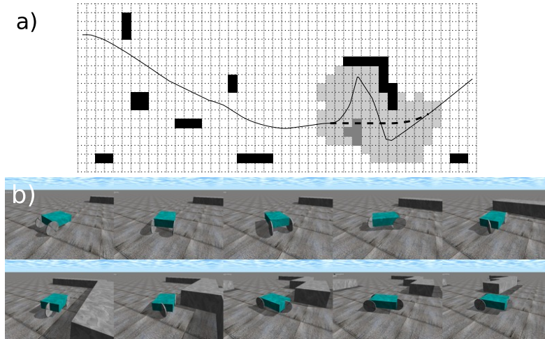
Figure 8.4.3: Kinodynamic incremental planning. Robot is avoiding a number of obstacles (black cells), while traveling at high speed on slippery surface. A new obstacle (dark gray cells) is discovered and invalidates a segment of the previous trajectory (dotted line). D^* repairs the path by expanding states (light gray) only in the affected region.
