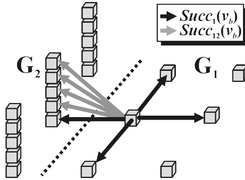
Figure 4.4.2: Spanning dimension boundary. The 2D subgraph G_1 (4-connected grid) is connected to another subgraph G_2 of a higher dimension. Black arrows are the standard node expansion (4 nearest neighbors), and gray arrows are additional edges that connect the two subgraphs.
