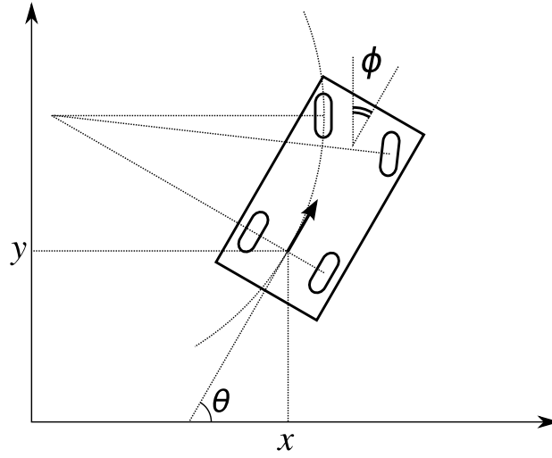
Figure 1.2.1: Car-like system model. The figure shows a simple system model that represents the kinematics of a typical four-wheeled vehicle with car-like mobility. The variables x and y are the 2D coordinates of a reference point of the vehicle with respect to a Cartesian frame, and \theta is the angle between the positive x -axis and the main axis of the vehicle; \phi is the steering angle.
