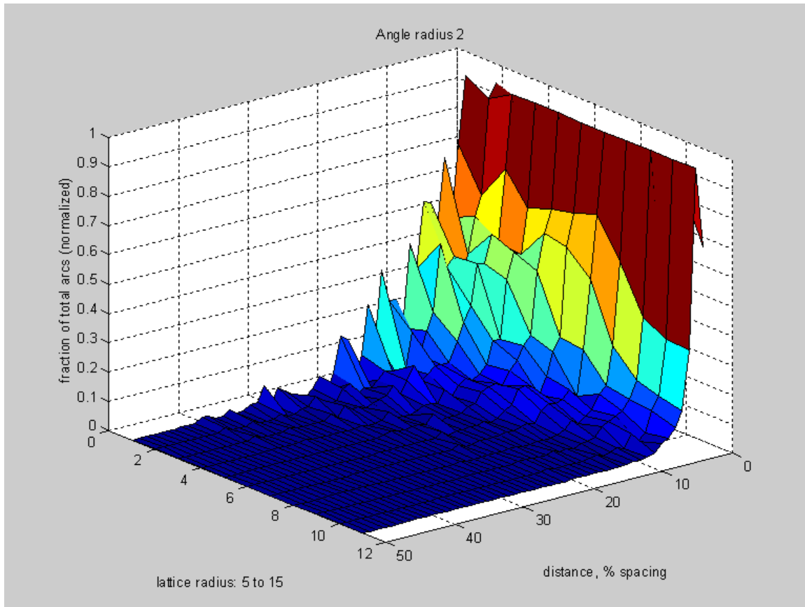
Figure 7.3.2: Node distance histogram. Summary of the minimum distance to any node study. This graph shows the percentage of the paths that have a particular value of minimum distance to any node, expressed as a percentage of 2D spacing between control set nodes, given a particular control set radius (here same as lattice radius).
