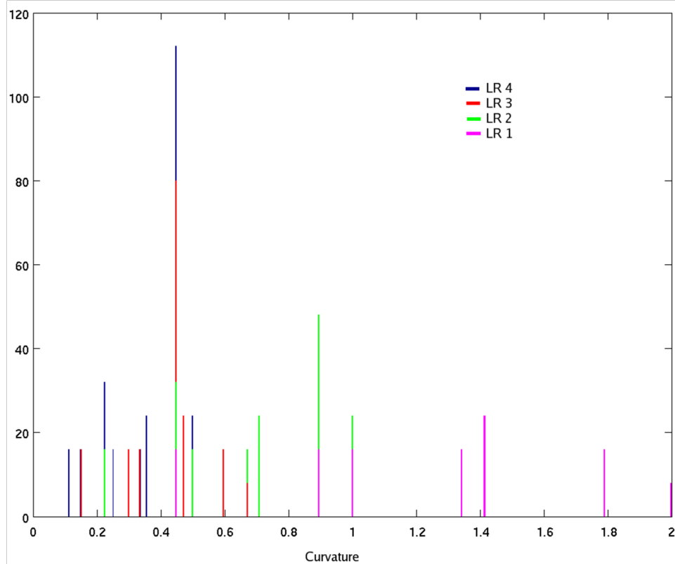
Figure 6.3.4: Distance-sorted curvatures. The histogram shows the number of constant-curvature trajectories for each curvature value. Curvature values are sparse because the study in this example only computes arcs connecting lattice nodes exactly. The vicinity of the connected nodes is represented by Lattice Radius (LR), equivalent to L_1 -norm in 2D. Note that arcs from origin to 8 immediate neighbor nodes (magenta bars) provide all curvature values above 50% of max. curvature.
