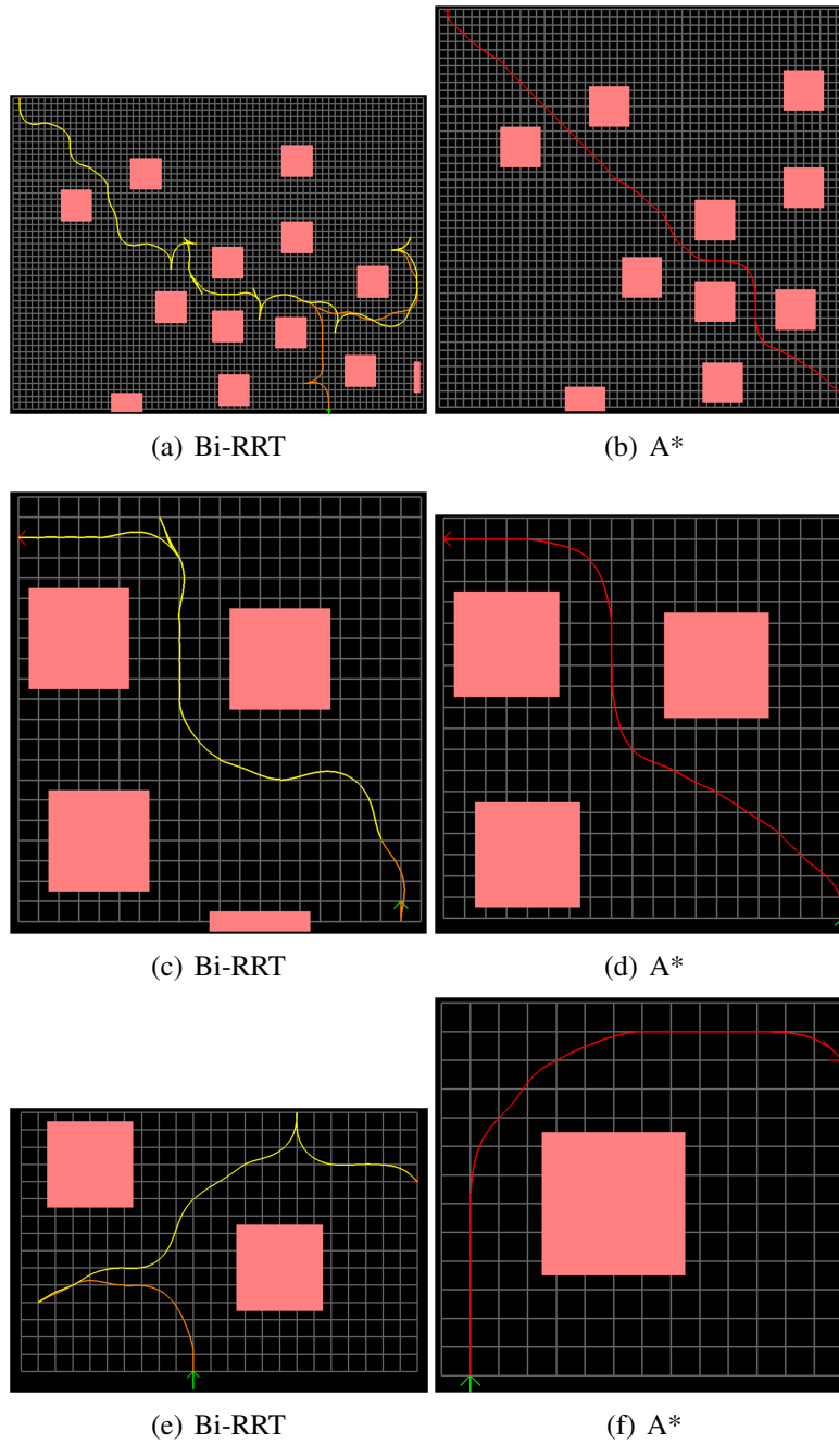
Figure 4.5.2: Bi-RRT results. Motion plans computed with Bi-RRT search (left) and A* (right). The performance results are presented in Table 4.2.
