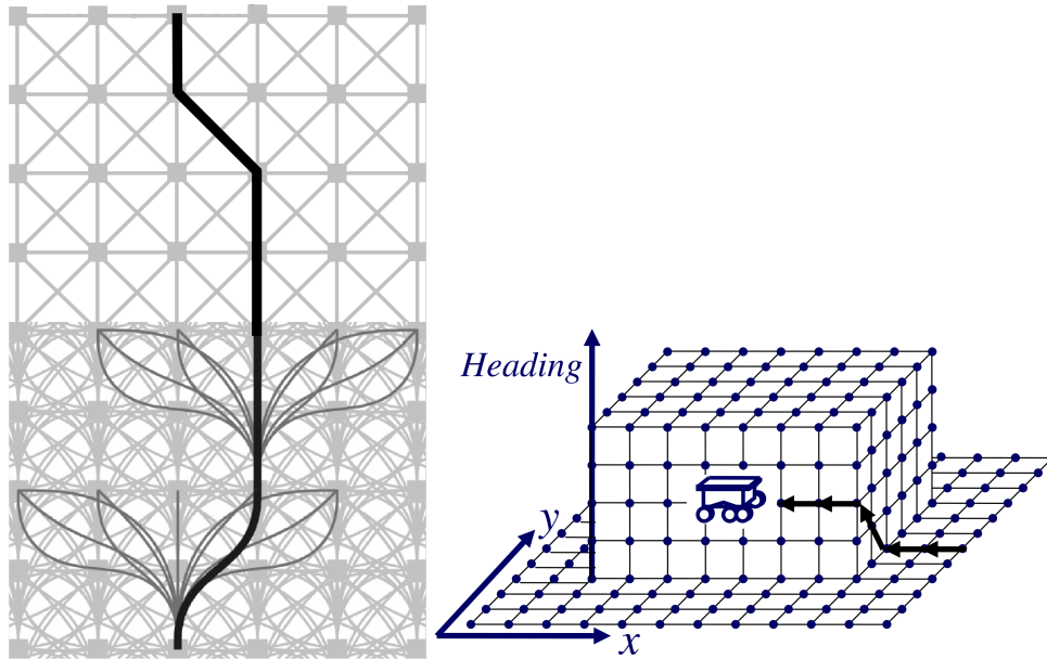
Figure 4.4.3: Graduated fidelity example. A simplified representation of two state lattices of different fidelities, seamlessly merged due to structure: a three-dimensional roadmap that includes position (x, y) variables and heading is allocated in the vicinity of the vehicle, and a lower-dimensional one, with just position variables, is further away.
