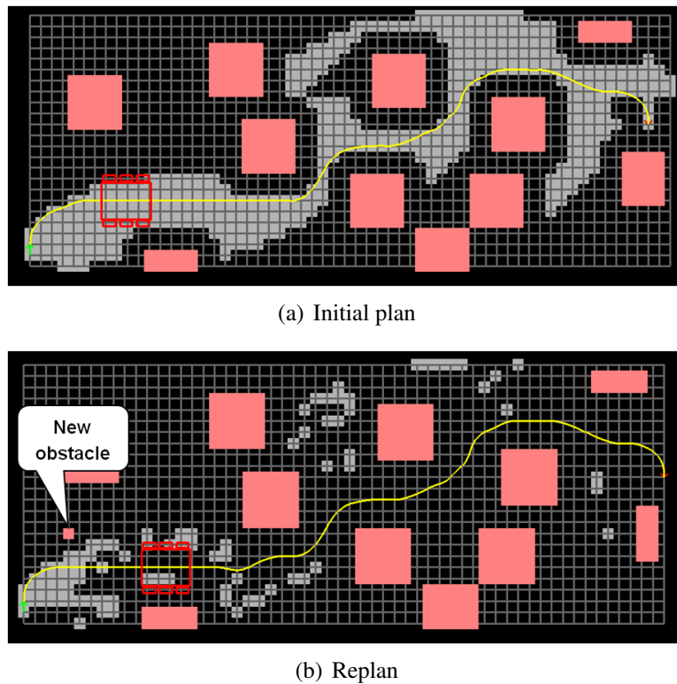
Figure 4.2.2: Nonholonomic D* . A simple 2D example of incremental planning with D*. An initial plan (a) and an incremental replan (b) to “fix” the initial plan that was blocked by a point obstacle (new point obstacle in figure placed in collision with red vehicle frame). Grey cells are expanded vertices.
