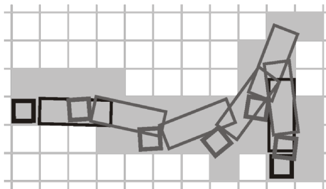
Figure 4.1.1: Trajectory swath. One of the motion primitives from a state lattice developed for a tractor-trailer robot is shown. It is a maneuver that re-oriens the robot by 90^\circ in heading. The trajectory swath was computed using Runge-Kutta simulation and cached off-line. During on-line planning, the evaluation of the cost of this maneuver with respect to a cost map is reduced to a summation operation over a memory array, resulting in approximately 100x speed-up.
