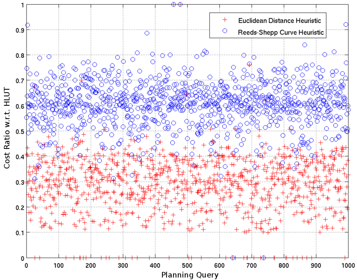
Figure 4.1.3: Heuristic comparison. Euclidean and Reeds-Shepp distance metrics are compared with the HLUT, in the context of a car-like system. The units of each of the three metrics were maintained to be the same. Reeds-Shepp and Euclidean distances are fairly significant underestimates of the true path of the car-like robot. This observation motivates an inquiry into better-informed heuristics for this type of motion planning.
