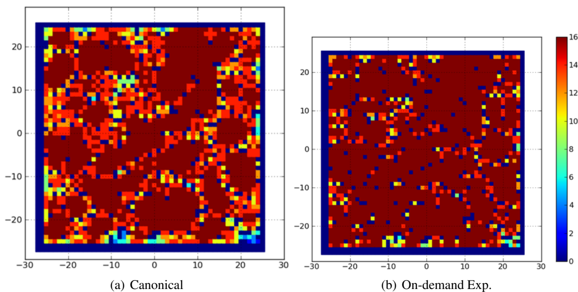
Figure 8.5.3: Coverage pseudo-color. The figure illustrates the capacity of the robot to move to locations that are hard to achieve due to dense obstacles. The pseudo-color represents the number of different headings that are attainable for each cell in the environment using the canonical template (left) and on-demand expansion (right). Shades of red denote the number of attainable headings (deep red represents all desired headings), while blue cells are obstacles.
