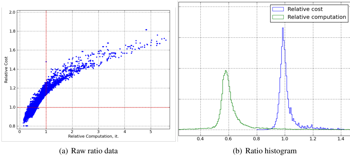
Figure 5.2.1: Empirical ratio metrics. The figure compares two different state lattice search spaces and indicates that, on average, one of the search spaces was as much as 40% more efficient at computing approximately the same quality of solutions (cost ratio peaks at 1.0).
