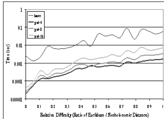
Figure 8.1.6: Lattice vs. Grid with 5% Obstacle Density. Queries of length 40 cells are shown. The grid outperforms the lattice, but it usually returns infeasible solutions in a dense obstacle field. Lattice planner runtime is still acceptably fast.
