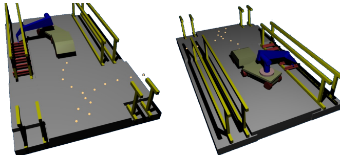
Figure 8.6.5: A pick-and-place experiment. The robot’s task is to install red I-beams between long yellow beams at a construction site. A 5-DOF, PUMA-class arm with a 1-DOF gripper is installed on the trailer of a mobile robot with tractor-trailer mobility. The system must operate in narrow passages among obstacles. The figure shows the base placement of the robot computed by the planner, given the desired pose for placing the I-beam object. Orange dots show the base planner solution, the trajectory of the tractor robot. Left and right subfigures show different viewpoints of the scene.
