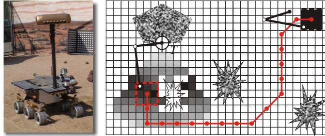
Figure 8.6.2: 2D point-at task. Left subfigure shows the Rocky8 rover that inspired this and the following subsection (courtesy of JPL [103]). The figure on the right illustrates mobile manipulation in the scenario where the robot moves from top right of the figure (arm is stowed initially) to the pose that maximizes manipulability. Note that the base joint of the arm lands in the black cell, indicating minimal manipulation cost). The red line with dots is the motion of the base, computed by the planner. The dots are the vertices of the graph (elaborated by the planner), and the lines are the edges. The motion represents the resolution-optimal trade-off between path cost (length) and manipulation cost (manipulability) automatically made by the planner.
