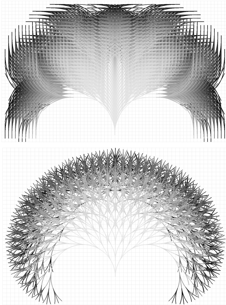
Figure 8.1.8: Reachability Trees for the Lattice and BL. At top, the first 1400 expansions of the basic state lattice control set in best-first order. At bottom, the first 1400 expansions of the BL control set were generated using the same algorithm. Lighter edges are older in both images.
