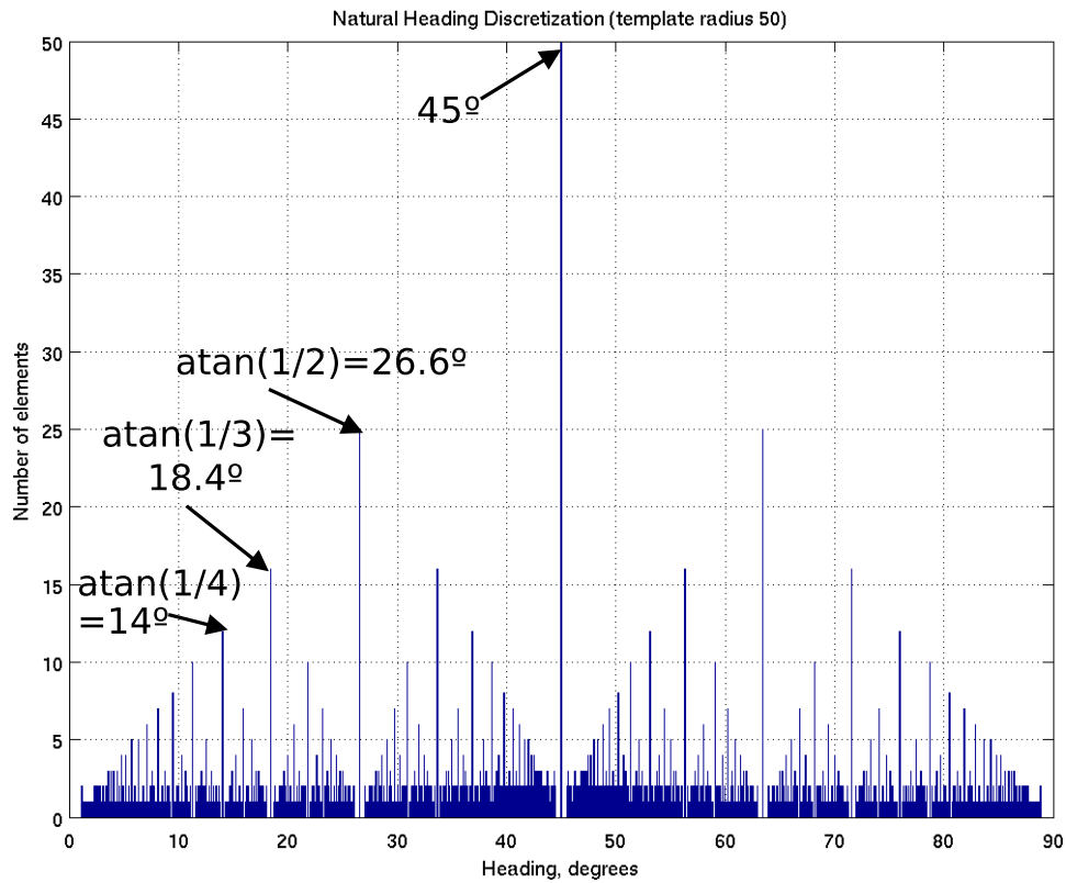
Figure 6.3.2: Natural heading discretization. The heading values that correspond to spikes in the histogram are shared by a greater number of natural motions in this example, and therefore are good candidates for inclusion in sampling the heading dimension, in the order of their frequency.
