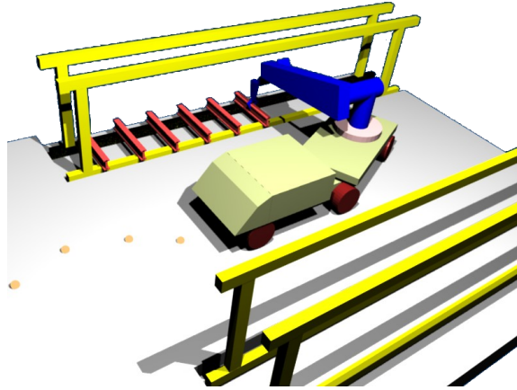
Figure 8.6.4: Placing I-beams in autonomous construction. The proposed approach is well-suited for “pick-and-place” and other common manipulation tasks. In this example, the robot’s task is to install I-beams at a construction site that is too large and constrained to allow the use of a fixed manipulator workcell. The motion, computed by the planner, represents a resolution-optimal trade-off between path length, traversed by the tractor-trailer platform, and the subsequent manipulator operation.
