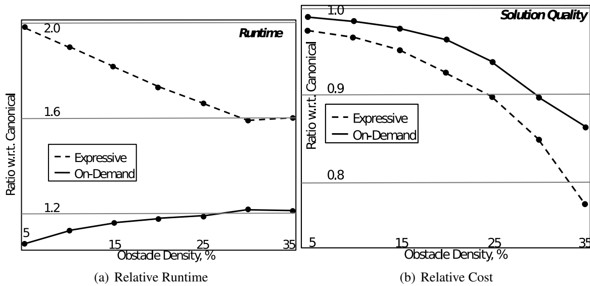
Figure 8.5.1: On-demand expansion performance. Simulation experiments evaluating the performance of canonical, expressive, and on-demand expansion control sets. Parts a) and b) compare the relative runtime and solution cost, respectively, of expressive and on-demand expansion-based motion sets with respect to canonical motion sets (with varying obstacle density). Although the expressive motion set unsurprisingly produces the safest paths, almost the same quality of motions is achieved by the on-demand expansion-based motion set while consuming significantly less computational resources.
