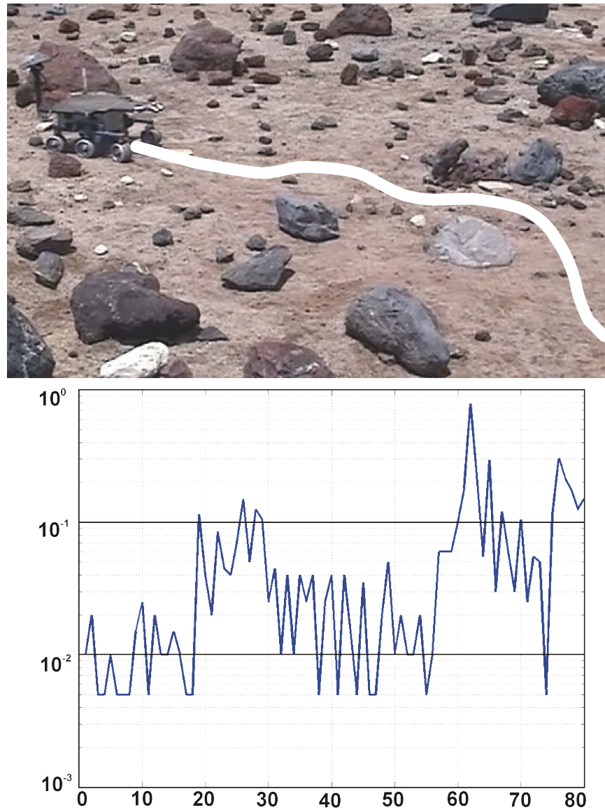
Figure 8.3.2: JPL Mars Yard experiment. FIDO rover navigated autonomously among previously unknown obstacles, while running the graduated fidelity lattice planner on-board. Top: approximate path the rover followed. Bottom: a plot of planner runtime (vertical axis is runtime in seconds, and the horizontal axis is replan cycle number).
