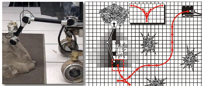
Figure 8.6.3: 3D point-at task. Left subfigure is intended to motivate this class of manipulation tasks; it shows a close-up view of the Rocky8 rover's arm performing a rock imaging study, common in planetary exploration (courtesy of JPL [103]). The figure on the right illustrates a more realistic set of experiments that extend Figure 8.6.2. The initial pose of the rover is shown in top right (with arm stowed). The inset shows the control set utilized by the state lattice nonholonomic planner [109]; an identical set of controls for reverse motion is omitted for conciseness. The red line with dots represents the solution of the planner, where the dots are the vertices of the graph, elaborated by the planner, and the lines are the edges. Similar to Figure 8.6.2, the motion represents the trade-off between path cost (length) and manipulation cost (manipulability), automatically made by the planner.
