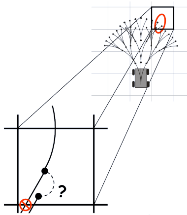
Figure 4.2.1: Motivation for graph structure. Sampling control space without regard for state space structure may not result in the cyclic graph structure that is necessary to reuse previous computation. For example, tree-based search spaces where vertices are dense in X , would not allow reusing previous computation via predecessor redirection. In case a predecessor edge becomes invalidated due to new environment information (red stop-sign in the figure), an attempt to reuse an alternative predecessor would result in a gap in the trajectory (question mark).
