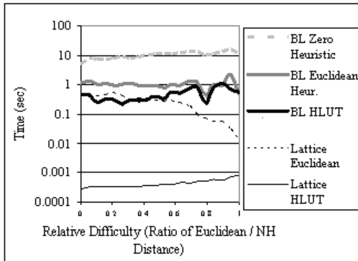
Figure 8.1.9: Lattice vs. BL without Obstacles. Queries with an absolute difficulty of 40 cells are shown. Various heuristics are considered for each planner. Only when the slow Zero heuristic is used does BL return optimal paths.
