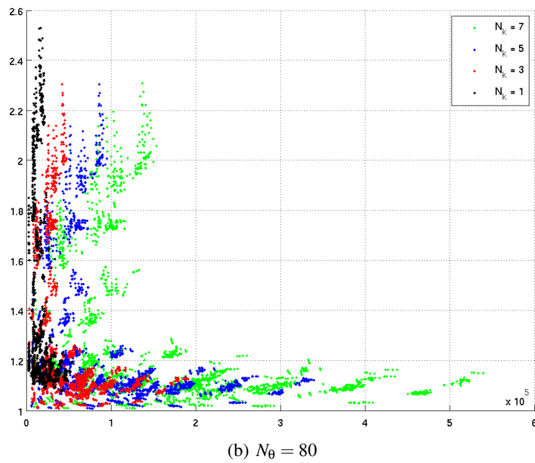
Figure 5.2.4: Resolution-space analysis (cont.). The resolution space of heading and steering angle dimensions is continued here for heading discretizations with 32 and 80 values.
