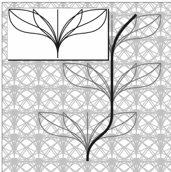
Figure 3.2.2: State lattice for general car-like system. This is one of the potential designs of a state lattice for a car-like system in Example 1.2.1. The motion primitives are regularly arranged in state space; to design them, a convenient state sampling rule is chosen (e.g. a low discrepancy lattice), and a controller is used to connect the samples via feasible motions. Given heading discretization in this particular example, such a set is to be defined for each of the 8 discrete values of initial heading, the multiples of \pi/4 ; symmetry can be exploited to define only two such sets, corresponding to the initial heading in the interval [0, \pi/2) .
