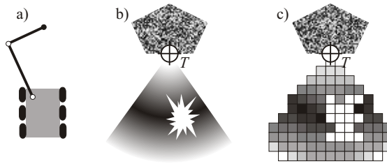
Figure 8.6.1: Discretized goal region. Figure a) shows a two-link planar arm installed on a mobile base. Figure b) illustrates a subset of the goal region G induced by \rho(\bullet) , where grayscale intensity corresponds to its value (white color indicates \rho(\bullet) = \infty ). An odd-shaped obstacle is visible near the manipulation target T . Figure c) shows the discretized version of the goal region, G_d . The obstacle causes a set of cells to be white – infeasible poses for the base joint of the arm.
