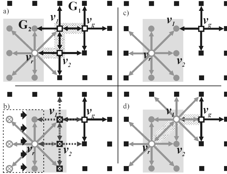
Figure 4.4.1: Dynamic search space. Maintaining the connectivity between two subgraphs of different fidelities of representation. G_1 is a static subgraph (black square vertices), and G_2 (gray circular vertices) moves w.r.t. the former. Arrows are edges. Hollow vertices have been expanded. Subfigure a) shows the initial plan (thick patterned line), as it originates in G_1 and proceeds into G_2 ; b) as G_2 moves from left to right, the six crossed out vertices change subgraph ownership, and convert_vertex is executed on each of them, which results in undoing the previous expansions of v_1 and v_2 ; c) shows the completion of moving G_2 : the vertices v_1 and v_2 now belong to G_2 and are available for re-expansion, if necessary, when the search algorithm performs replanning; lastly, d) shows the result of replanning in the search space from c), where due to re-expansion of v_1 under G_2 edge connectivity, a new plan is found.
