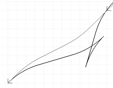
Figure 8.1.9: Lattice vs. BL without Obstacles. Queries with an absolute difficulty of 40 cells are shown. Various heuristics are considered for each planner. Only when the slow Zero heuristic is used does BL return optimal paths.
