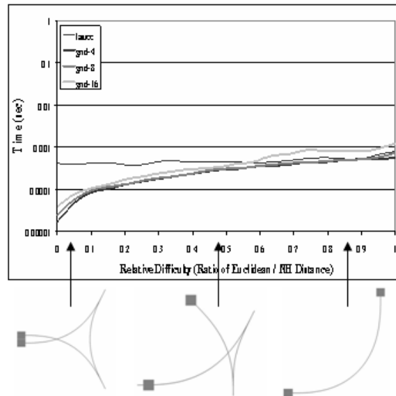
Figure 8.1.5: Lattice vs. Grid without Obstacles. Queries with an absolute difficulty of 40 cells are shown. The lattice performs similarly to the grid planners overall. Only for the greatest relative difficulty (nearest zero) does the lattice require more CPU cycles. Of course, the benefit of this extra computation is a plan which is feasible.
