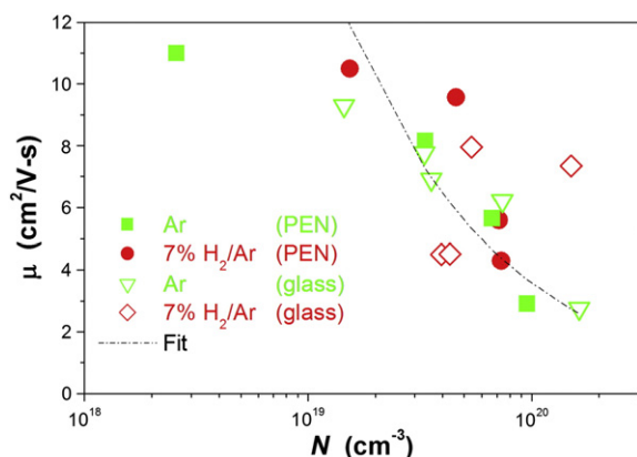
Fig. 13. Mobility variation as a function of carrier concentration on films deposited on glass and PEN substrates. Dashed line indicates the theoretical fit from Conwell, Weisskopf and Shockley equation with Z=2 .
