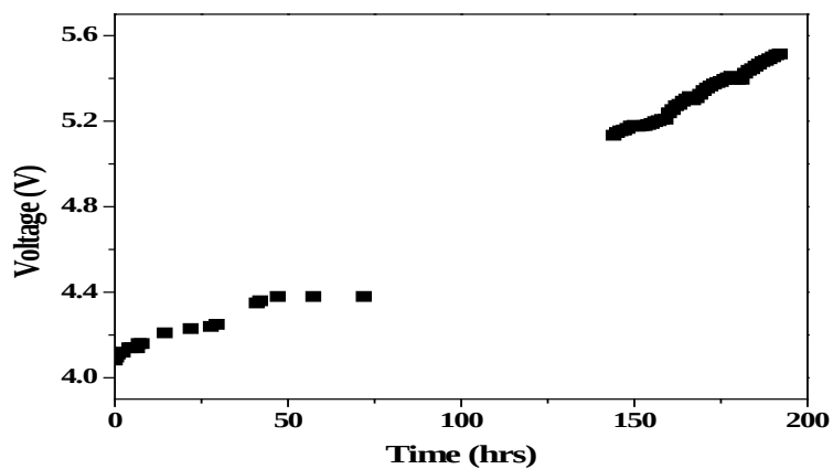
Figure Y5.10. Plot of voltage vs. time for the OLED.
