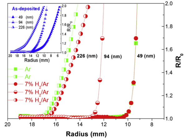
Fig. 11. Collapsing bend test results for as-deposited, Ar annealed and 7% H 2 /Ar annealed films.
