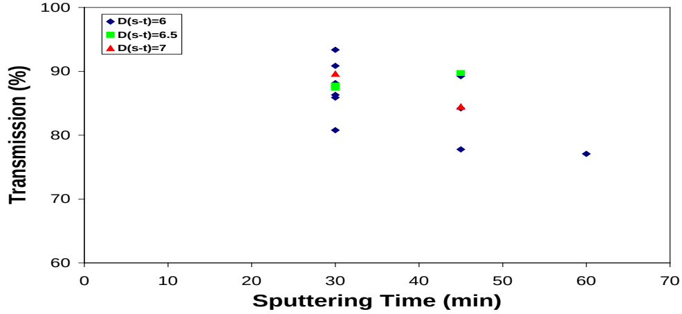
Figure Y3.2. Transmission of the layers as a function of sputtering duration for different source to target distances ( D(s-t) ).
