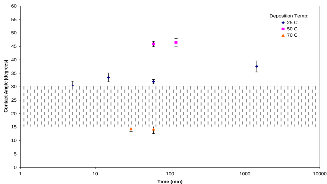
Figure 2-6. Pentafluorophenyltriethoxysilane (PFPTO) contact angle as a function of immersion time at temperatures of (◆) 25^\circ\text{C} , (■) 50^\circ\text{C} , and (▲) 70^\circ\text{C} .
