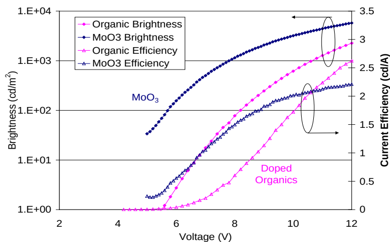
Figure 2-22. Comparison of B-V and \eta -V curves for MoO 3 buffer layers vs. doped organic (m-MTDATA:F4TCNQ) buffer layers.
