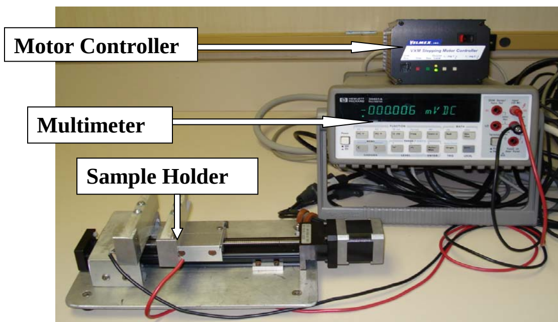
Figure Y3.5. Bend test system set up
