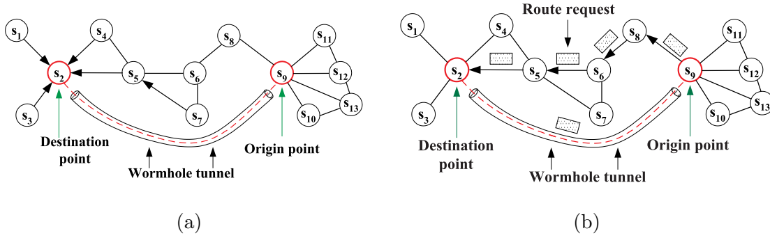
Figure 2.1: (a) Wormhole attack on a distance vector-based routing protocol. (b) Wormhole attack against an on-demand routing protocol.
