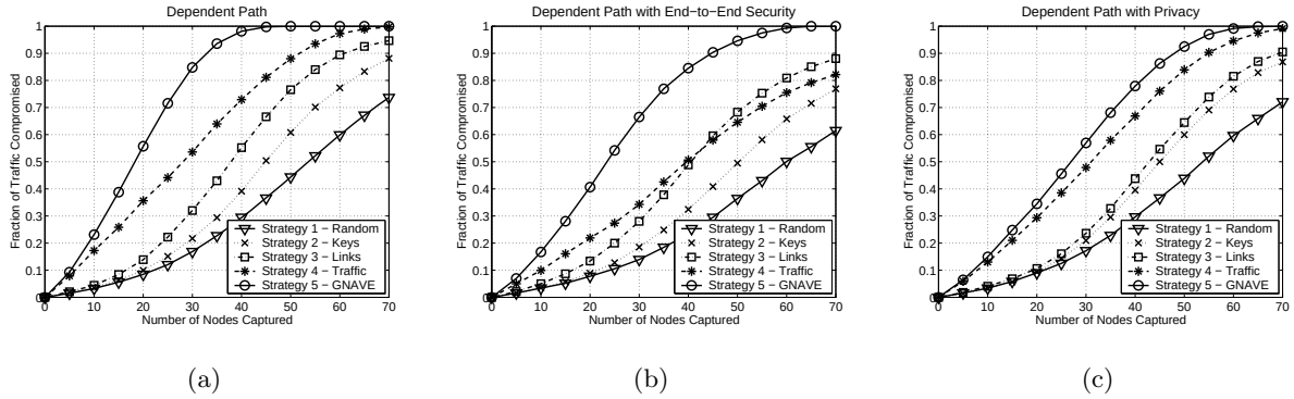
Figure 5.6: Node capture attacks using the five strategies are illustrated for a wireless sensor network of |\mathcal{N}| = 500 nodes for dependent path routing (a) without end-to-end security, (b) with end-to-end security, and (c) using a privacy-preserving set intersection protocol.
