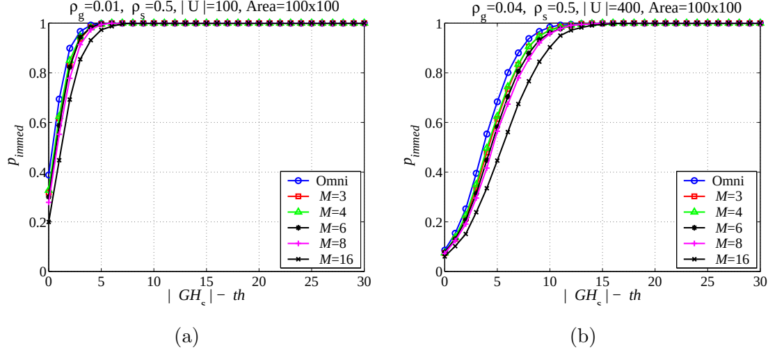
Figure 2.12: Percentage of immediate neighbors that share more than th fractional keys for r_s = 0.5 nodes/ m^2 , A = 10,000m^2 when, (a) different antennas are used at the guards and r_g = 0.01 guards/ m^2 , (b) different antennas are used at the guards and r_g = 0.04 guards/ m^2 .
