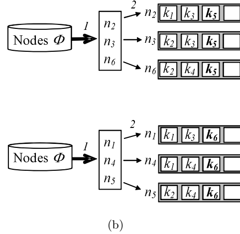
Figure 4.7: The NSNR key assignment algorithm is illustrated (a) in pseudo-code and (b) graphically with numbered steps: 1 - select subset of nodes, 2 - assign key to nodes.
