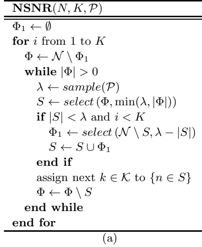
Figure 4.7: The NSNR key assignment algorithm is illustrated (a) in pseudo-code and (b) graphically with numbered steps: 1 - select subset of nodes, 2 - assign key to nodes.
