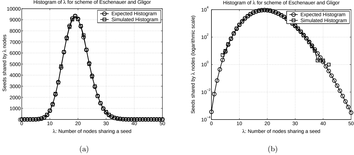
Figure 4.1: The expected histogram \mathcal{H}(\lambda) , representing the number of keys shared by exactly \lambda nodes, is illustrated for Example 1 with vertical axis in (a) linear scale and (b) logarithmic scale.
