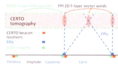
Figure 2. Tomographic and common-volume measurements envisioned for SpreadFEx-2.
