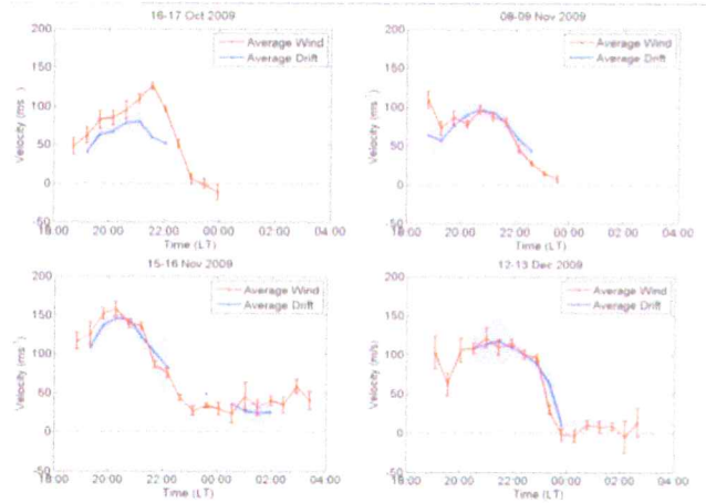
Figure 6. SpreadFEx-2 common-volume zonal winds (red) and EPB zonal drift velocity (blue) for 16-17 Oct., 8-9 Nov., 15-16 Nov., and 12-13 Dec. 2009. Note the variations at \sim 30 -min to 2-hr periods indicative of GWs superposed on the tidal motions.
