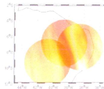
Figure 3. Overlapping imager FOVs in the 6300 Å emission showing EPBs.
