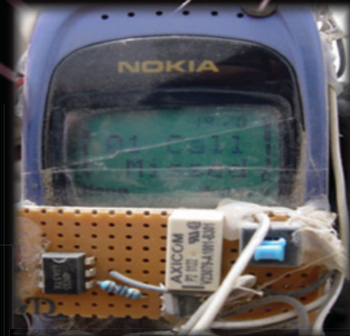
This cell phone was rigged as a detonator for an improvised explosive device. The detonator was recovered undamaged after having been successfully jammed by electronic warfare personnel using Counter Radio-Controlled IED Electronic Warfare equipment funded by the Joint Improvised Explosive Device Defeat Organization. (Photo courtesy of the Department of Defense)
