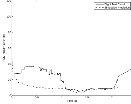
(a) Root Sum Square Error in Surrogate Missile Position Estimate
