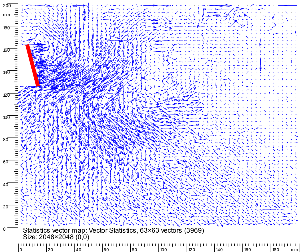
Figure 55. Quiver Plot of Phase 8 ( \psi = 235^\circ , \alpha = -10^\circ ); Water at Re = 54,400 with Prescribed Rotation Angles; 100% Span
