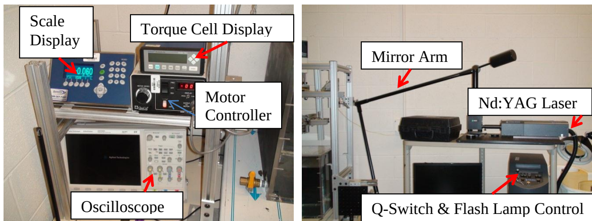
Figure 30. Test Equipment
