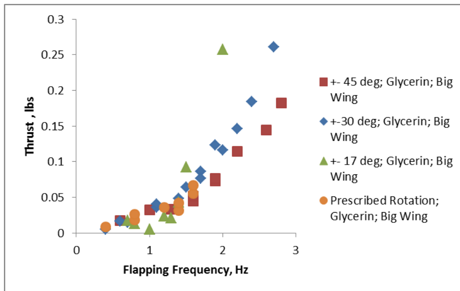
Figure 38. Thrust vs. Flapping Frequency in Glycerin with the Big Wing; Re = 44 to 188
