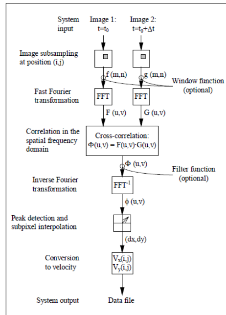
Figure 31. Numerical Processing Flowchart of PIV [Dantec Manual, 2002]
