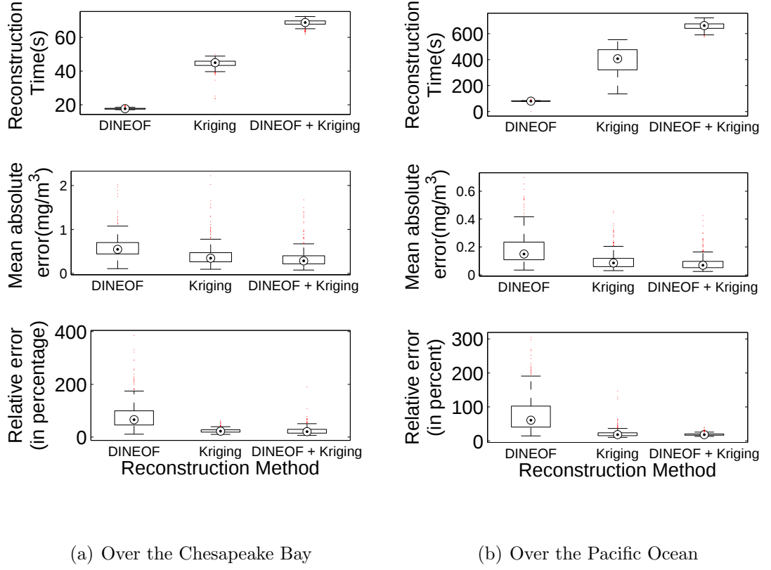
Figure 3.8: Reconstruction performances
