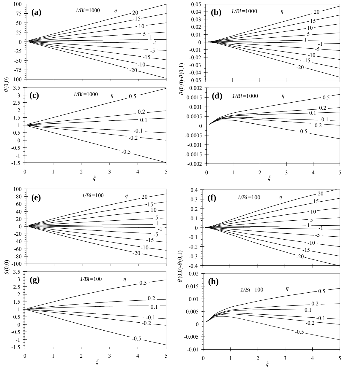
Figure 27. Top surface dimensionless centerline temperature, \theta(0,0) , and temperature variation, \theta(0,0) - \theta(0,1) , plotted against aspect ratio, \zeta , for varying dimensionless heat input, \eta ; (a), (b), (c), (d) 1/Bi = 1000 and (e), (f), (g), (h) 1/Bi = 100 .
