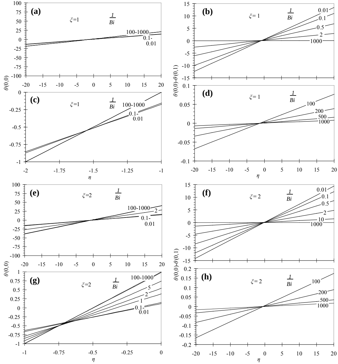
Figure 7. Top surface dimensionless centerline temperature, \theta(0,0) , and temperature variation, \theta(0,0) - \theta(0,1) , plotted against dimensionless heat input, \eta , for varying 1/Bi ; (a), (b), (c), (d) \zeta = 1 and (e), (f), (g), (h) \zeta = 2 .
