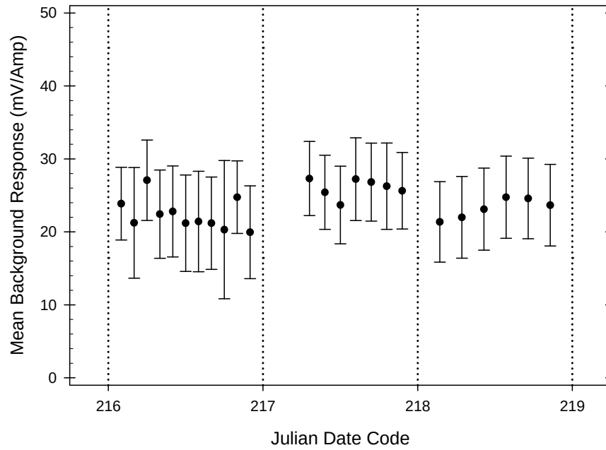
Figure 5-8 – Intra- and inter- daily variations in the response of the TEMENTADS MP 2x2 array to background anomaly-free areas at a time gate of 42 \mu s for the Remington Woods, CT demonstration.
